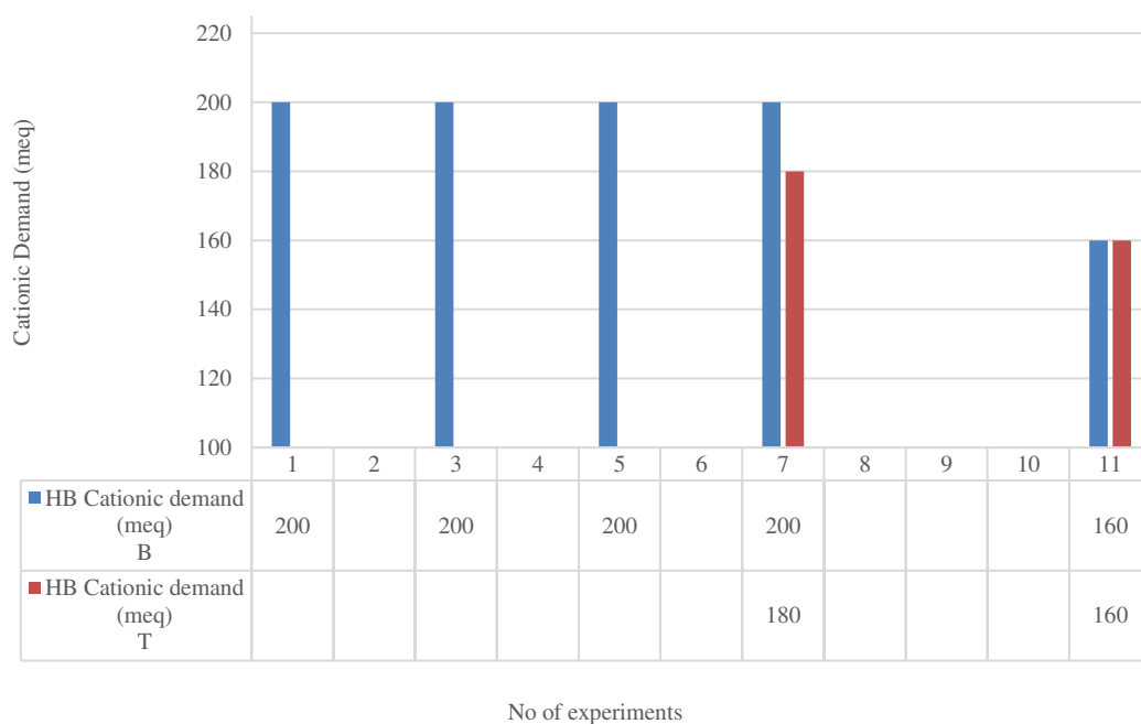
Figure 4.11 : Cationic demand values of top & bottom formers
