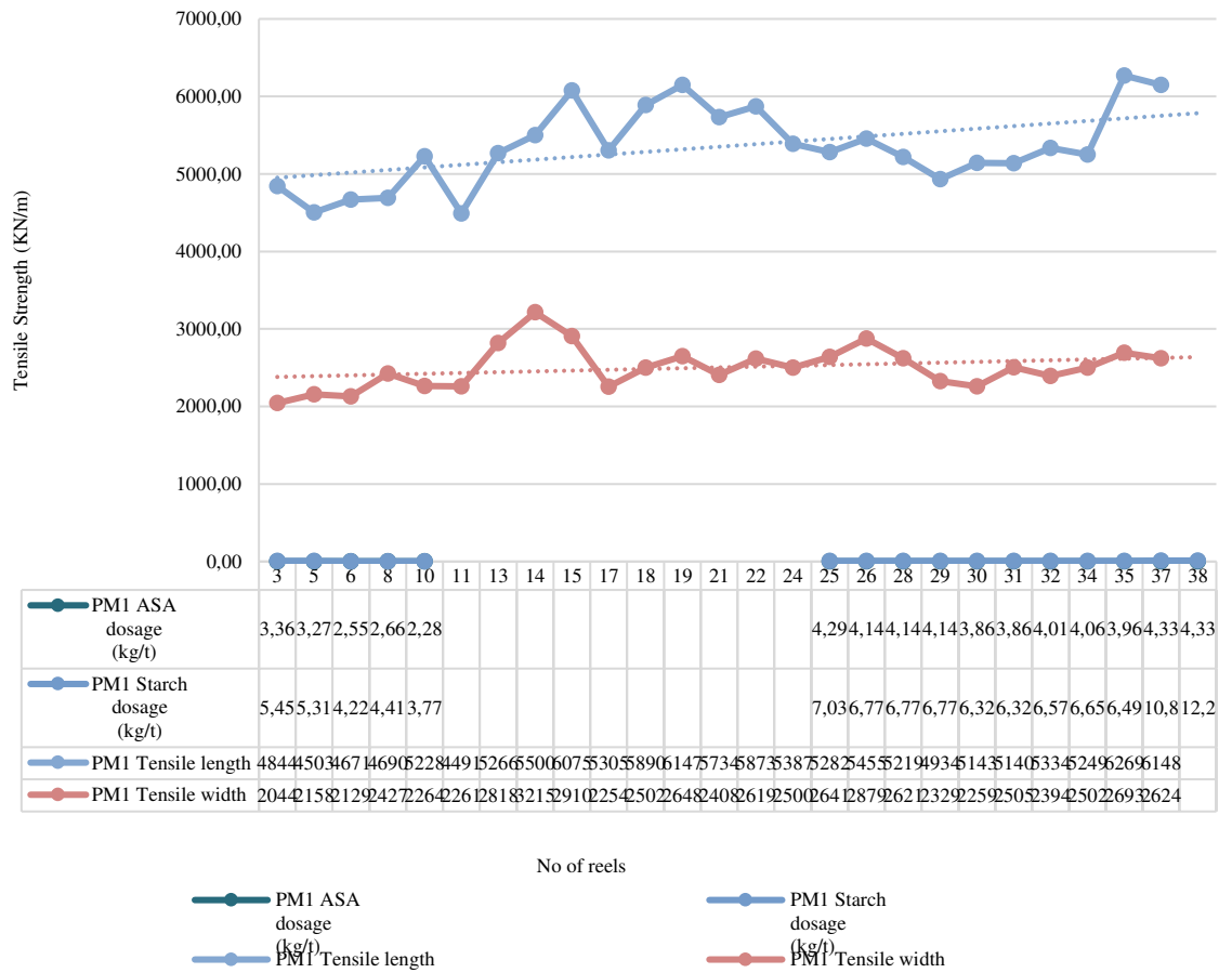
Figure 4.21 : ASA & emulsifiers dosage (kg/t) vs. tensile strength values of length & width of (kN/m)
