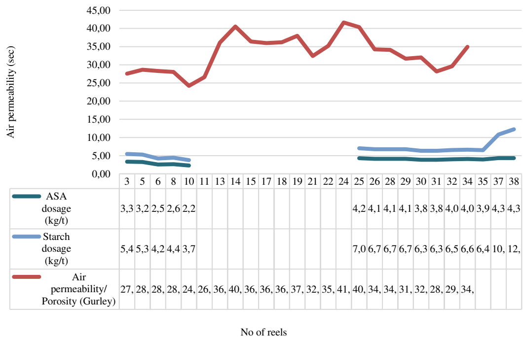
Figure 4.22 : ASA & emulsifiers dosage (kg/t) vs. air permeability values (second)
