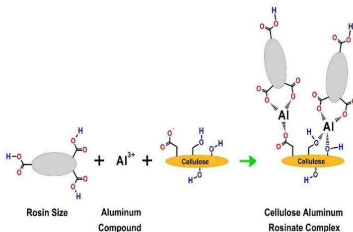
Figure 2.1 : Rosin sizing mechanism [5]
