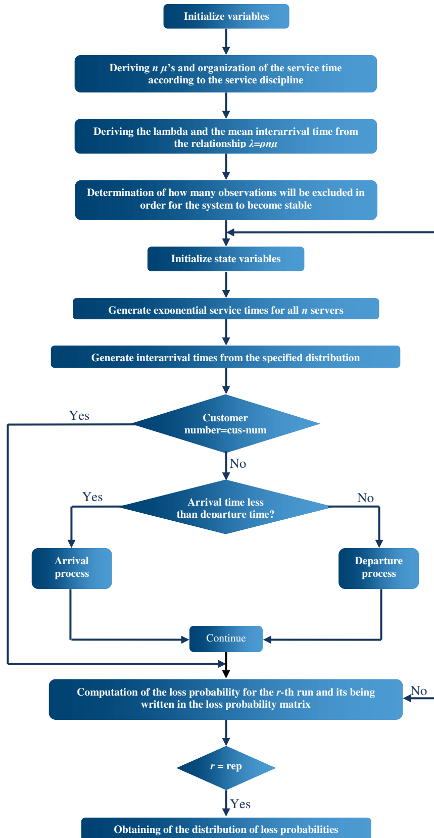
Figure 4.1 Simulation algorithm.
