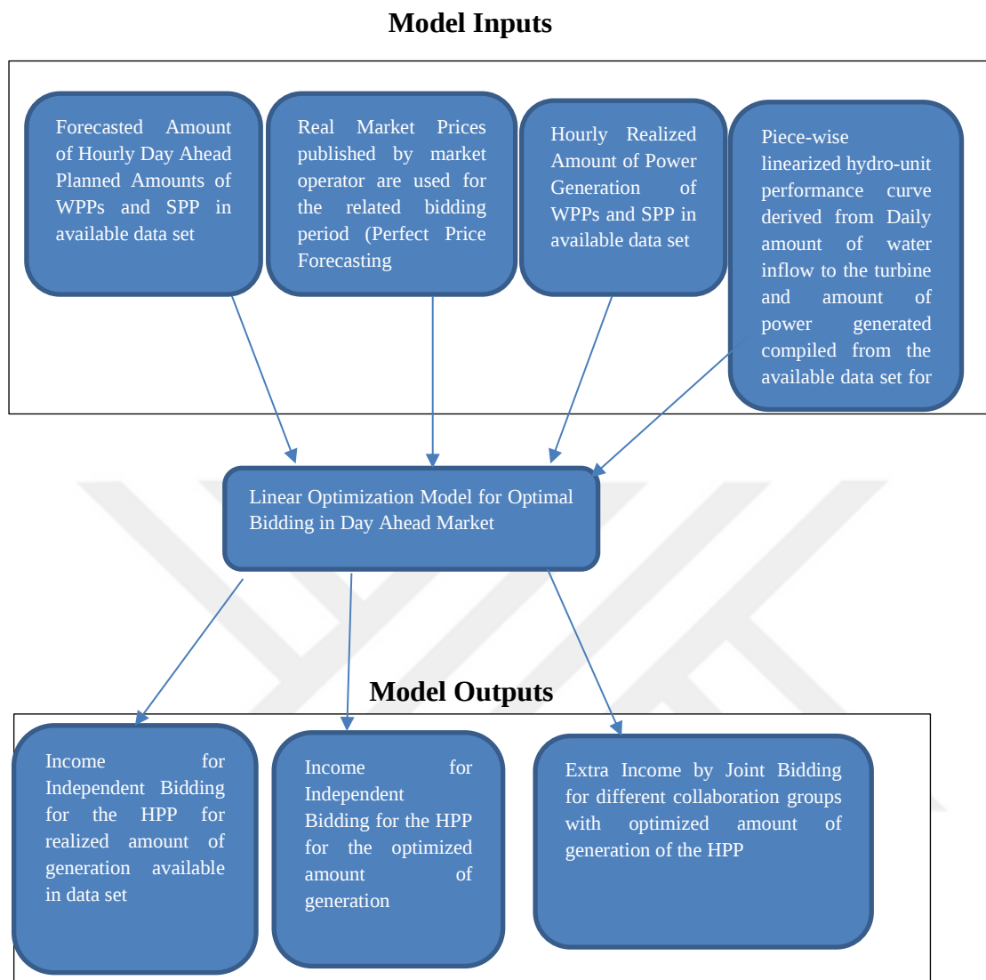
Figure 3. 18. Methodology for Joint Bidding Single-Hydro Model
