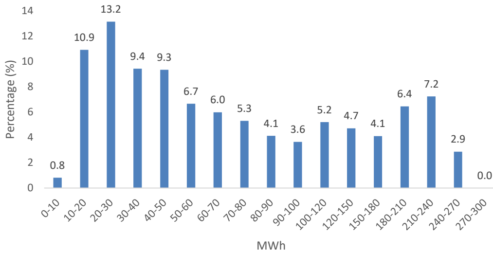
Figure 3. 10. The Distribution of Hourly Realized Generation Values of Hydro Power Plants with a Total Installed Capacity of 311 MW
