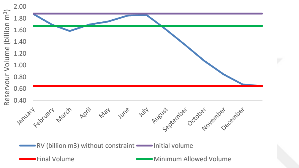
Figure 4. 1. Change in Reservoir Volume in the Absence of Reservoir Volume Limitations
