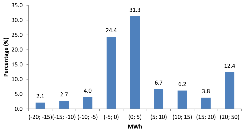
Figure 3. 12. Distribution of Hourly Imbalance Amounts for Hydro Power Plants with a Total Installed Capacity of 311 MW
