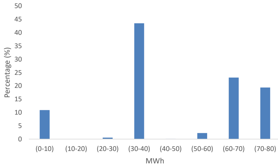
Figure 3. 14. The Distribution of Hourly Real Generation Values of Hydro Power Plant with a Total Installed Capacity of 80 MWs
