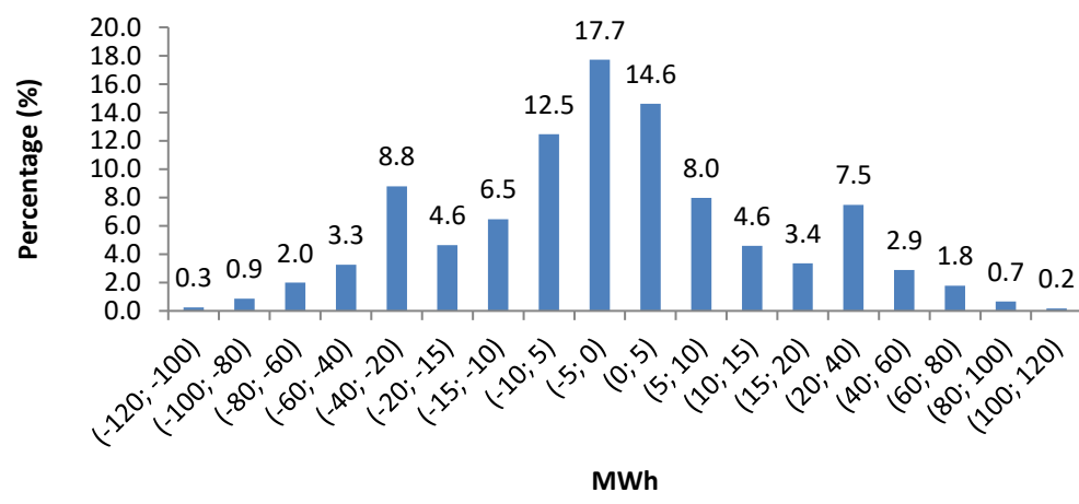
Figure 3. 8. Frequency Distribution of Amount of Imbalances for SPP
