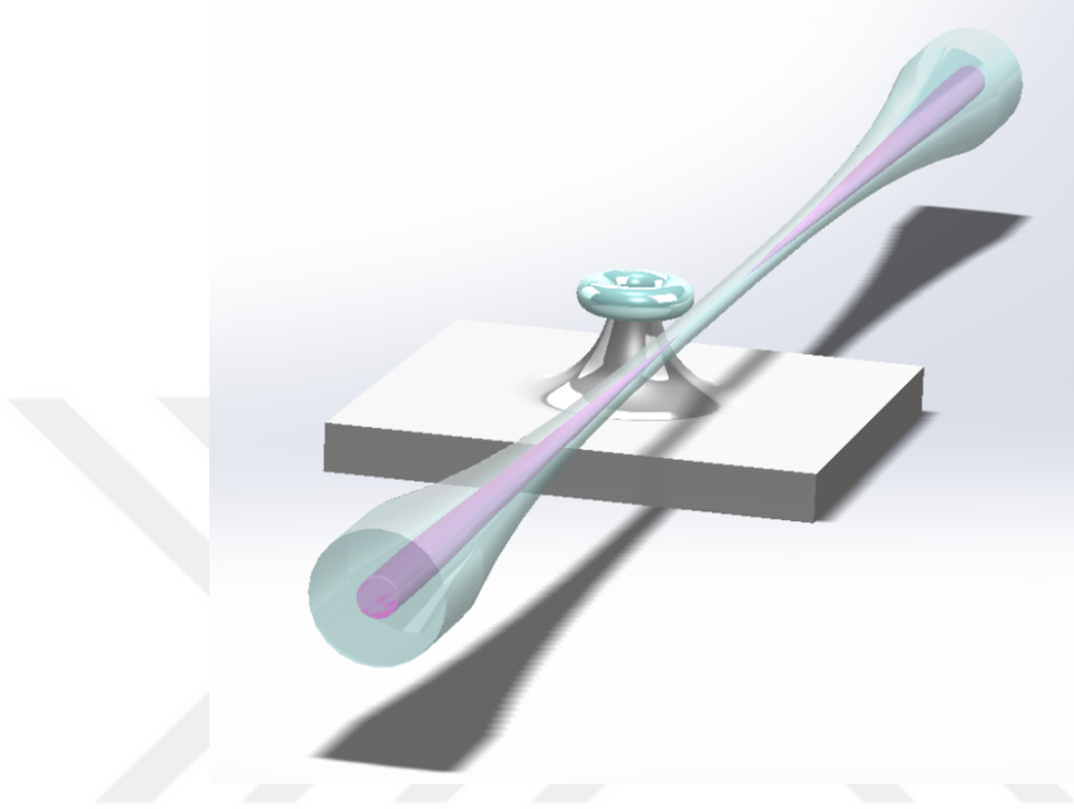
Figure 3.3: Light coupling into the toroidal resonator by using tapered optical fiber.
