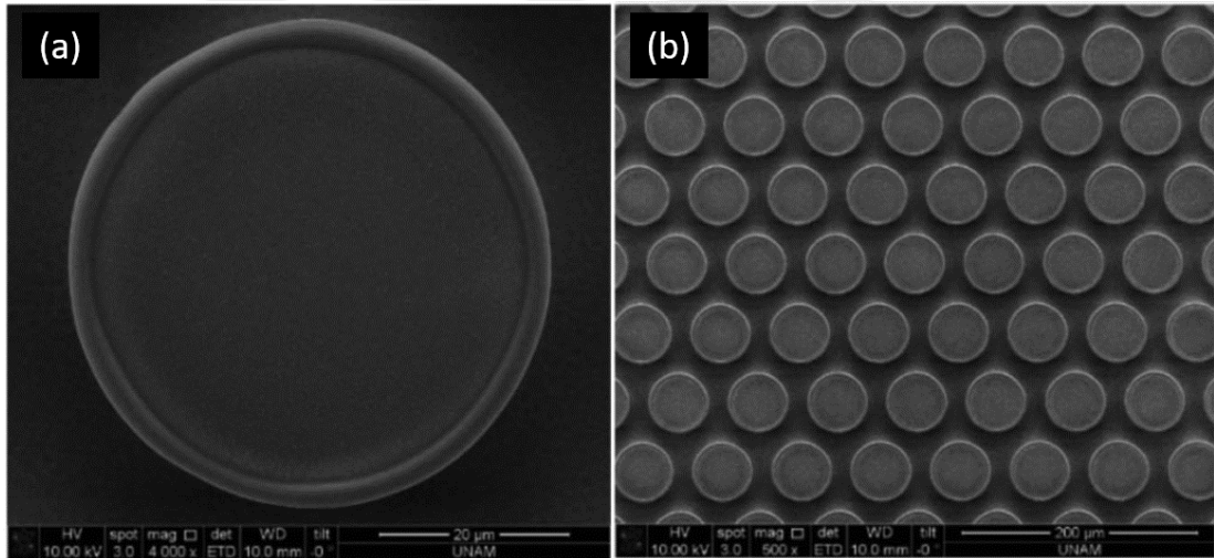
Figure 4.4: Scanning electron microscope images of (a) A single toroid in the array and (b) array of toroids on a chip.
