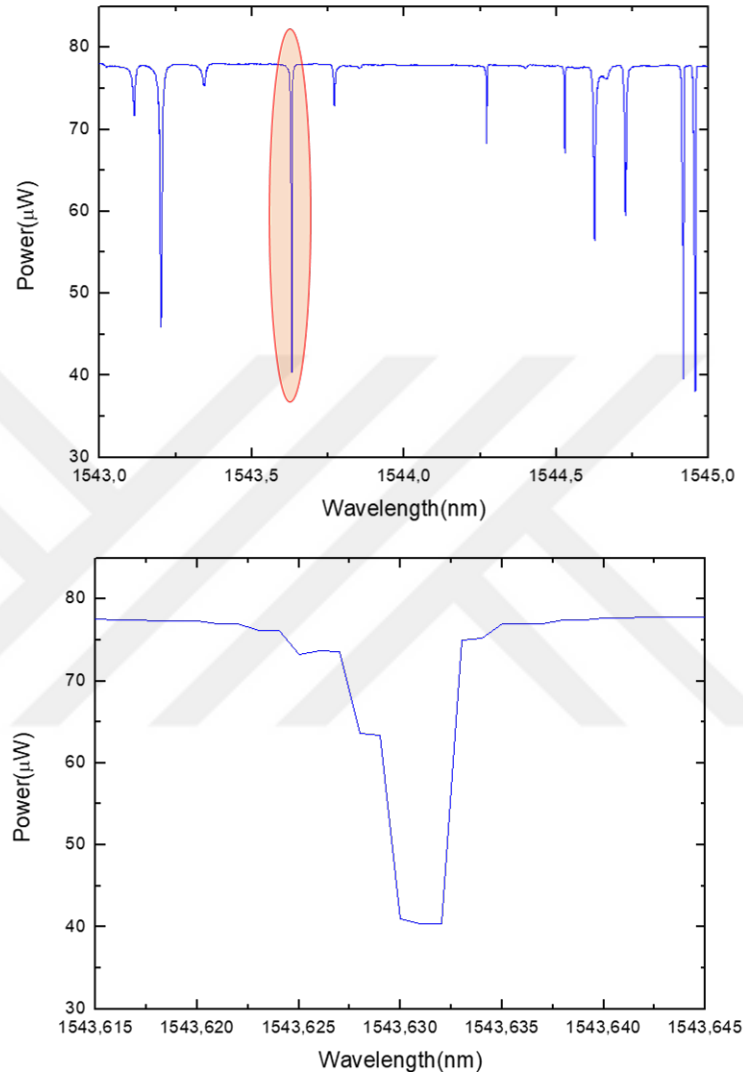
Figure 4.5: (a) Resonant mods recorded from a toroidal microresonator fabricated using raster scan diode laser. (b) One mod from the spectrum was chosen and detalied scan was conducted.
