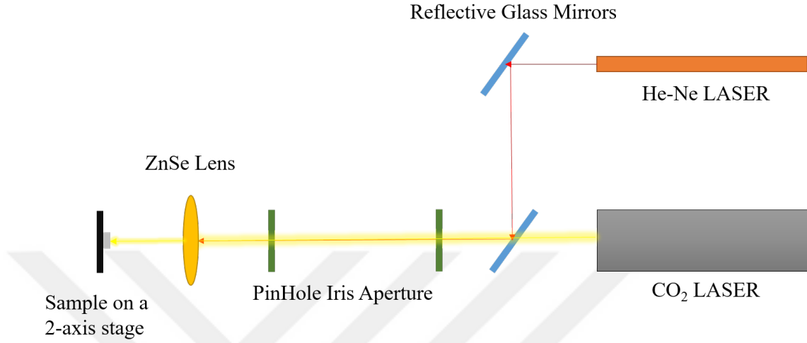
Figure 2.16: Illustration of the disk reflowing setup with carbondioxide laser.
