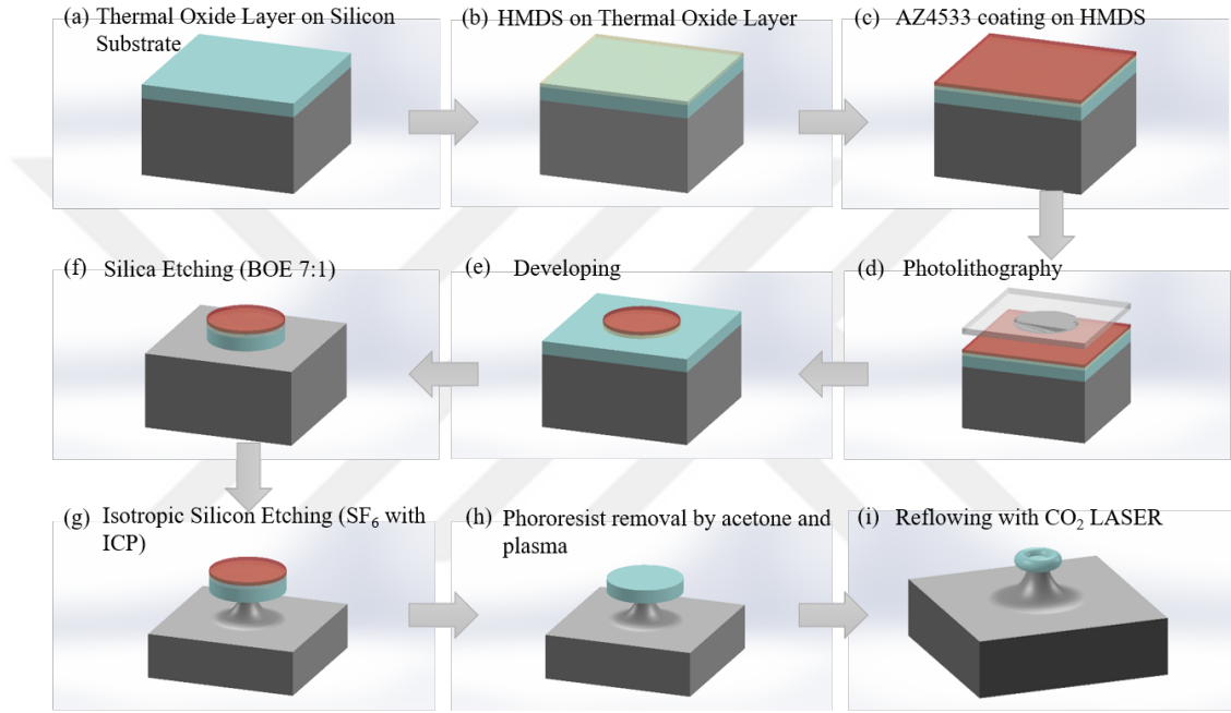
Figure 5.1: Silica microtoroid fabrication procedure from wafer to a toroidal resonator. (a) 20x30mm rectangular substrates diced from the wafer. (b) HMDS coating (yellow color) onto the substrate to enhance the bonding between the oxide layer (blue color) and photoresist. (c) Photoresist coating (red color) onto the substrate. (d) A designed mask with patterns on it is used to pattern the substrate by using photolithography. (e) The photoresist developing process is done in order to harden the photoresist to allow patterns on the substrate. (f) By using buffer oxide etchant (BOE 7:1), silica etching is done. The area under photoresist patterns is protected while the rest is etched. (g) Silicon etching is done after silica etching. The area under the silica undergoes isotropic etching to form a pillar while the rest is etched completely. (h) The photoresist is removed from the structure since there is no need for it anymore. (i) Silica microdisks on silicon pillars produced as a result of microfabrication are reflowed by using a CO 2 laser engraver.
