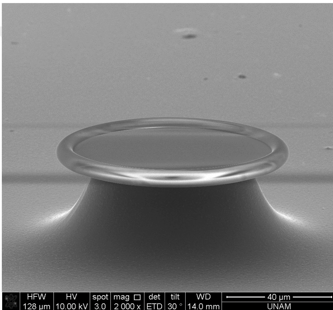
Figure 2.19: Tilted SEM image of a fabricated silica toroidal resonator.
