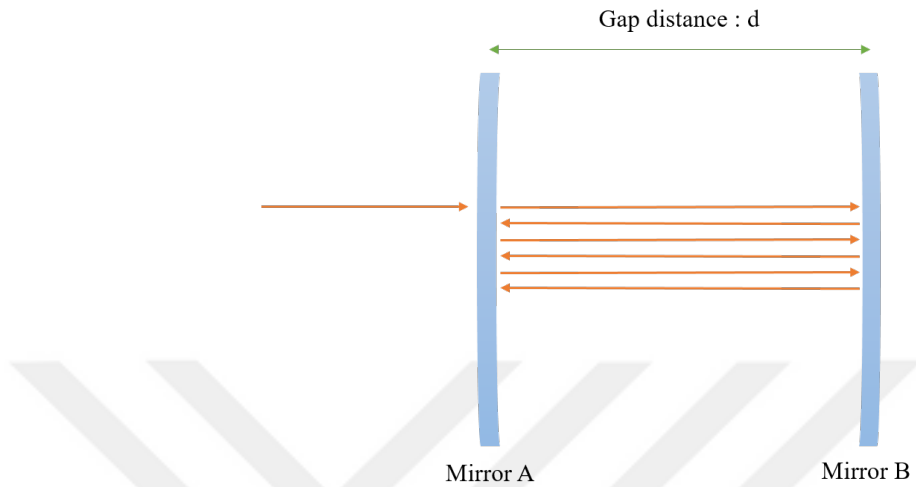
Figure 2.1: Schematic representation of a Fabry-Perot (two-mirror planar) resonator.
