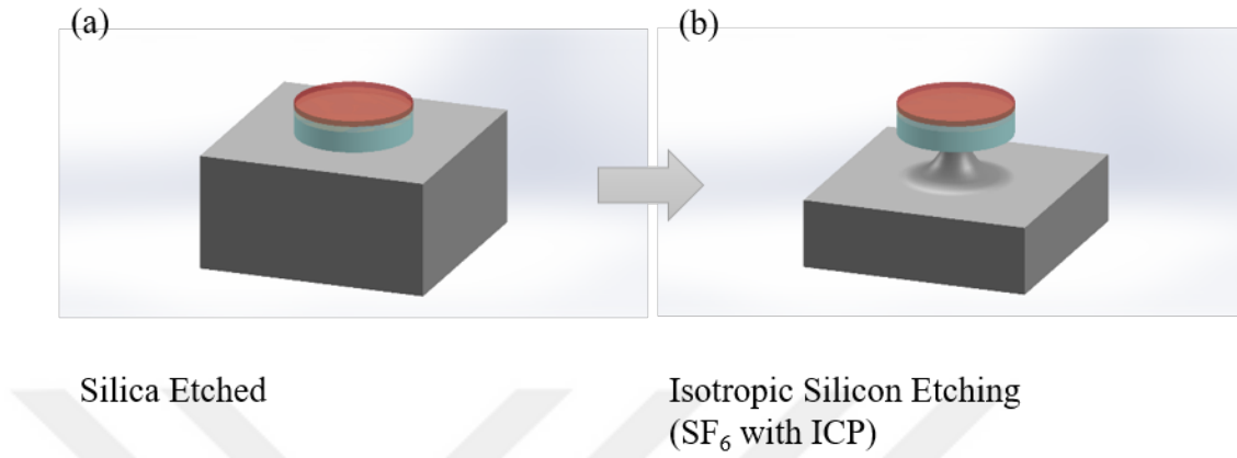
Figure 2.15: Isotropic etching of silicon layer under the silica disk. (a) Before silicon etching, (b) After silicon etching.
