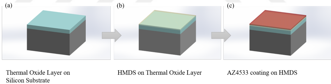
Figure 2.8: Spin Coating of a silicon substrate (gray color) with a thermal oxide layer (blue color) on top. (a) Diced substrate, (b) HMDS (yellow color) spin-coated substrate, (c) Photoresist (red color) coated substrate.
