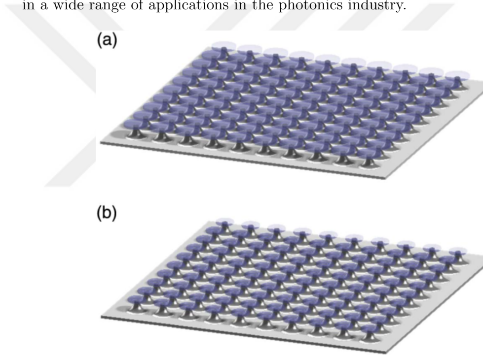
Figure 4.2: (a) Array of microdisks produced on a chip by standard microfabrication techniques. (b) The array of microdisks is reflowed to produce high Q-factor microtoroids.
