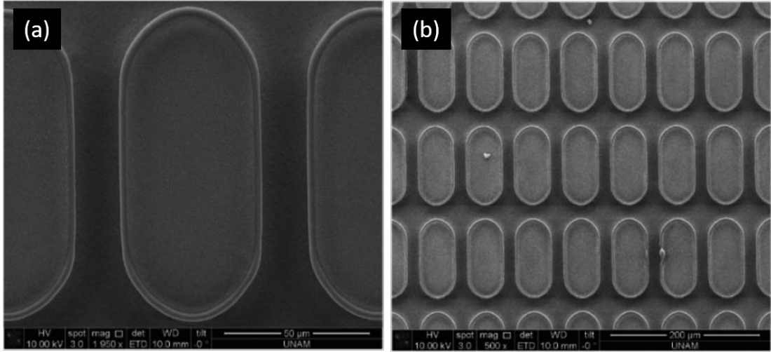
Figure 4.8: Scanning electron microscope images of (a) A single racetrack resonator in the array and (b) an array of racetrack resonators on a chip.
