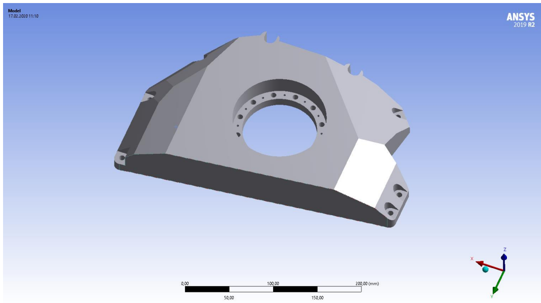
Figure 4.7. Final Optimized Design of the Gimbal Holder Part in the 1 st Optimization
