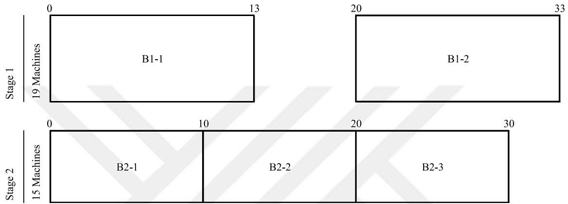
Figure 5.6. Placement of time blocks in the optimal schedule for S2-P16
