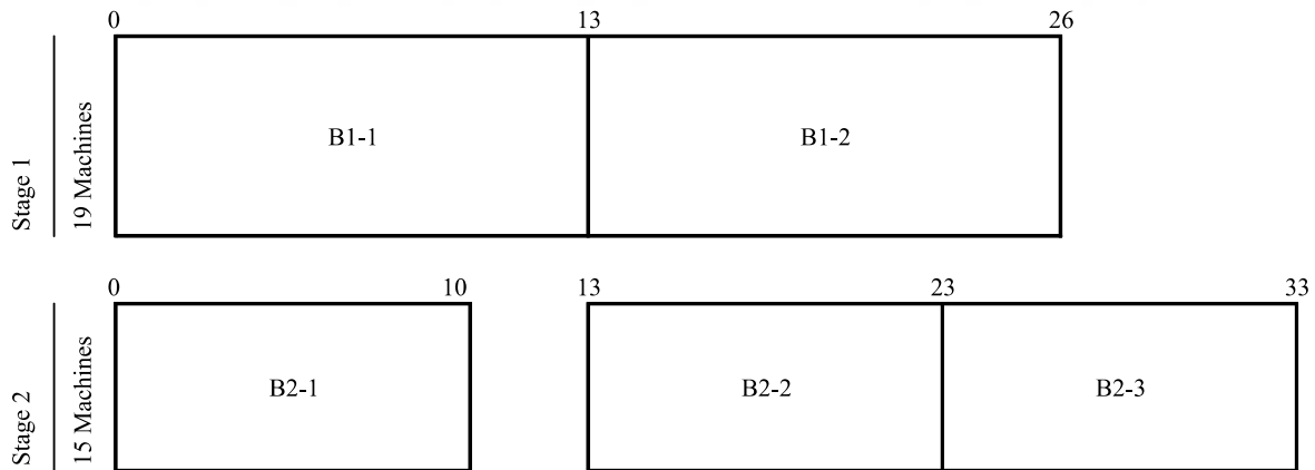
Figure 5.7. Alternative placement of time blocks in the optimal schedule for S2-P16
