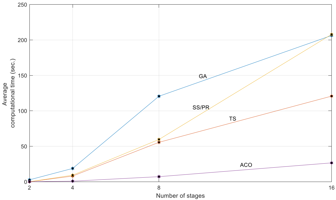
Figure 5.1. Change in computational time with increasing problem size
