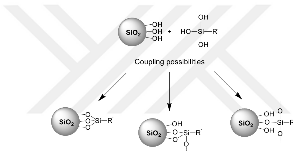
Figure 2.15 : Coupling possibilities of alkoxy silane precursors with silica particles.
