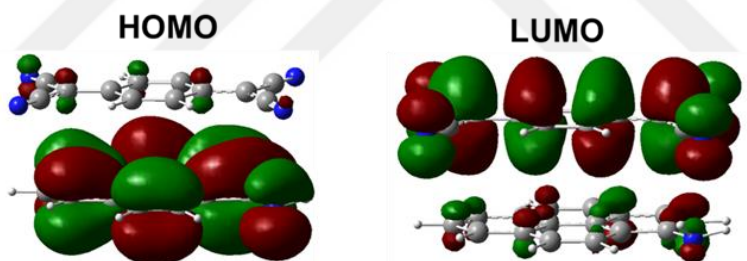
Figure 4.9. HOMO and LUMO orbitals mapped on the pairwise interactions of donor-acceptor charge transfer complex for -NH 2 substitutions on pyrene donor.
