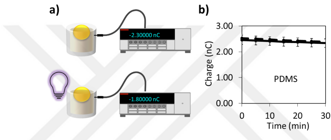
Figure 2.2. Contact charge and charge decay measurement setup for solid undoped and doped PDMS pieces. The pieces (shown in yellow in the scheme) are manipulated by tweezers, contact charged against Al foil, and immersed in a Faraday cup. a) The contact charge and charge decay measurements with a homemade Faraday cup attached to an electrometer. b) A typical charge decay plot of PDMS sample in dark (solid line) and under UV illumination (dashed line). The plots overlap since there is no effect of UV illumination on the decay rate of undoped samples. The error bars in the plot display the standard deviation calculated from five independent measurements.
