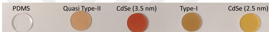
Figure 6.4. QD doped PDMS samples
