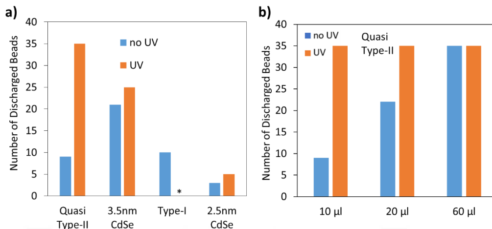
Figure 6.9. a) The number of discharged beads (N=35) in the first 5 minutes after the QD solution was added into the hexane in the glass vial with 35 contact-charged PTFE beads. * indicates the Type-I QDs did not discharged beads in 5 minutes under UV illumination. b) The number of discharged beads in 5 minutes vs added microliters of quasi-type-II QDs in the vials. All of beads discharged in 5 minutes in UV illumination.
