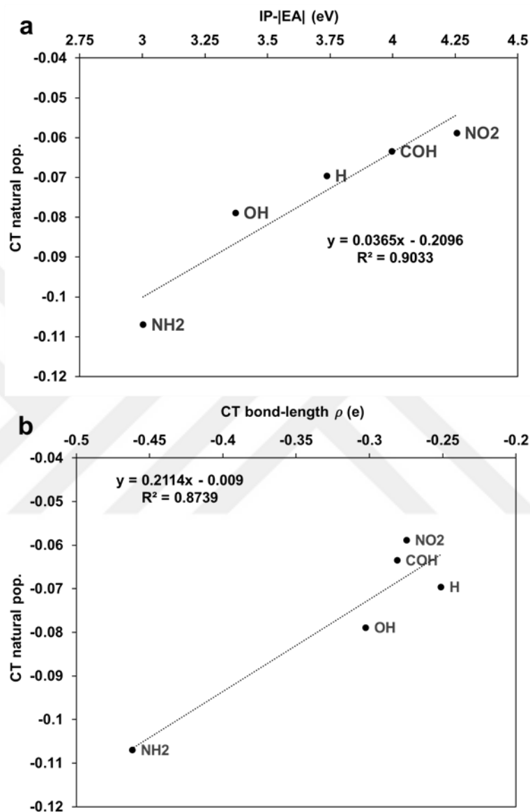
Figure 4.11. a) Correlation of IP - |EA| offset with the charge transfer based on NPA. b) Correlation of charge transfer from the bond lengths of acceptor ( \rho ) with the charge transfer based on the NPA.
