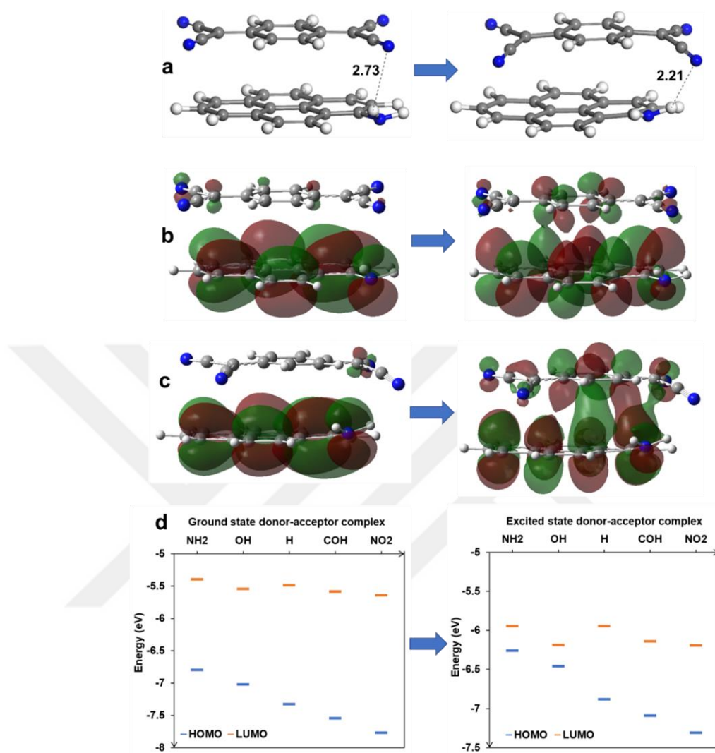
Figure 4.12. a) Optimized geometries for the ground state and first singlet excited state pairwise interactions for- \text{NH}_2 substitution, S_0 \rightarrow S_1 natural transition orbitals at the b) ground state optimized geometries and c) excited state optimized geometries, d) HOMO and LUMO energy levels for the ground state and excited state optimized geometries of binary complexes for different substitutions on the pyrene donor.
