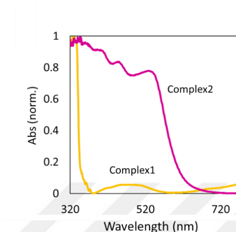
Figure 4.3. a) Solid state UV-visible spectra of pyrene-TCNQ (yellow) and 1-Aminopyrene-TCNQ (pink).
