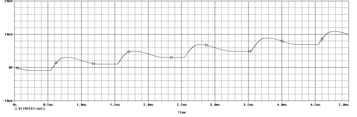
Figure 2.10: The plot of charge gain vs. time for a duration of 5ms when V = 5\text{V} , V_t \simeq 0.4\text{V} , C_{max} = 1\text{nF} , \gamma = 20 , f = 1\text{KHz} showing the charge transfer behavior.
