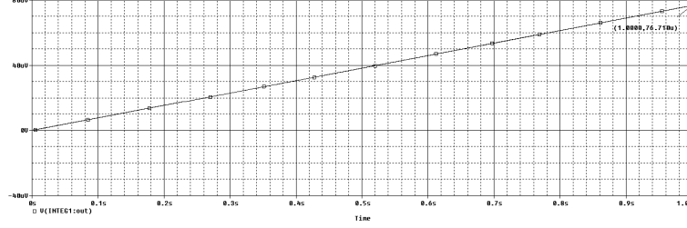
Figure 3.6: The plot of charge entering the reservoir vs. time for a duration of 1s when V = 5\text{V} , V_Q = 20\text{V} , V_t \simeq 0.4\text{V} , C_{max} = 1\text{nF} , \gamma = 20 , f = 1\text{KHz} and 5 capacitors are employed in the system.
