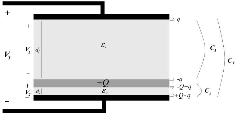
Figure 3.1: A charge embedded capacitor example. The capacitor is a parallel plate capacitor and there exists an electret in between the plates, and -Q charge is trapped in this electret. The structure can be treated as two capacitors in series, first arising between the top plate and the electret, and second between the electret and the bottom plate.
