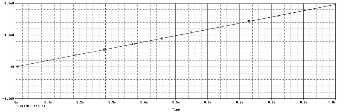
Figure 2.11: The plot of charge gain vs. time for a duration of 1s when V = 5\text{V} , V_t \simeq 0.4\text{V} , C_{max} = 1\text{nF} , \gamma = 20 , f = 1\text{KHz} , showing the consistency of the theoretical calculations and simulations.
