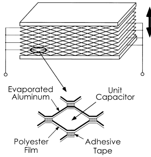
Figure 4.8: Honeycomb capacitor
