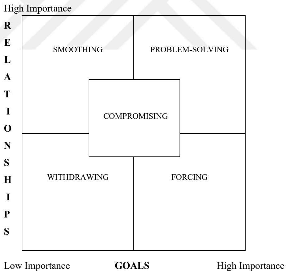
Figure 1: Conflict Strategies
