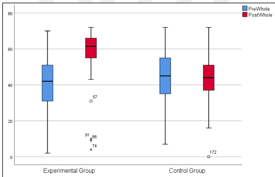
Figure 6. Extreme Values from Computational Thinking Skills Self-Efficacy Scale
