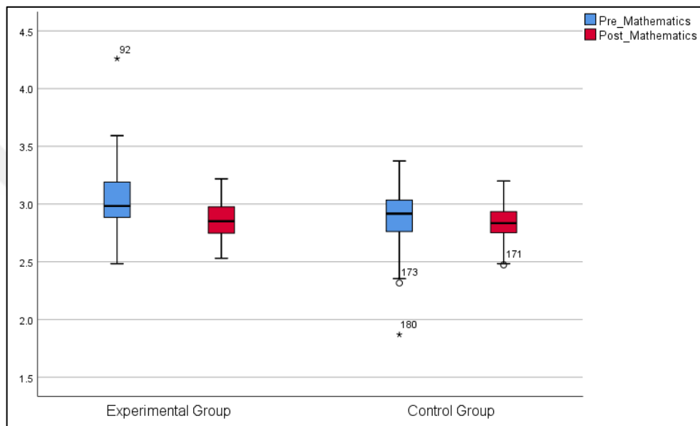
Figure 3. Extreme Values Obtained from Mathematics Attitude Scores
