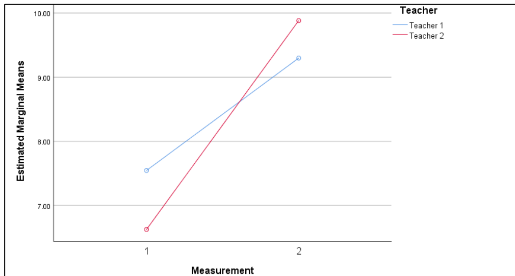
Figure F.3 Effect of Pretest Scores and Teachers' Attitude on Computer Programming Self-Efficacy Scale Posttest Scores
