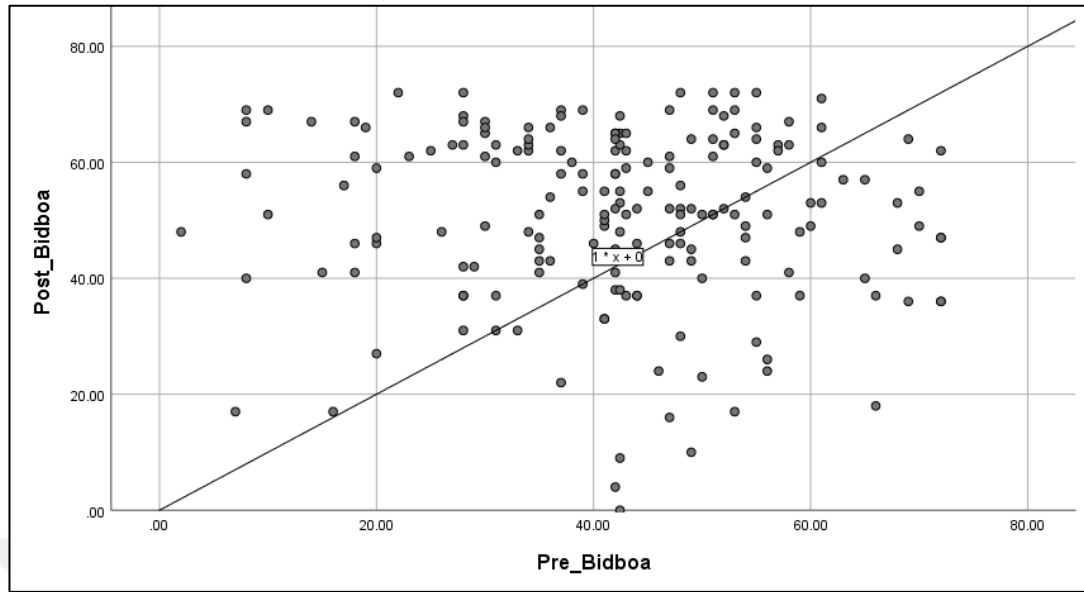
Figure 7. Outliers of Computational Thinking Skills Self-Efficacy Scale (Pretest–Posttest)
