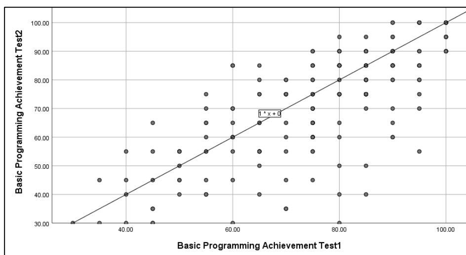
Figure 11. Outliers of Small Basic Programming Achievement Test (Pretest–Posttest)
