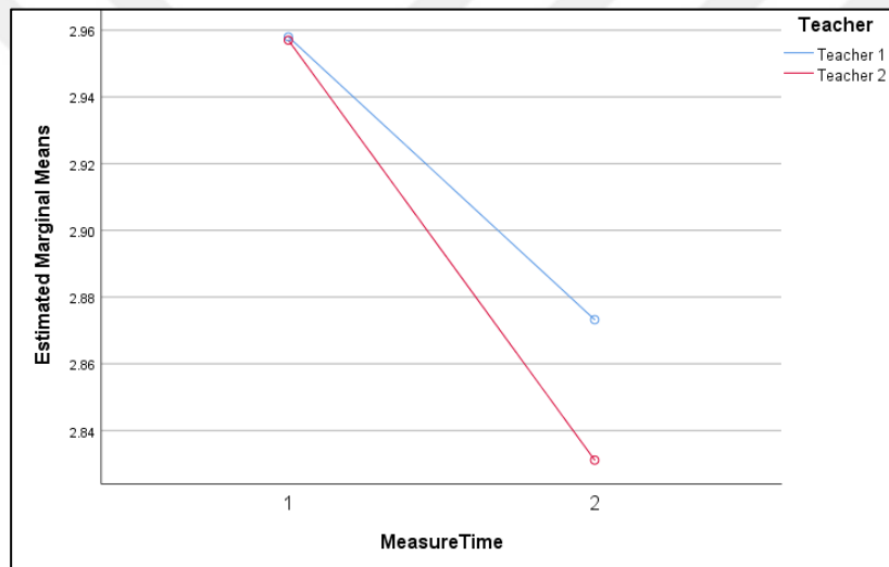
Figure F.1. Effect of Pretest Scores and Teachers' Attitude on Mathematics Attitude Scale Posttest Scores
