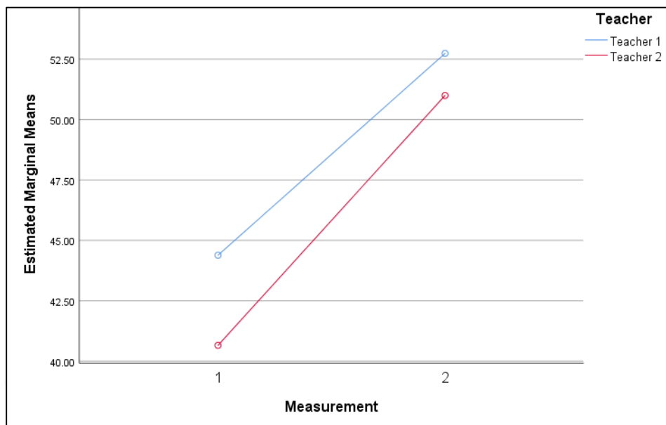
Figure F.2. Effect of Pretest Scores and Teachers' Attitude on Computational Thinking Skills Self-Efficacy Scale Posttest Scores
