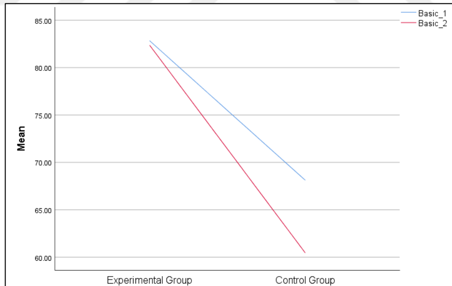
Figure 13 Differences Between Groups for Students' Small Basic Programming Achievement (Pretest–Posttest) Scores
