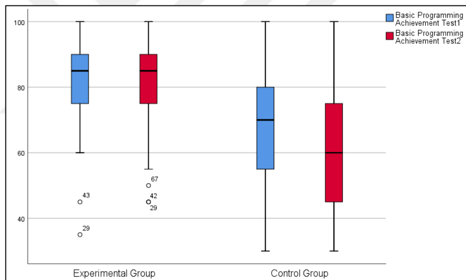
Figure 10. Extreme Values from Small Basic Programming Achievement Tests
