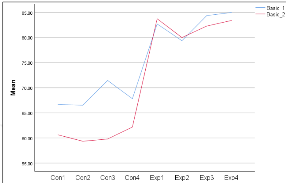
Figure 12. Differences Between Groups for Students' Small Basic Programming Achievement Test Pretest–Posttest Scores
