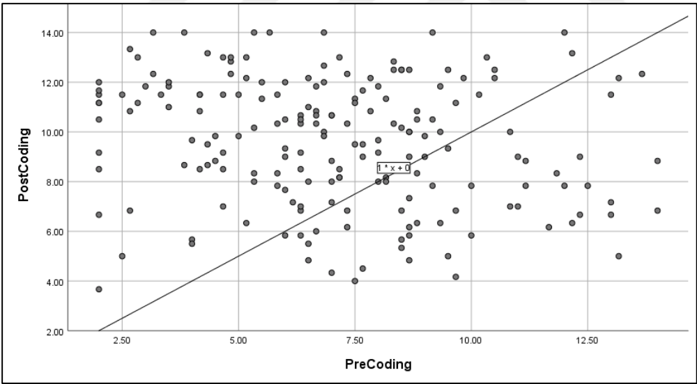
Figure 9. Outliers of Computer Programming Self-Efficacy Scale Pretest–Posttest Applications
