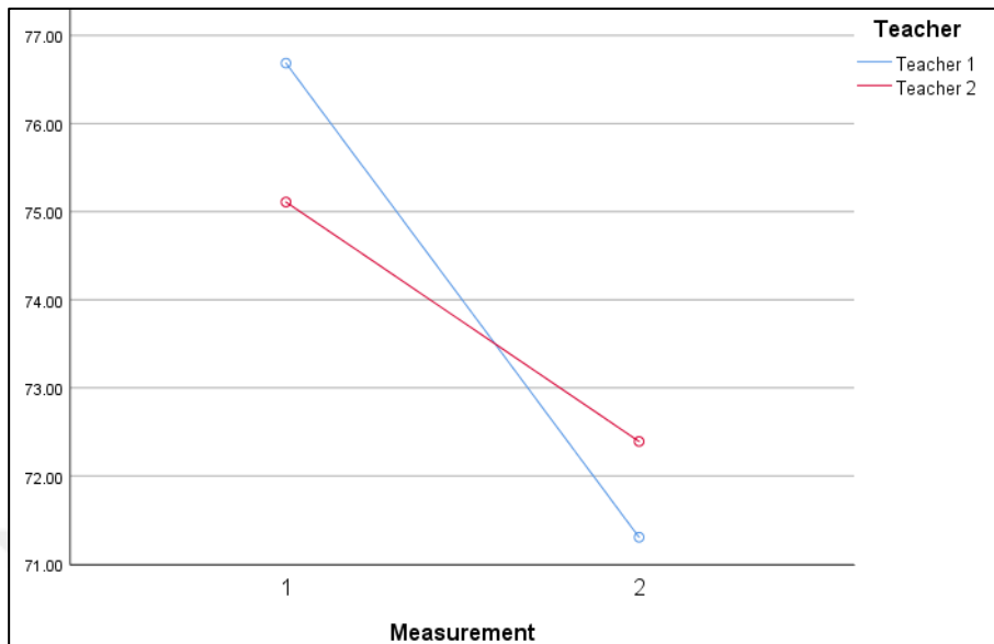
Figure F.4 Effect of Pretest Scores and Teachers' Attitude on Small Basic Programming Achievement Test's Posttest Scores
