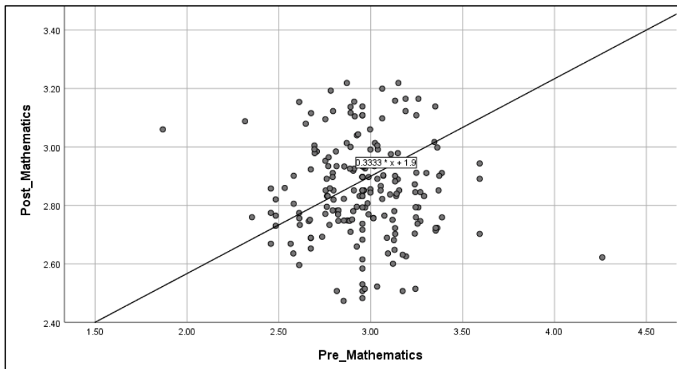
Figure 4. Outliers of Mathematical Attitude Pretest–Posttest Scores
