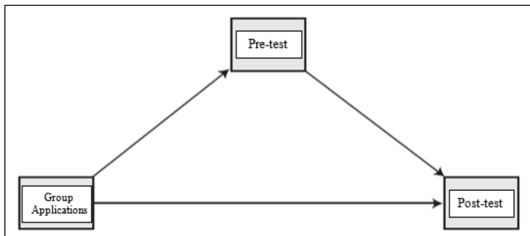
Figure 5. Conceptual Diagram of Multiple Regression Analysis
