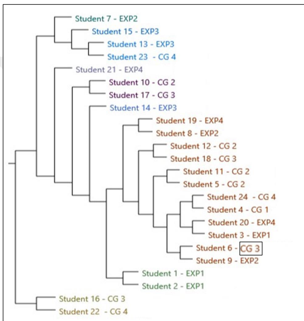
Figure 15. Similarities Between Students' Views (by Group)
