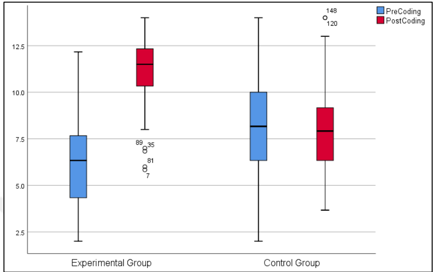
Figure 8. Extreme Values from Computer Programming Self-Efficacy Scale
