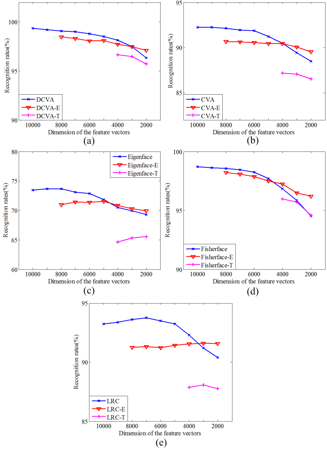
Figure 3.8 Recognition rates of (a) DCVA, (b) CVA, (c) Eigenface, (d) Fisherface, and (e) LRC in AR face database with original images, the face images cropped elliptically and in T —shape with respect to the dimension of the feature vectors.
