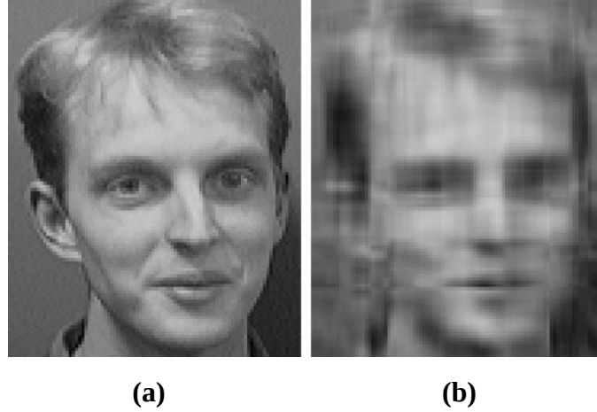
Figure 4.6 (a) The original image, (b) the approximated image evaluated using SVD.
