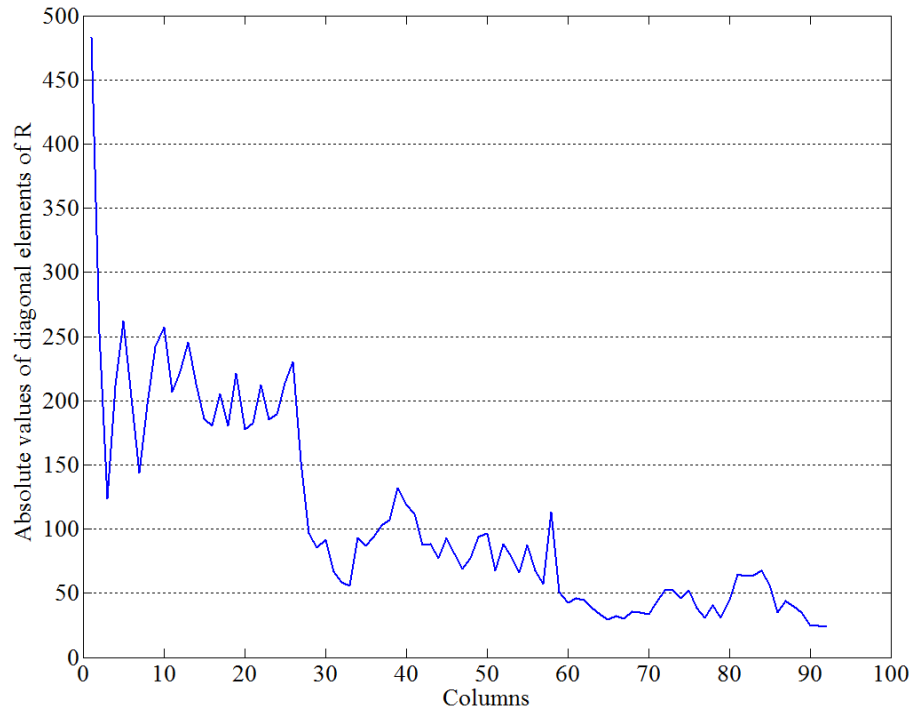
Figure 4.1 The absolute values of diagonal elements of \mathbf{R} evaluated from QR decomposition
