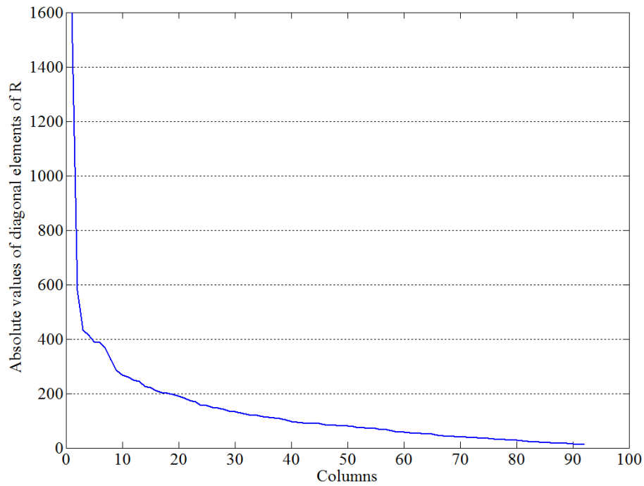
Figure 4.2 The absolute values of diagonal elements of \mathbf{R} evaluated from QRCP decomposition
