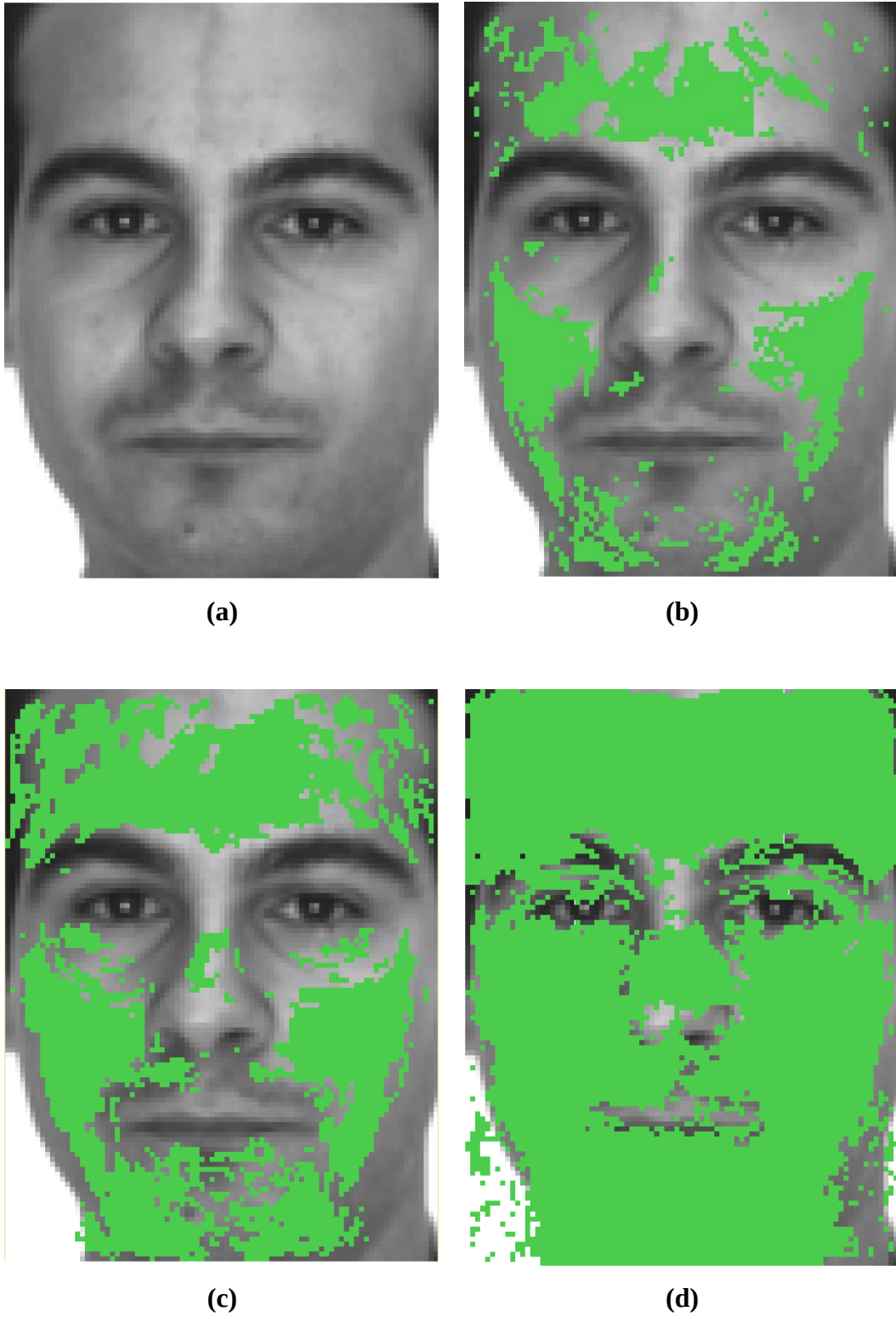
Figure 3.2 (a) Original image and (b) 2000, (c) 4000, and (d) 8000 pixels eliminated images, using the proposed feature selection method.
