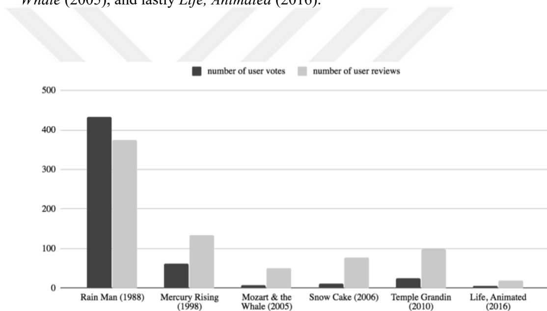
Figure 1: Number of IMDb user rating votes and reviews for the selected films
