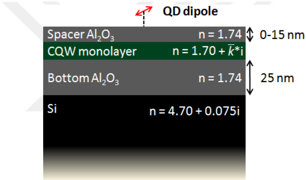
Figure 4.8: Schematic cross-section of the layered media below an isotropic QD dipole. For the only-donor system, there are no CQW or spacer layers. For the FRET system without a spacer, there is no \text{Al}_2\text{O}_3 layer on top. \bar{k} is 0.065 for the face-down CQW monolayer and 0.080 for the edge-up one.
