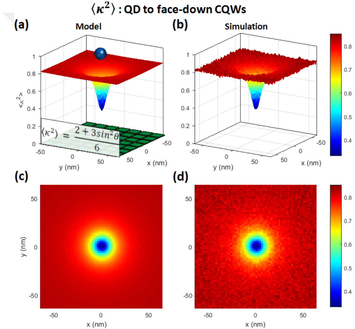
Figure 4.5: Variation of the average dipole-dipole orientation factor \langle \kappa^2 \rangle as a function of the coordinates of the dipole of a face-down CQW (a) calculated by the formula (Equation 4.18) and (b) estimated by the Monte-Carlo simulations. The QD and the CQWs are drawn out of scale for clarity purposes. (c), (d) Top-view of the surfaces in (a), (b), respectively.
