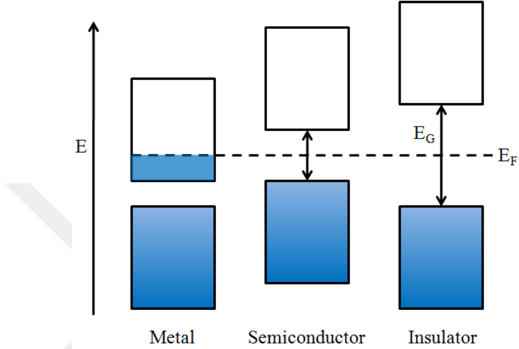
Figure 2.1: Representative band alignments with respect to the Fermi level E_F and band filling at absolute zero temperature. For semiconductor and insulators, the highest occupied band (valence band) and the lowest unoccupied band (conduction band) are separated by an energy gap E_G , which is called the bandgap.
