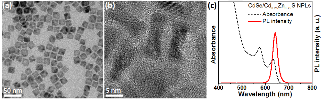
Figure 3.5: (a) Transmission electron micrograph of CdSe/Cd 0.25 Zn 0.75 S CQWs used for their self-assembly. (b) TEM image of the same CQWs in vertical orientation. (c) Absorbance (dashed black line) and photoluminescence (solid red line) spectra of these CQWs. Adapted from Ref. [131]
