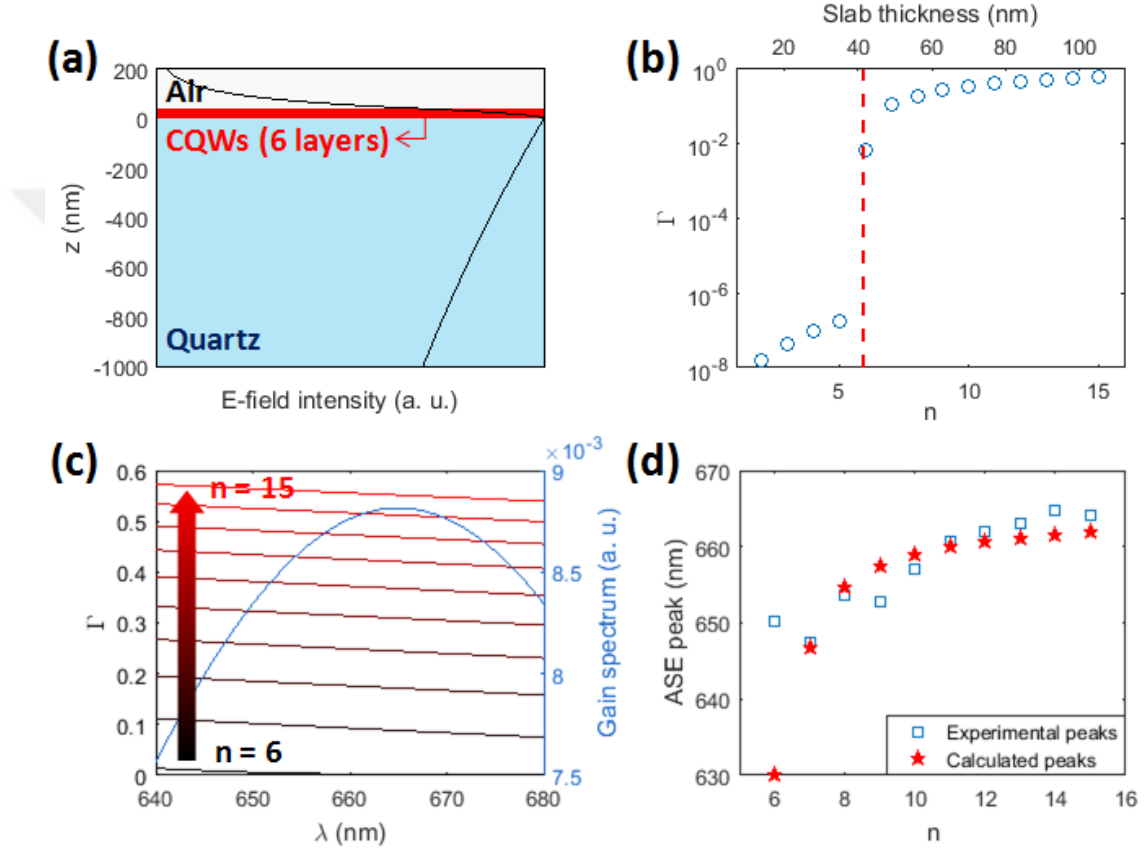
Figure 5.4: (a) Field intensity profile of the fundamental TE mode numerically calculated for the CQW slab with n = 6 . (b) Optical confinement factor \Gamma calculated at 650 nm for varied numbers of CQW layers (and slab thickness). Dashed line indicates the critical thickness of 41.2 nm for the existence of propagating modes within the slab. (c) Left axis: Variation of the confinement factor \Gamma with wavelength for different numbers of layers. Right axis: Gain spectrum \Gamma(\lambda) for our CQWs estimated using the measured ASE peaks at different film thicknesses, modeled as a Gaussian centered at 665 nm with a FWHM of 106.6 nm (blue) (d) ASE peaks calculated as the maximum of \Gamma(\lambda) \times G(\lambda) for each n (red stars), together with the experimentally measured ASE peaks (blue squares). Adapted from Ref. [131].
