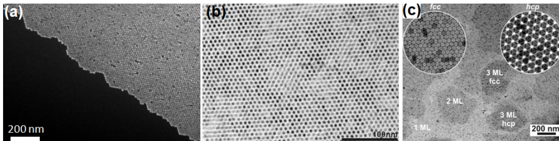
Figure 2.8: (a) Scanning electron micrograph of self-assembled monodisperse QDs forming a 2D hexagonal lattice. (b) Self-assembly of vertically oriented NRs. Adapted with permission from Ref. [84]. Copyright 2010 American Chemical Society. (c) Colloidal QD superlattices with face-centered cubic (fcc) and hexagonal close packed (hcp) crystal structures in different regions. Adapted with permission from Ref. [82]. Copyright 2010 American Chemical Society.
