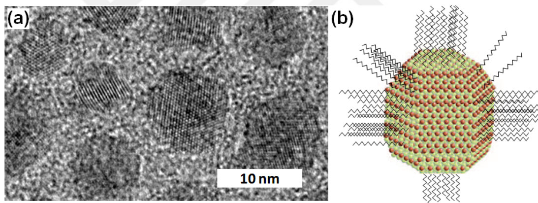
Figure 2.5: (a) Transmission electron micrograph of CdZnS/ZnS QDs synthesized and imaged by our group. (b) Schematic depiction of a quasi-spherical colloidal nanocrystal together with ligands on facets. Ligands on some facets are not drawn for clarity purposes. Adapted with permission from ref. [31]. Copyright 2008 American Chemical Society.
