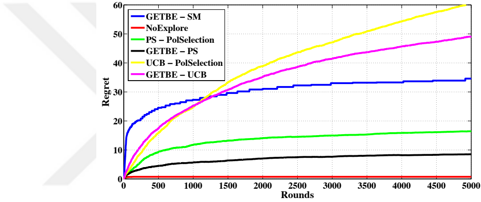
Figure 2.3: Regrets of GETBE and the other algorithms as a function of the number of rounds. when transition pair is in exploration region ( p^u = 0.65, p^F = 0.3, G = 4 ).
