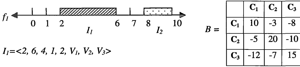
Figure 4.3: An example interval formation
