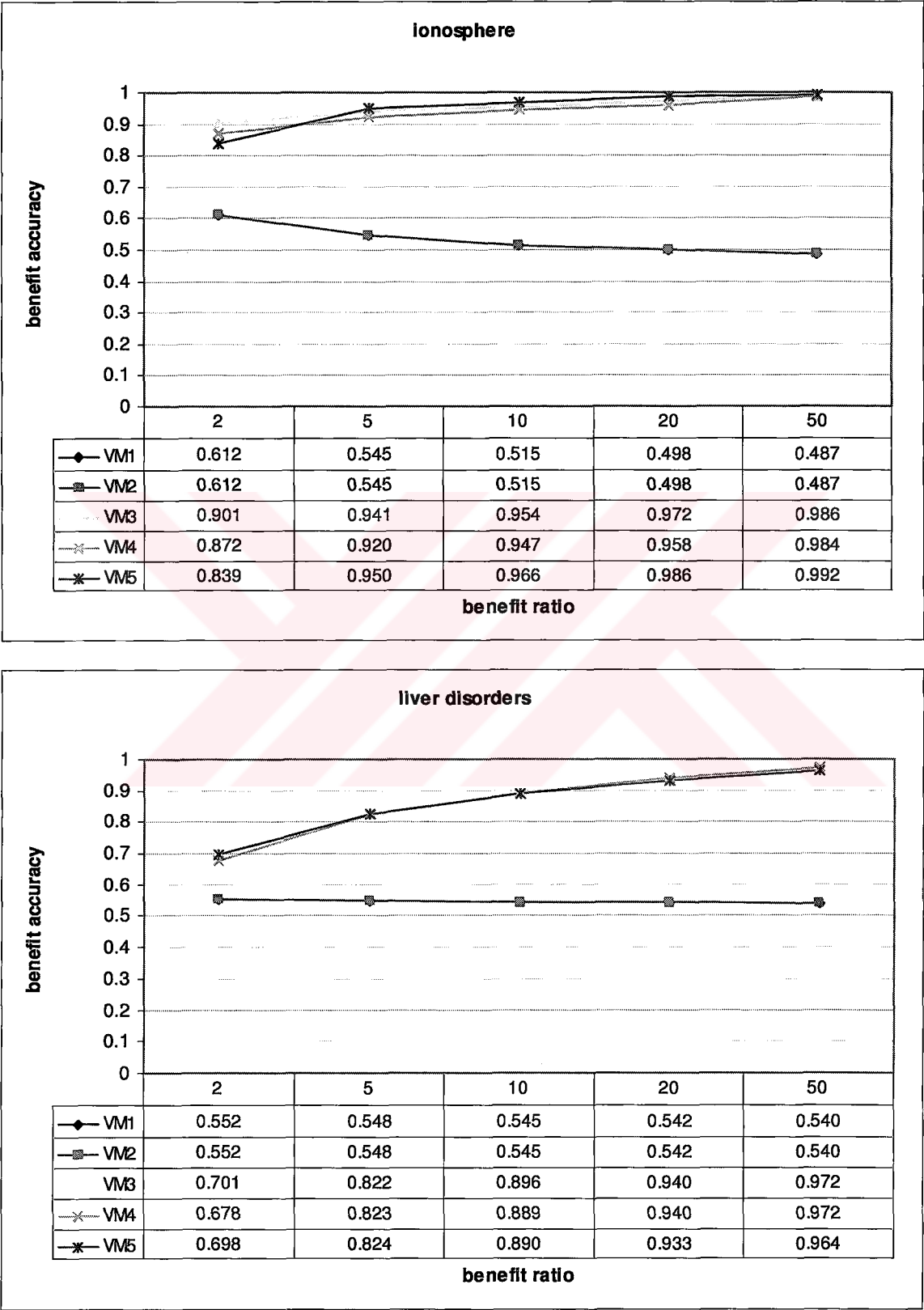
Figure 5.1(cont.): Behavior of voting methods on two-class benchmark datasets
