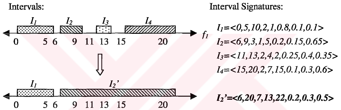
Figure 4.8: Example for illustrating merging high confidence intervals
