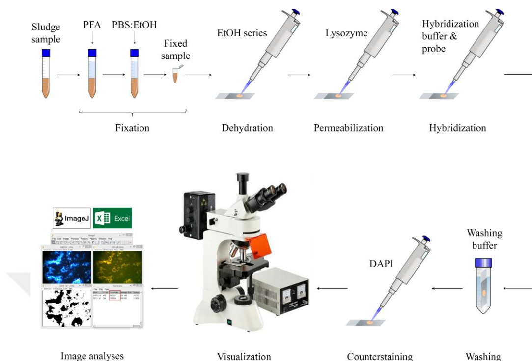
Figure 3.8. Schematic diagram of FISH procedure followed in the study
