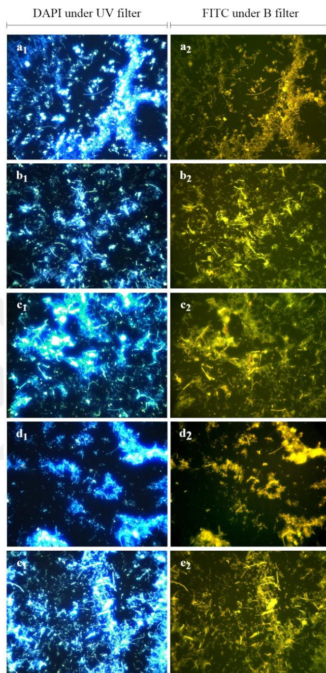
Figure 4.34. Representative hybridization images for methanogenic probes of MX825 (a 1 -a 2 ), MS1414 (b 1 -b 2 ), MG1200 (c 1 -c 2 ), MB1174 (d 1 -d 2 ) and ARC915 (e 1 -e 2 ) at optimal stringency conditions. Total microorganisms stained with DAPI (a 1 , b 1 , c 1 , d 1 , e 1 ) and target microorganisms hybridized with FITC-labeled probes for corresponding areas (a 2 , b 2 , c 2 , d 2 , e 2 )
