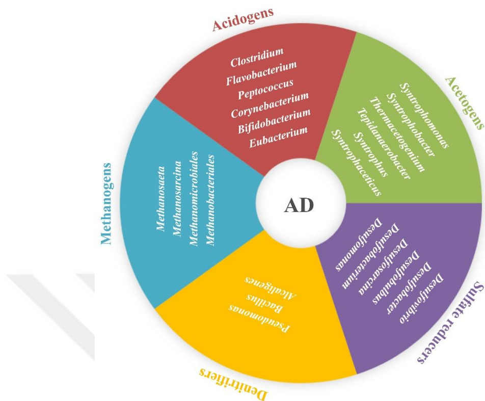
Figure 2.8. Schematic diagram of microbial communities and their representative members in anaerobic digesters
