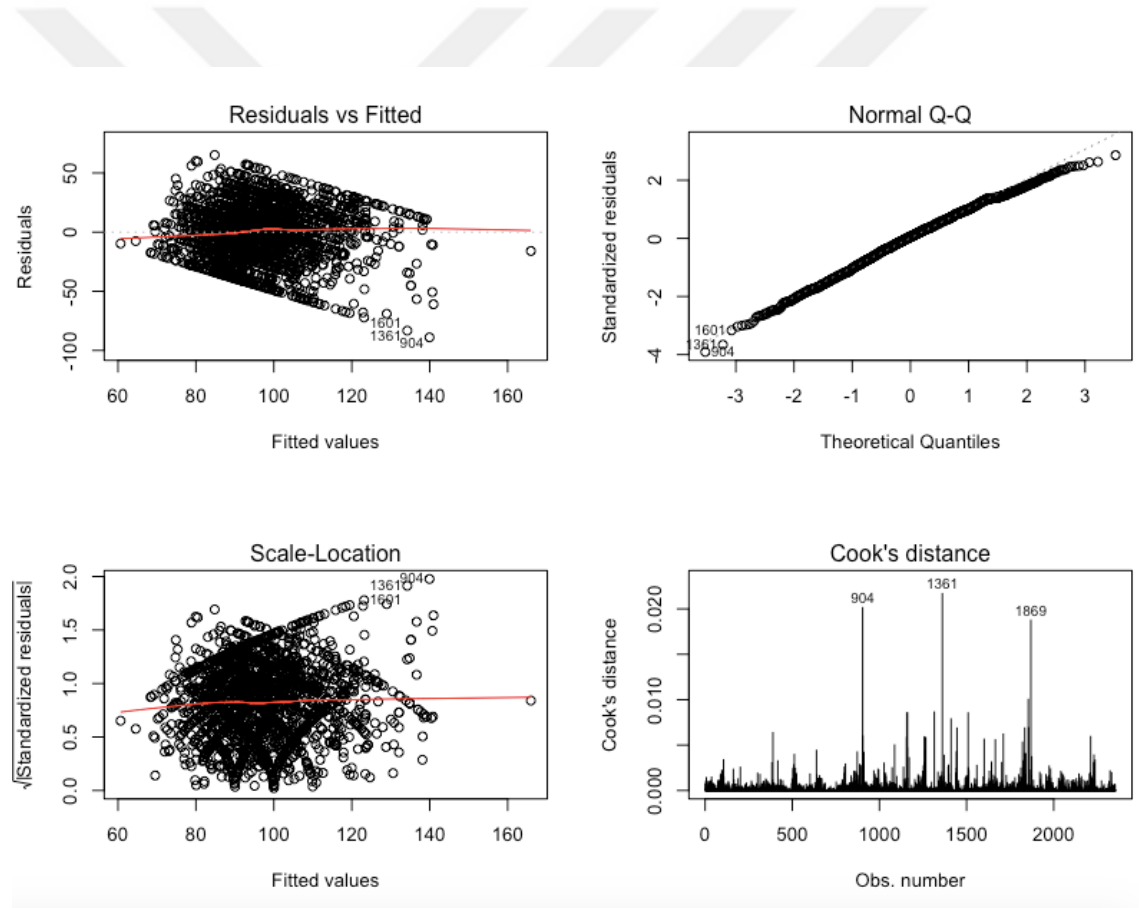
Figure 5: Model Diagnostics
