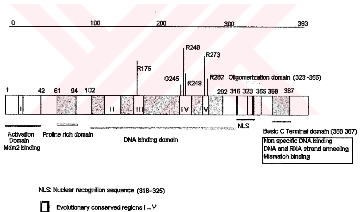
Fig.1. Schematic presentation of human p53. Several hot spots for mutations R175, G245, R248, R249, R273, R282 are also indicated
