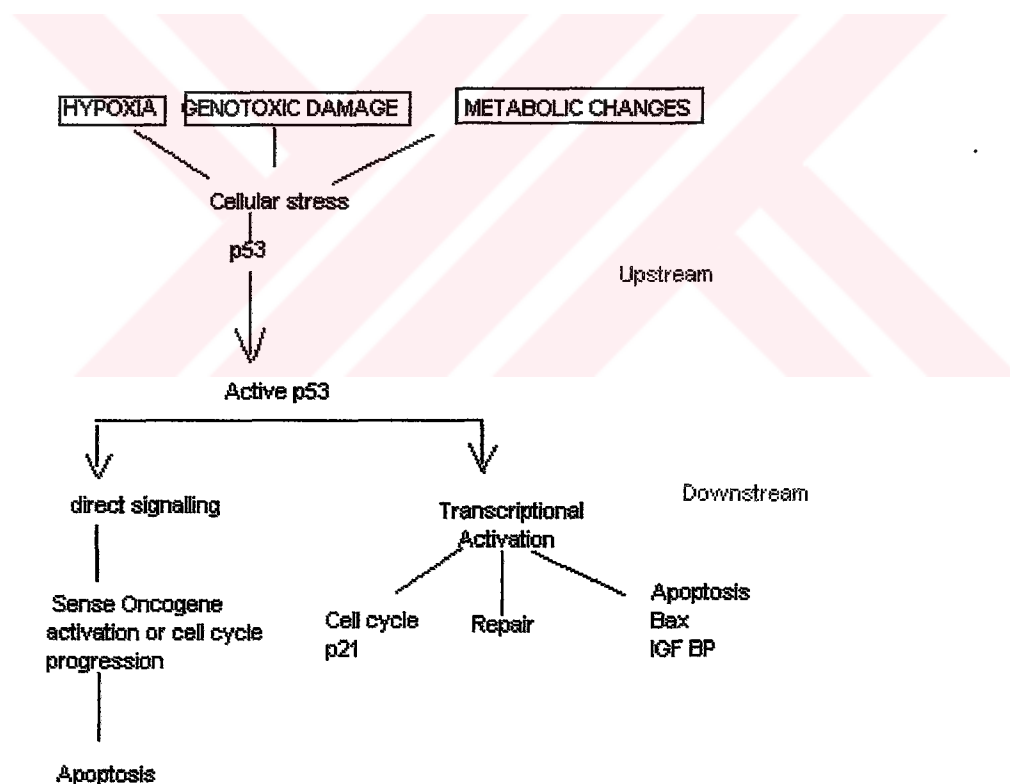
Figure 2. The p53 pathway Levine, A. J. 1997
