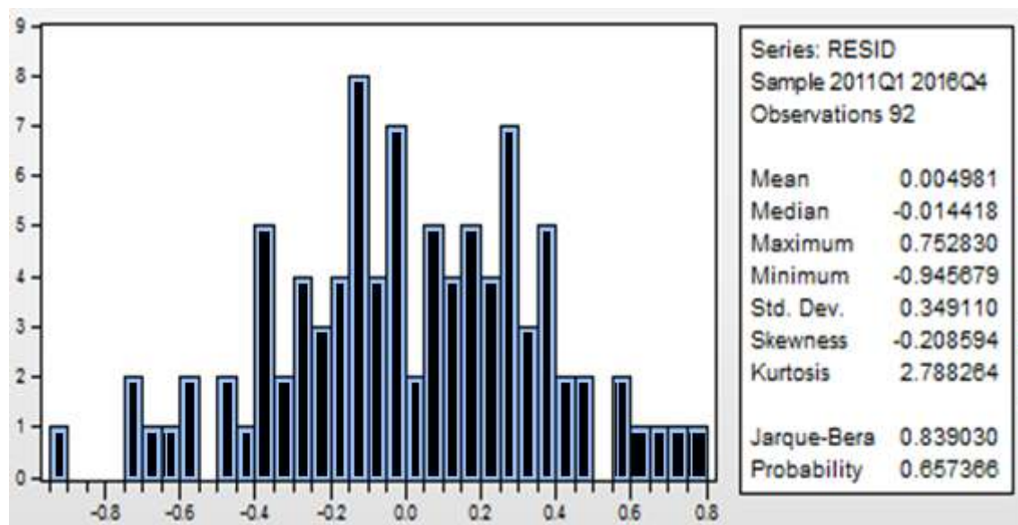
Figure 4.8 Histogram & Normality Test for Residuals
