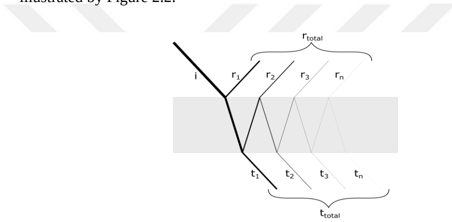
Figure 2.2. Multiple beams reflected from and transmitted through a non-absorbing dielectric slab.
