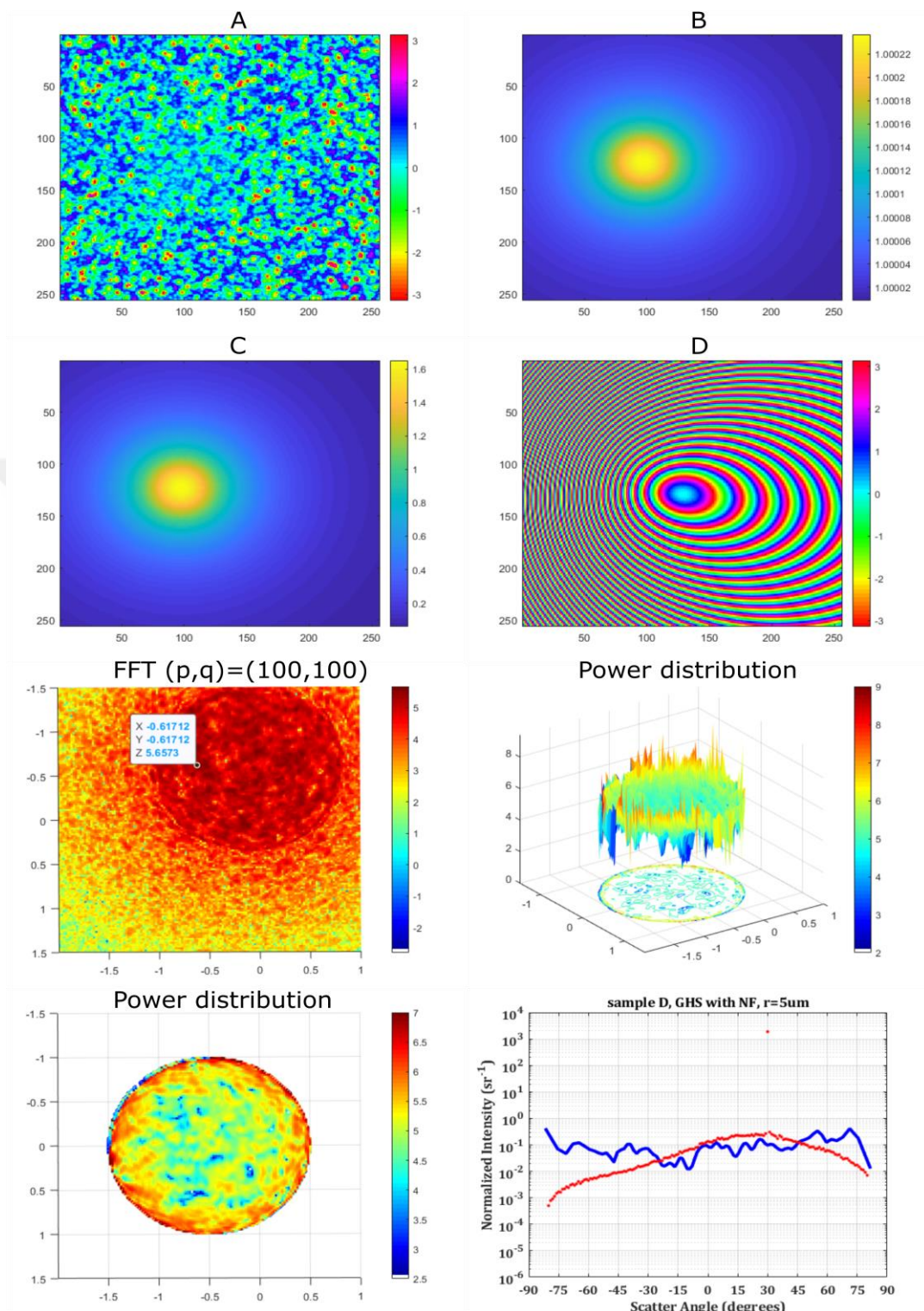
Figure 5.5. Select calculation steps for r=5\mu\text{m} , \theta_i=15.508^\circ ( \theta_t=30^\circ )
