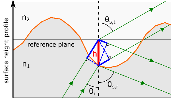
Figure 4.9. GHS interface optical path difference accumulation model.
