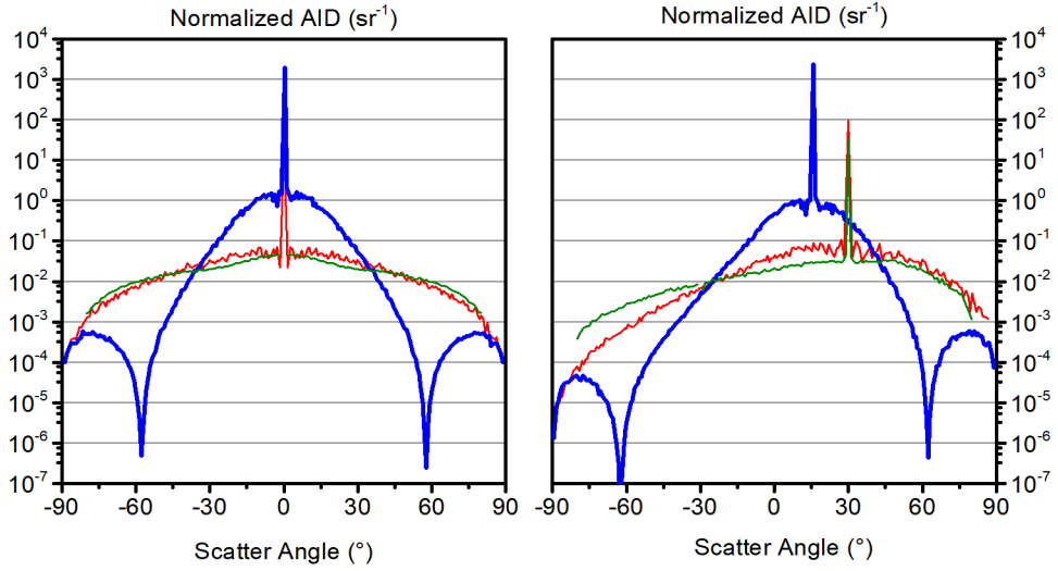
Figure 4.17. AID calculations for light scattering from sample D, for 0° and 30° incidence from air. Blue lines show transmission into n_s=1.87 , red lines show reflection into air, (green) lines show reflection measurements.
