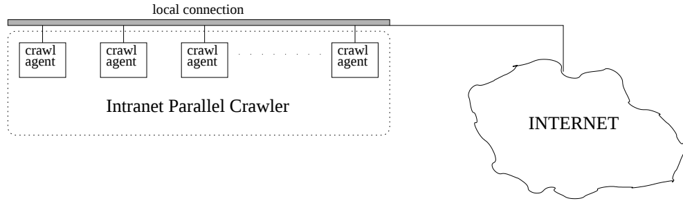
Figure 3.3: Architecture of an intranet crawler
