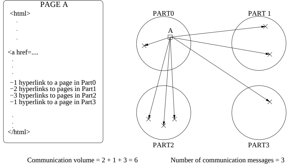
Figure 5.1: Communication volume vs. number of messages.
