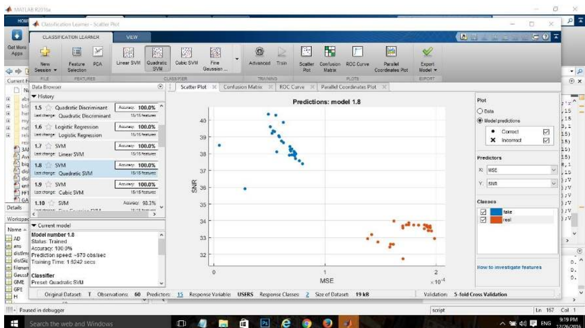
Figure C.10: Scatter plot
