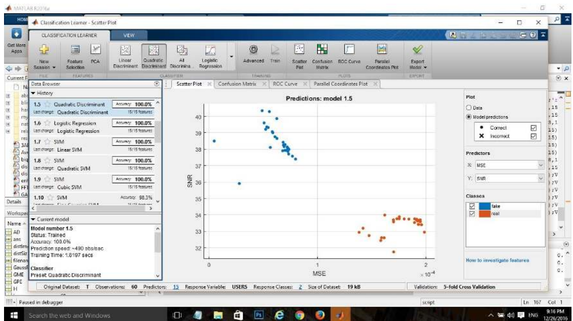
Figure C.4: Scatter plot
