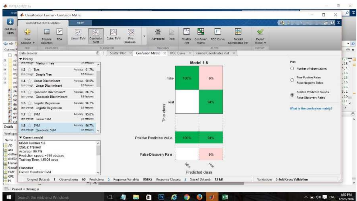
Figure C.25: Confusion matrix
