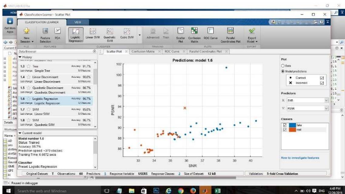
Figure C.27: Scatter plot
