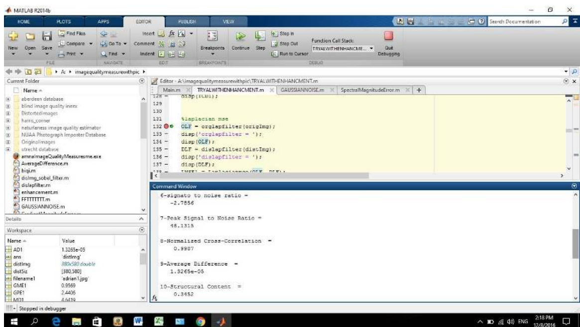
Figure: E.30: Results obtained from the present experiment on Gaussian noise, mean 0, variance 1
