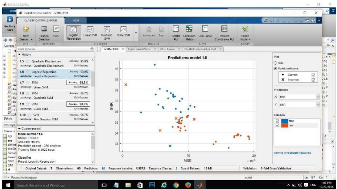
Figure C.42: Scatter plot
