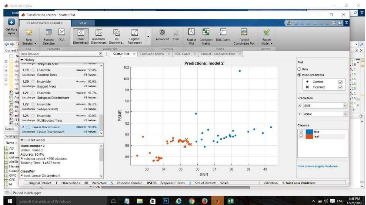
Figure C.16: Scatter plot
