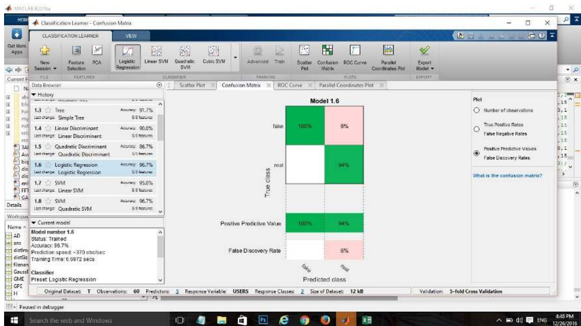
Figure C.28: Confusion matrix
