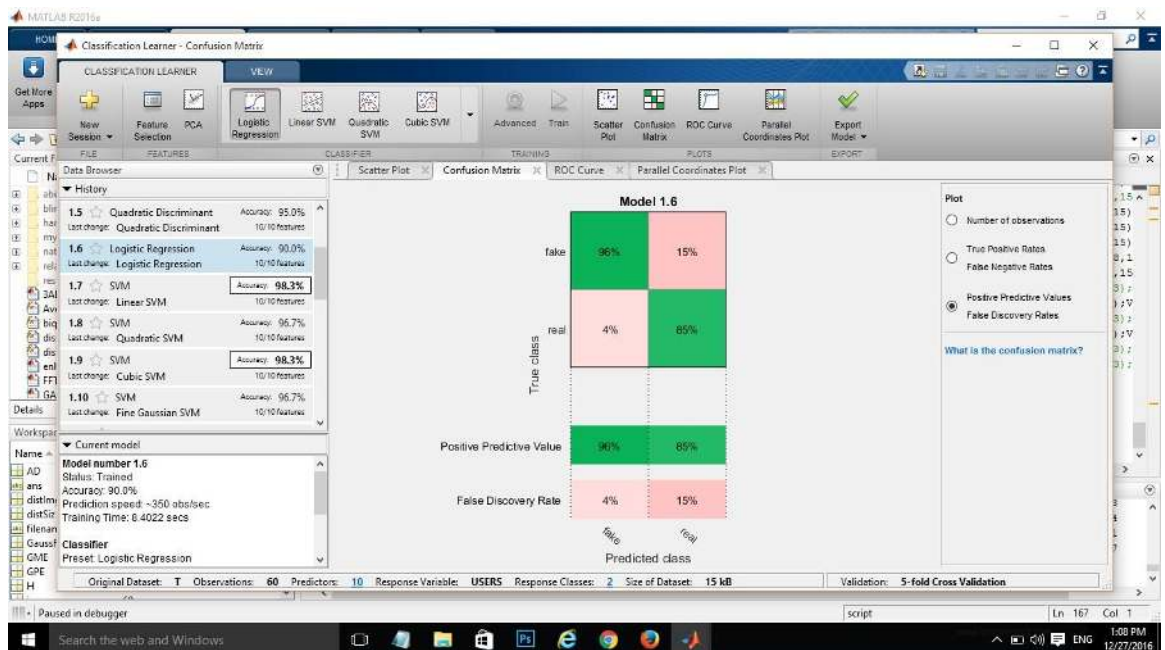
Figure C.43: Confusion matrix
