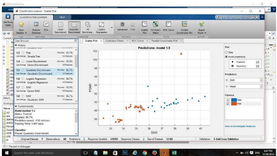
Figure C.19: Scatter plot
