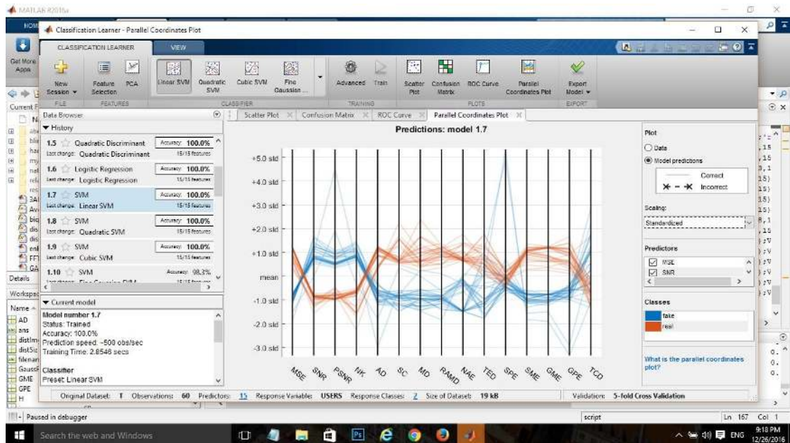
Figure C.9: Parallel coordinate
