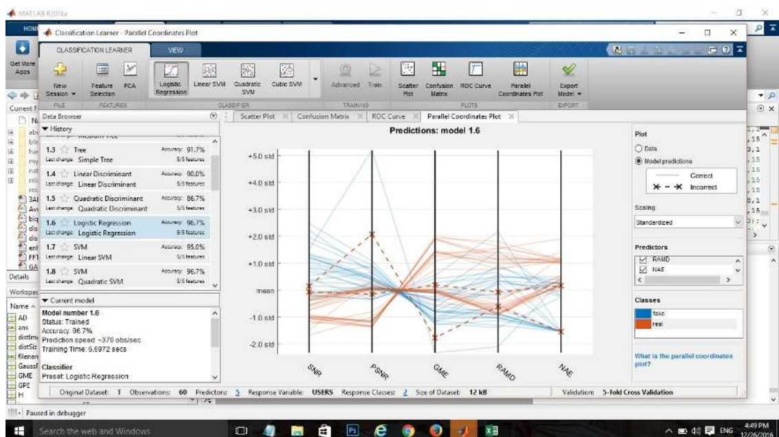
Figure C.29: Parallel coordinate
