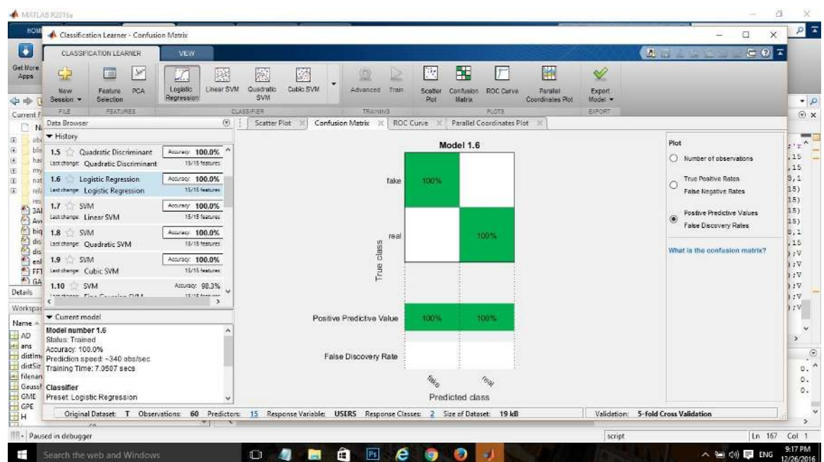
Figure C.14: Confusion matrix
