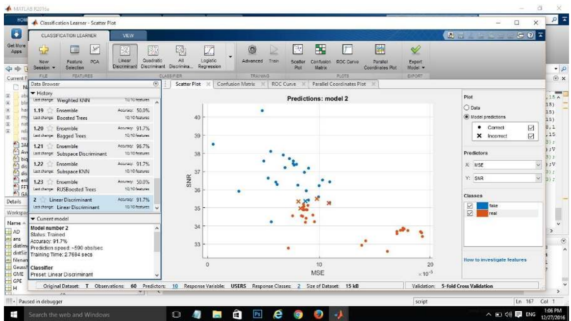
Figure C.30: Scatter plot
