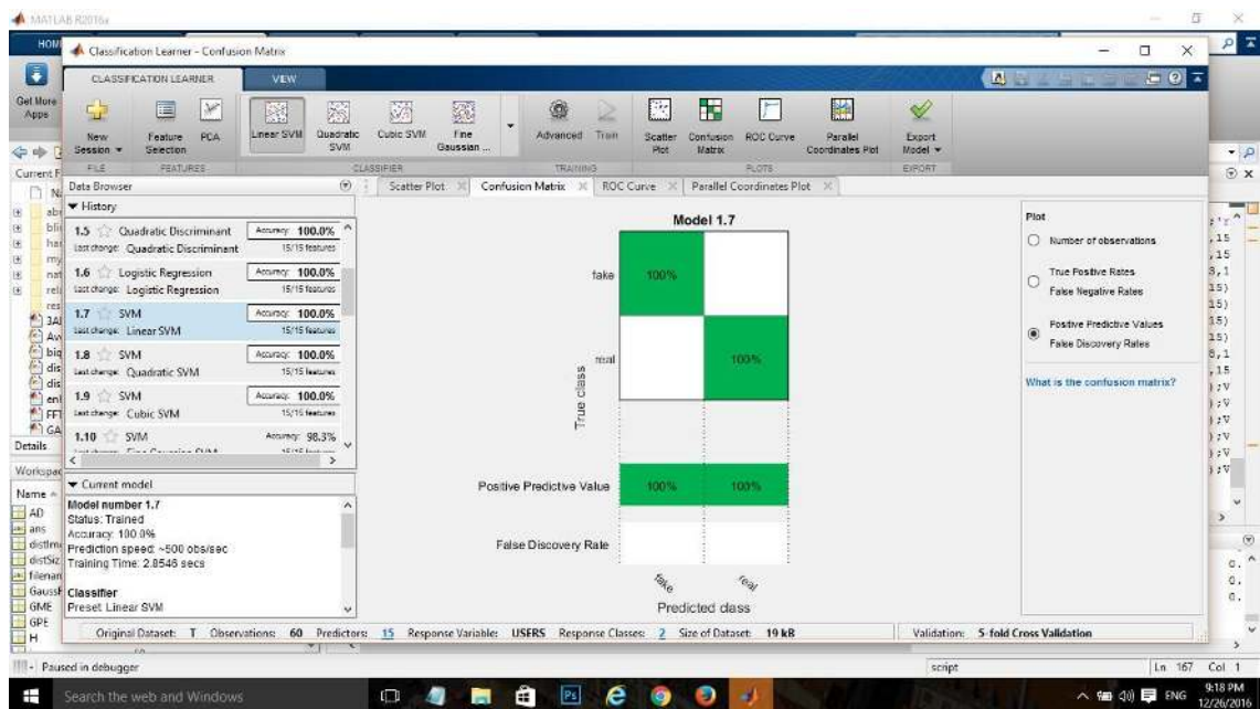
Figure C.8: Confusion matrix
