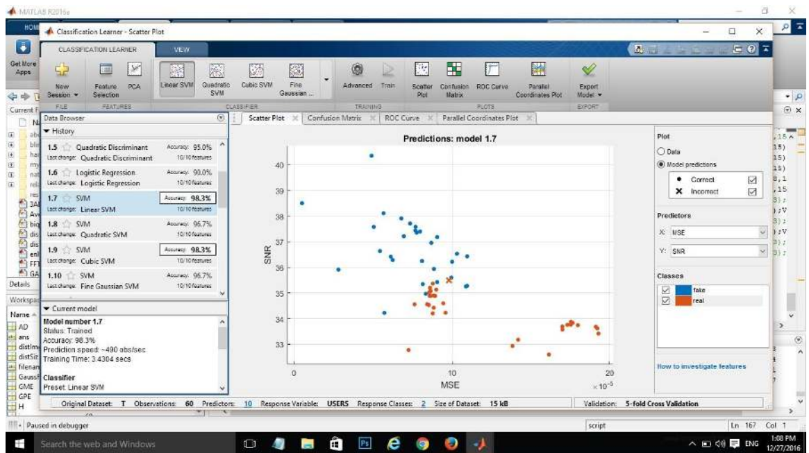
Figure C.36: Scatter plot
