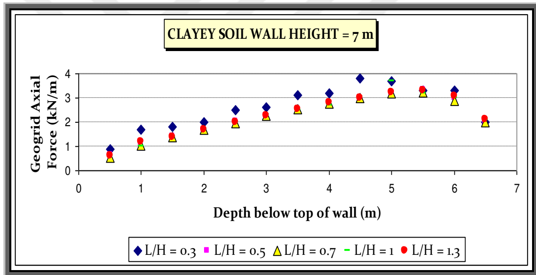
Figure 4.16 Effect of reinforcement length on geogrid axial force for (a) Loose sandy soil, (b) Dense sandy soil, (c) Clayey soil
