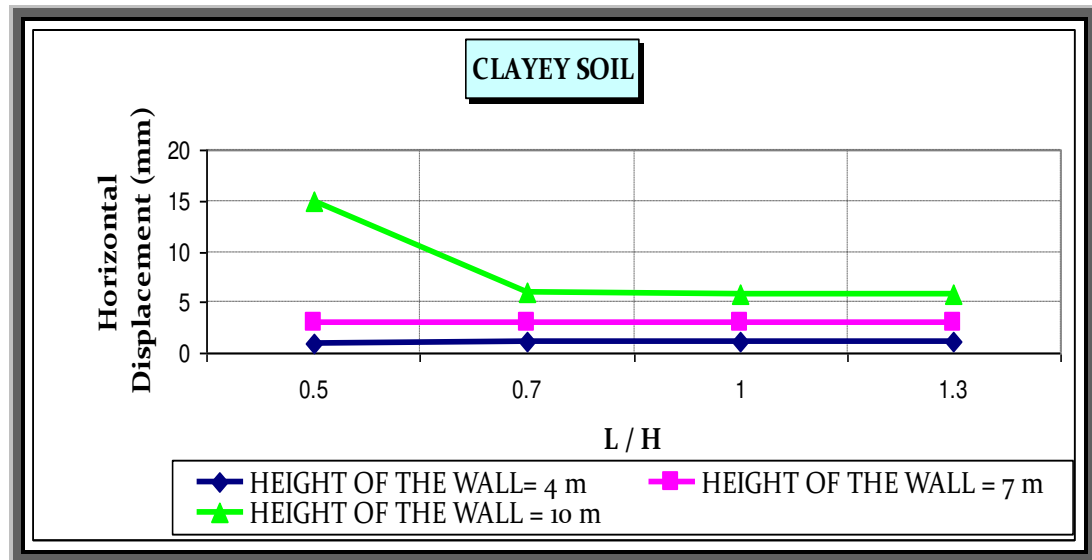
Figure 4.14 Effect of reinforcement length on horizontal displacement in (a) Loose sandy soil, (b) Dense sandy soil, (c) Clayey soil
