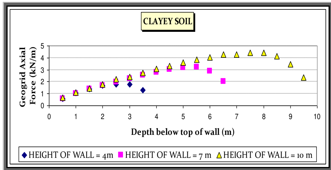
Figure 4.12 Effect of wall height on geogrid axial force in: (a) loose sandy soil, (b) Dense sandy soil, (d) clayey soil
