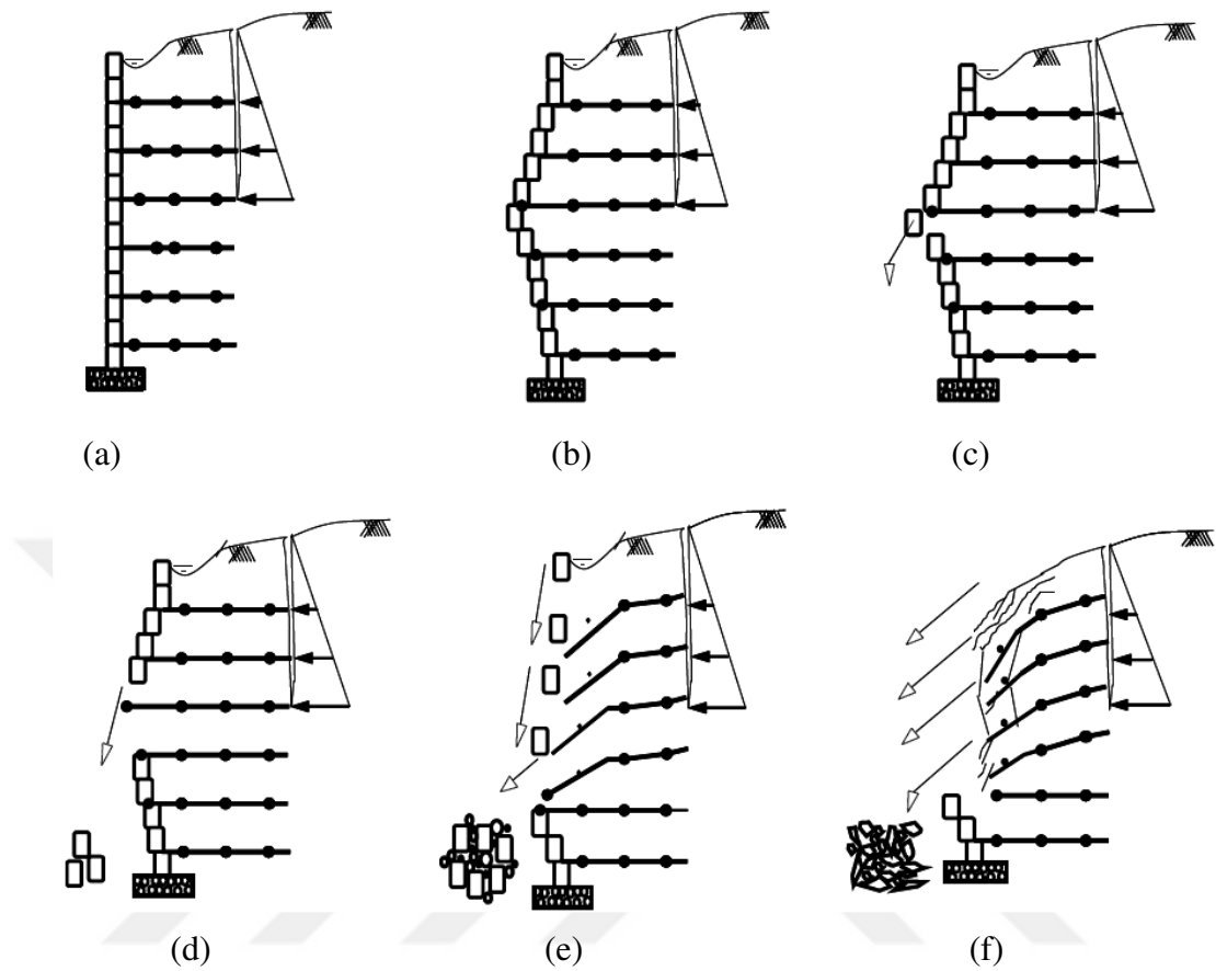
Figure 2.27 Modular block wall collapse progression due to hydrostatic pressure in tension cracks: (a) Crack forms, water enters and pressure is mobilized, (b) Wall deforms; pressure continues, (c) Deformations continuous single block dislodges and drops to toe of wall, (d) Overlying blocks drop accordingly, (e) blocks progressively drop along with gravel and some backfill soil, (f) after the wall facing collapses; majority of the MSE mass remains behind (Koerner and Koerner, 2012)
