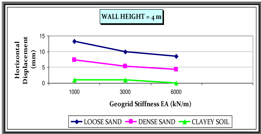
Figure 4.18 Effect of geogride stiffness and backfill soil type on horizontal displacement for: (a) H= 10 m, (b) H= 7 m, (c) H= 4 m
