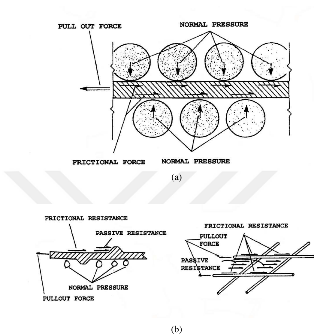
Figure 2.17 Stress transfer mechanisms for soil reinforcement: (a) frictional stress transference between soil & reinforcement surface, (b) soil passive resistance on reinforcement surface (Elise et al., 2001)
