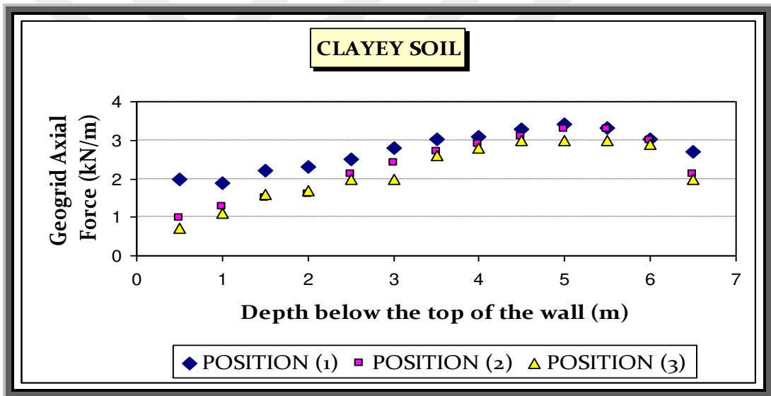
Figure 4.28 Effect traffic asurcharge load position on geogrid axial force in : (a) Loose sandy soil, (b) Dense sandy soil, (c) Clayey soil
