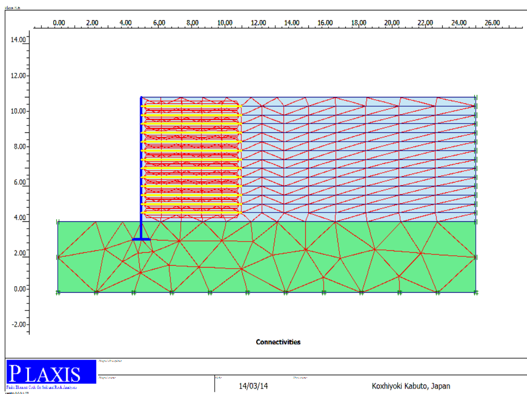
Figure 3.3 Generated Mesh at initial condition
