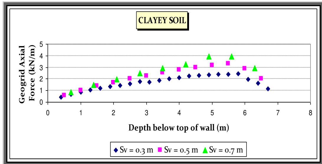
Figure 4.22 Effect of vertical spacing on geogrid axial force in: (a) Loose sandy soil, (b) Dense sandy soil, (c) Clayey soil
