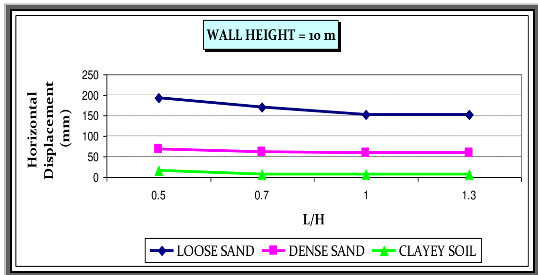
Figure 4.15 Effect of reinforcement length and type of reinforced soil on horizontal displacement for (a) H = 4 m, (b) H = 7 m, (c) H = 10 m
