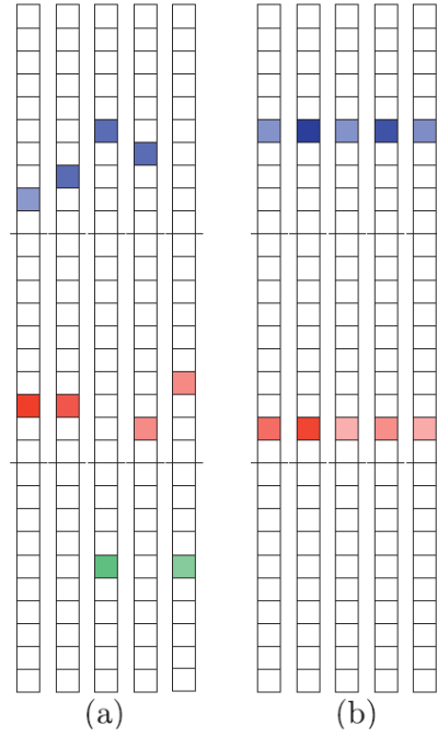
Figure 3.1: Demonstration of sparse matrix \mathbf{X} with N = 2 , L = 5 , K_1 = 10 and K_2 = 3 where white squares represent the zero coefficients and colored squares represent nonzero coefficients (a) When there is a change of value of parameters with respect to index l (b) When there is no change of value of parameters with respect to index l which shows the joint sparsity
