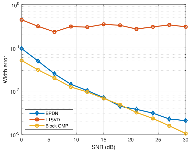
Figure 4.40: Width error for 4 well separated sources with slow evolution of delay parameter
