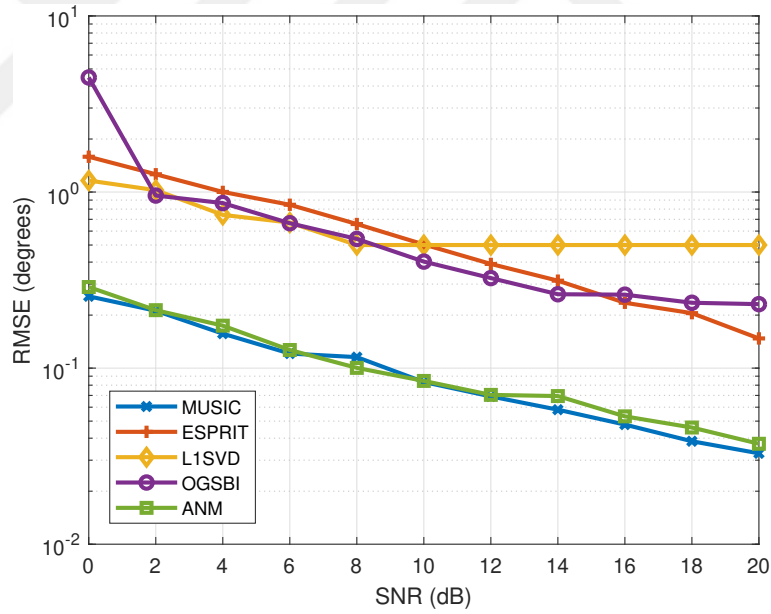
Figure 4.16: RMSE when two uncorrelated sources are well-separated and out of the grid, L = 100
