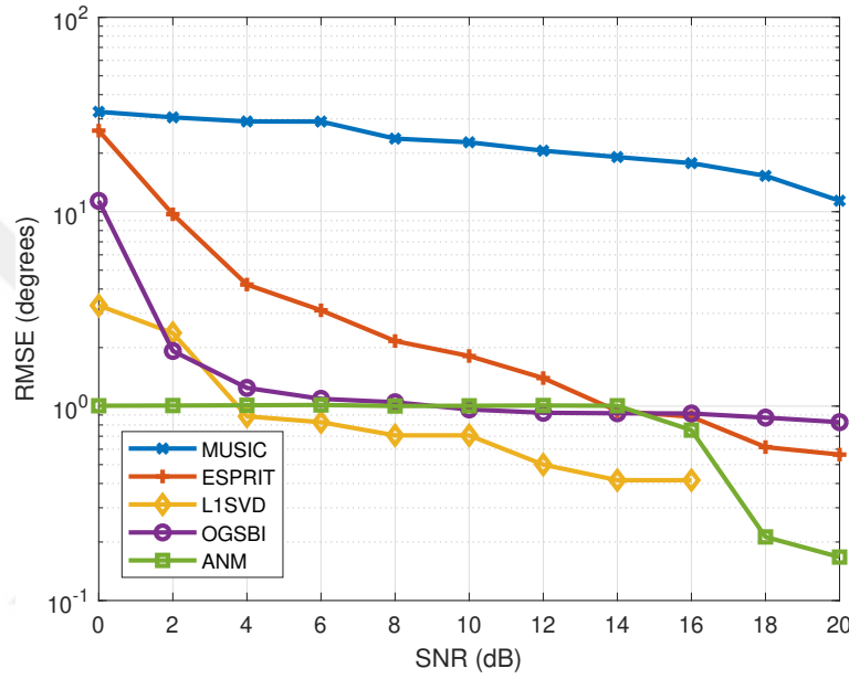
Figure 4.18: RMSE when two uncorrelated sources are closely-spaced and on the grid, L = 100
