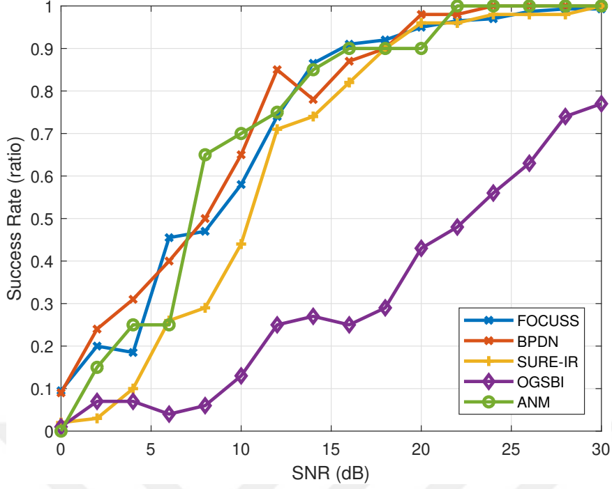
Figure 4.13: Success rate when two highly correlated sources are well-separated and out of the grid, L = 1
