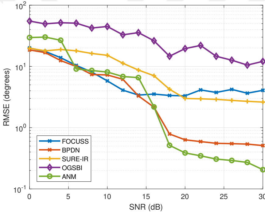
Figure 4.4: RMSE when two uncorrelated sources are well-separated and out of the grid, L = 1
