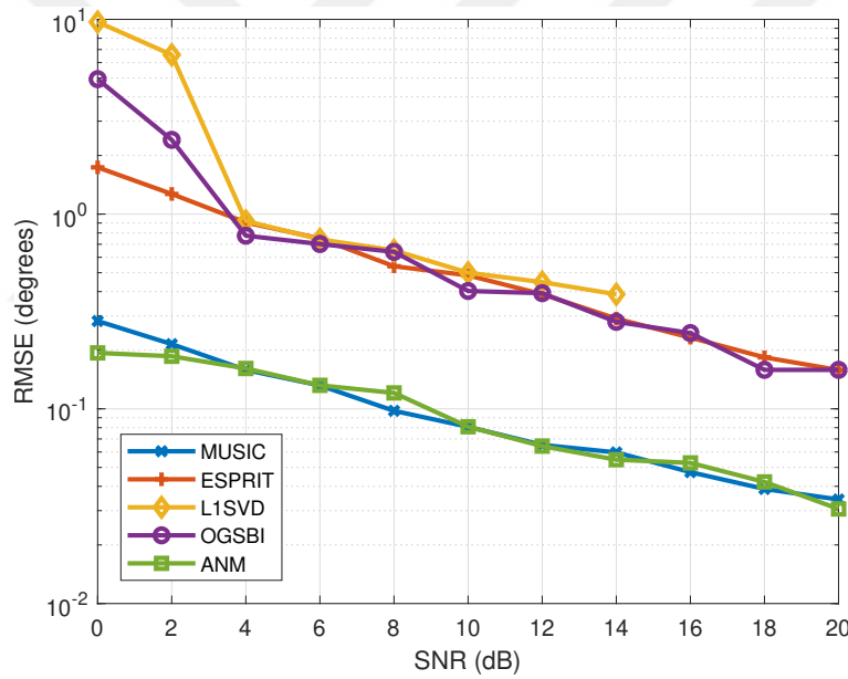
Figure 4.14: RMSE when two uncorrelated sources are well-separated and on the grid, L = 100
