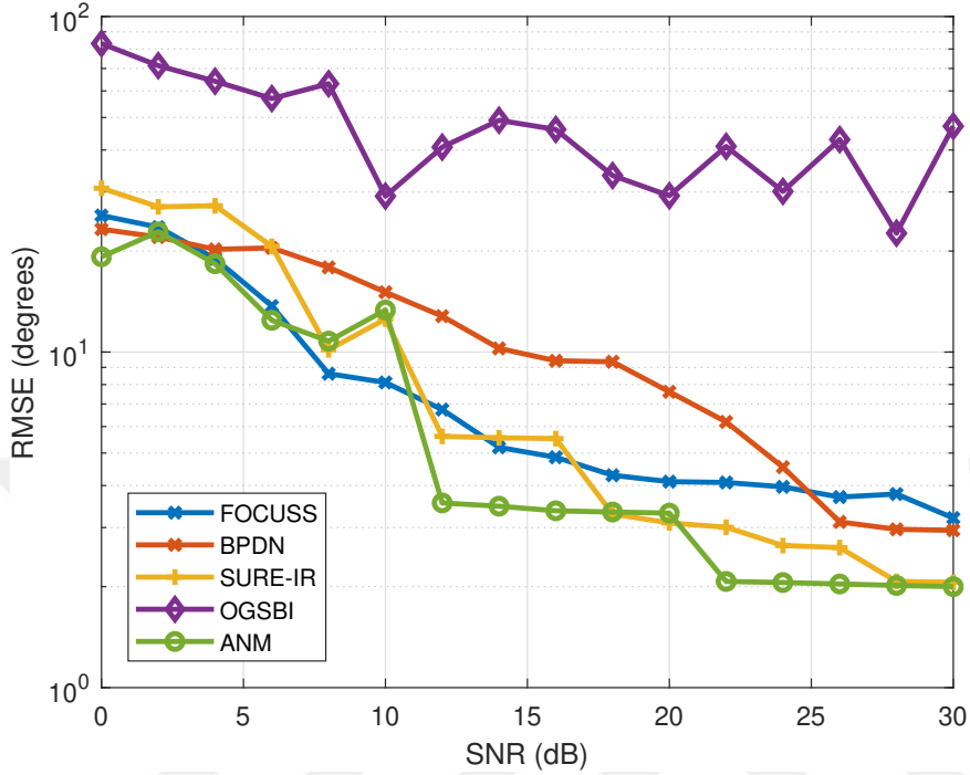
Figure 4.8: RMSE when two uncorrelated sources are closely-spaced and out of the grid, L = 1
