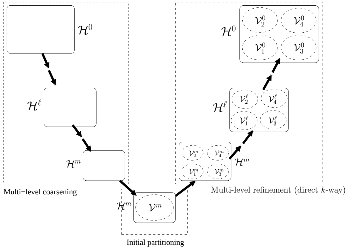
Figure 2.2: Sequential multi-level hypergraph partitioning
