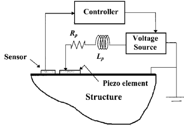
Figure 2-16 Piezoelectric Vibration absorber Suggested in [42]
