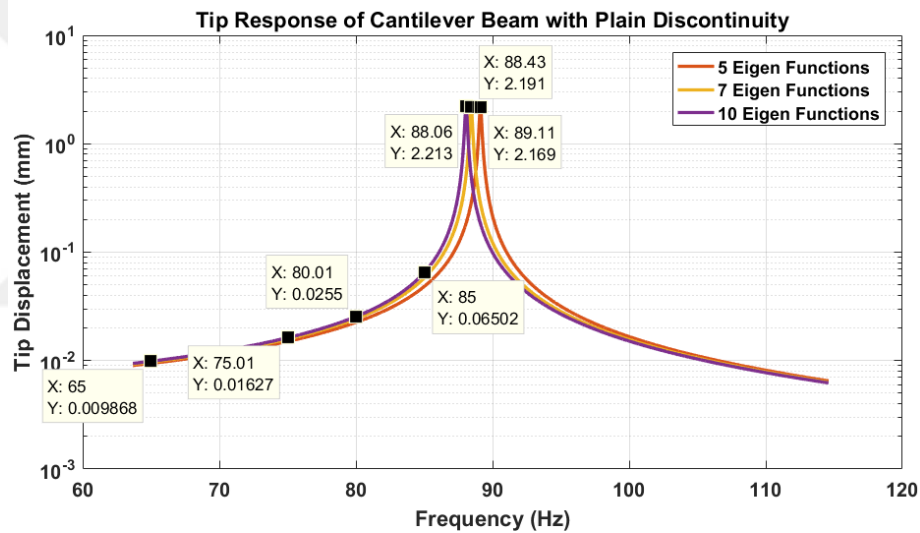
Figure 4-11 Matlab Response Tip Response of Cantilever Beam with Plain Discontinuity with Damping Constant of \gamma=2e-3
