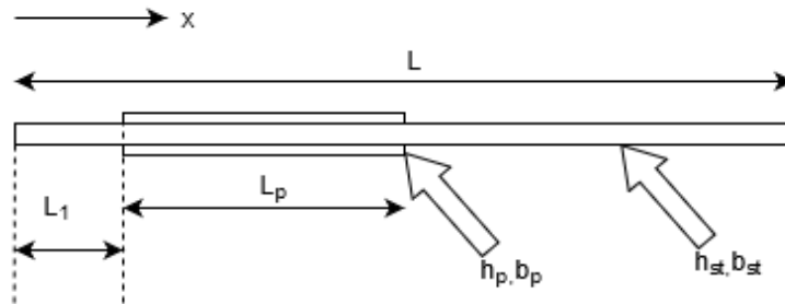
Figure 4-1 Schematic of Bimorph Composite Piezoelectric Integrated Cantilever Beam
