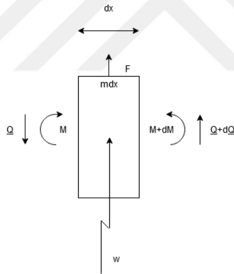
Figure 4-4 Free Body Diagram of Infinitesimal Element of Cantilever Beam Experiencing Transverse Vibration
