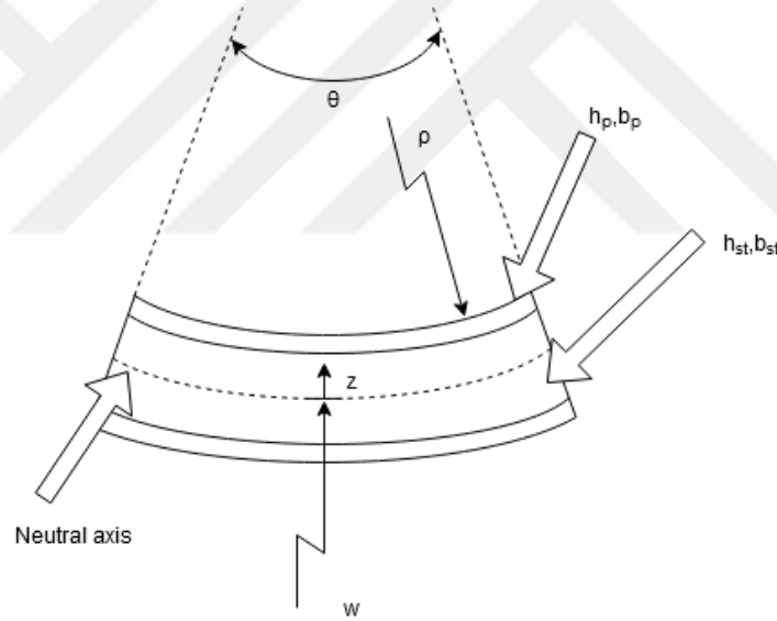
Figure 4-2 Bent Composite Beam Element
