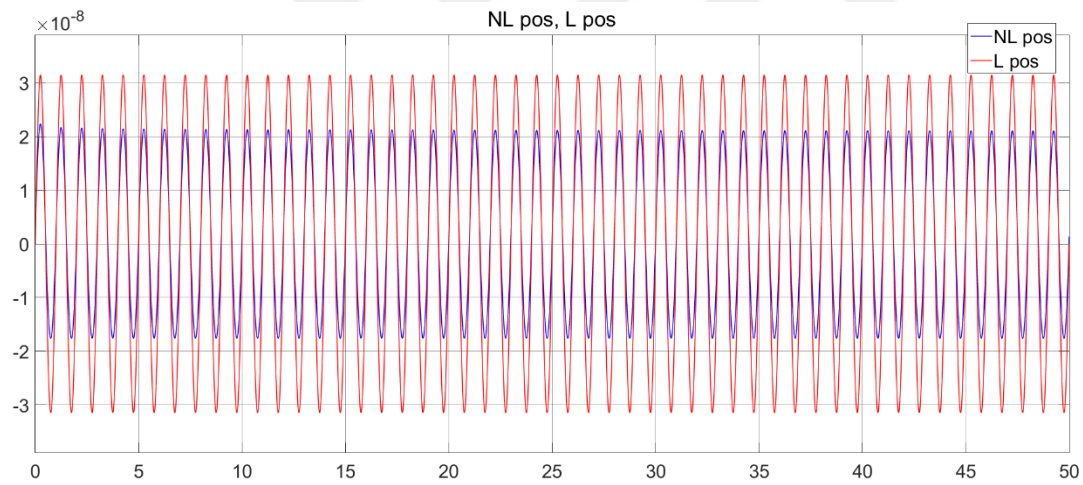
Figure 3-11 Displacement of SDOF Piezoelectric Patch under Harmonic Forcing in Simulink; Nonlinear Shunt (Blue), Linear Shunt (Red)
