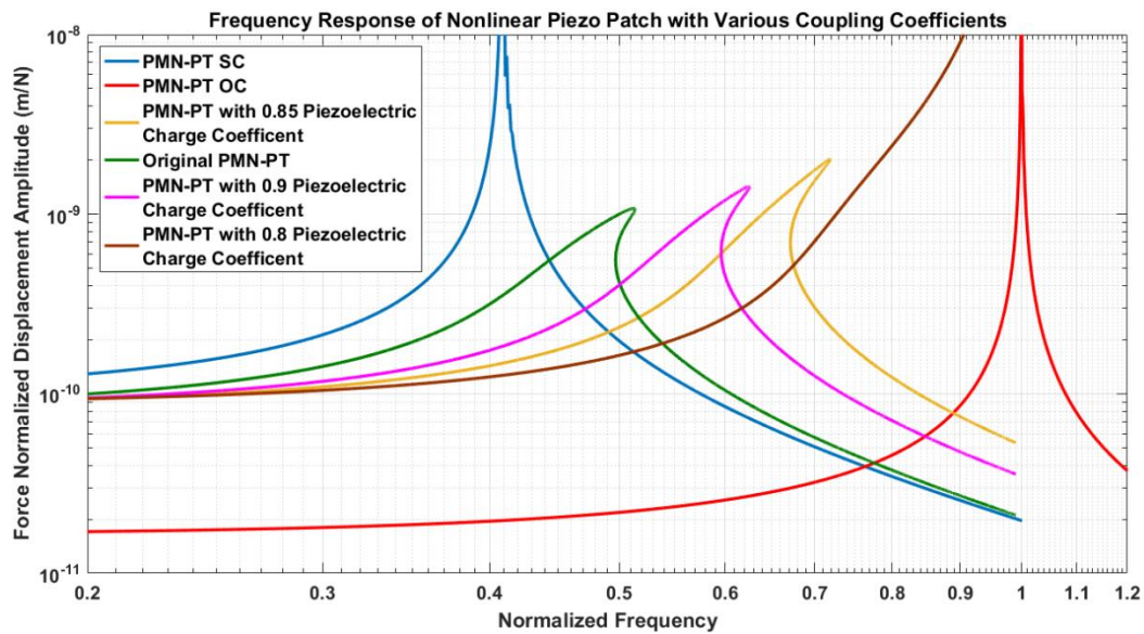
Figure 3-19 Displacement Frequency Response of Original and Weakened Piezoelectric Patches with Open Circuit, Short Circuit, and Nonlinear Circuit
