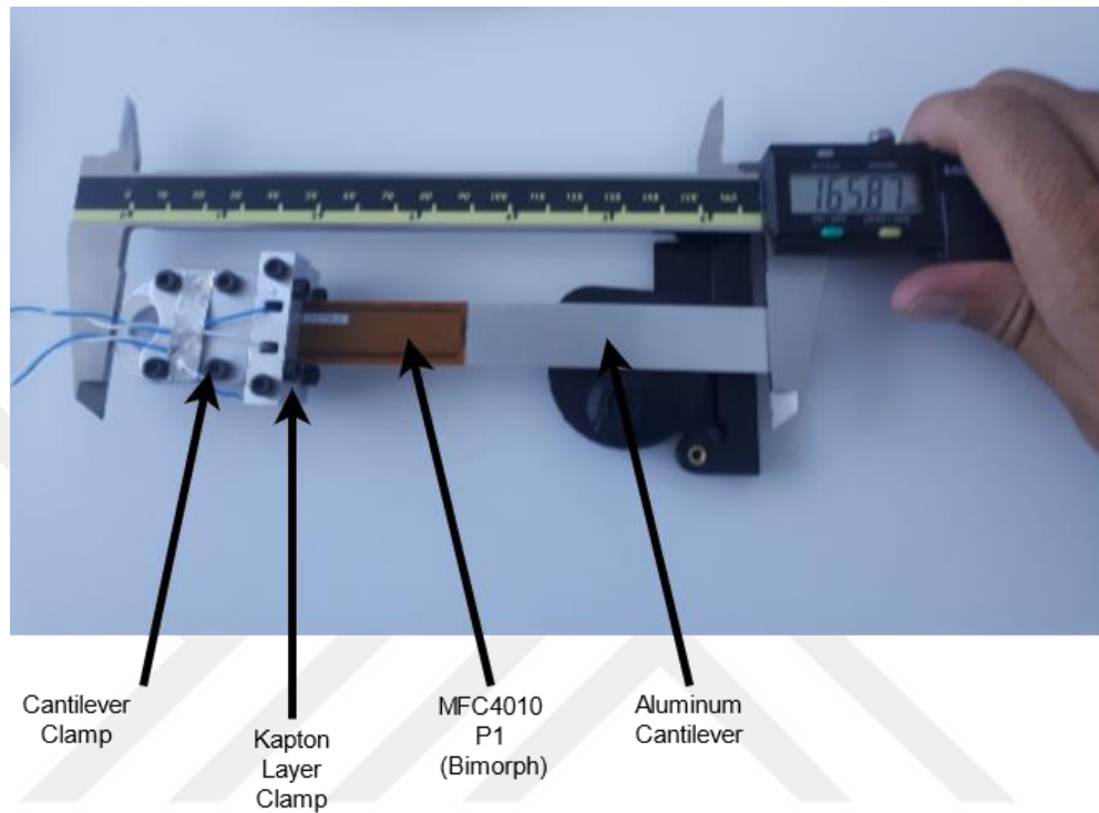
Figure 5-2 Cantilever Beam Assembly with Total Length
