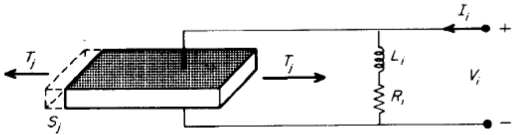
Figure 2-4 RL Shunt Circuit [17]
