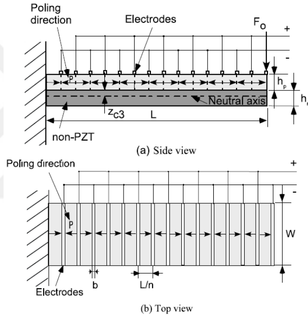
Figure 4-7 Piezoelectric Patch with Interdigitated Electrodes Integrated to Unimorph Cantilever Beam [73]
