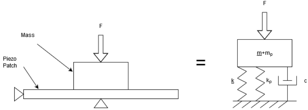
Figure 3-17 Equivalent Model of Piezoelectric Patch system with Mass under Harmonic Loading
