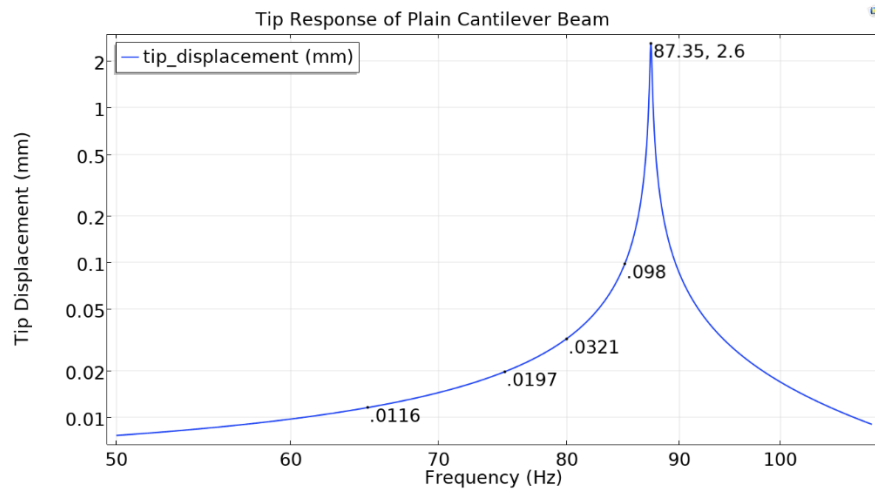
Figure 4-12 FEM Result for Tip Response of Cantilever Beam with Plain Discontinuity with Damping Constant of \gamma=2e-3
