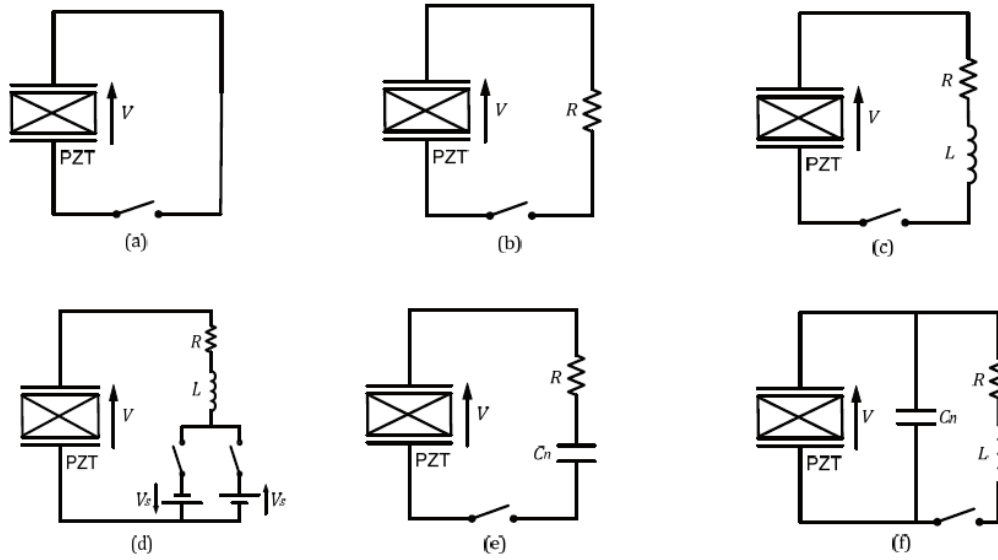
Figure 2-11 Switching Shunt Circuits [15]; (a) State Switch (b) Switch on Resistor (c) Switch on Inductor (d) Switch on Voltage (e) Switch on Negative Capacitor (f) Switch on Negative Capacitance and Inductor
