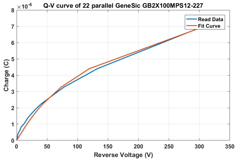
Figure 4-20 Read Data and Fit Curve for 22 Parallel Connected GeneSic GB2X100MPS12-227
