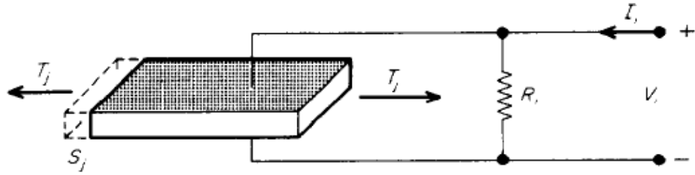
Figure 2-3 R Shunt Circuit [17]
