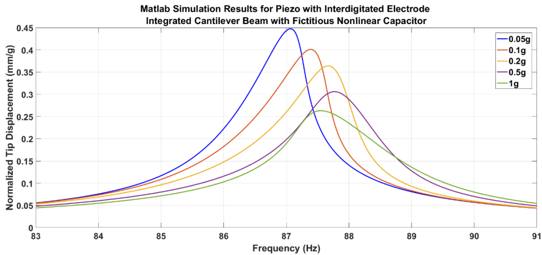
Figure 4-27 Matlab Result for Piezoelectric Patch with Interdigitated Electrodes Integrated Cantilever Beam under Fictitious Nonlinear Capacitor Shunt Circuit Condition
