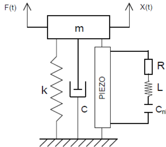
Figure 2-8 SDOF Nonlinear Shunt Circuit Introduced by Zhou et al. [24]
