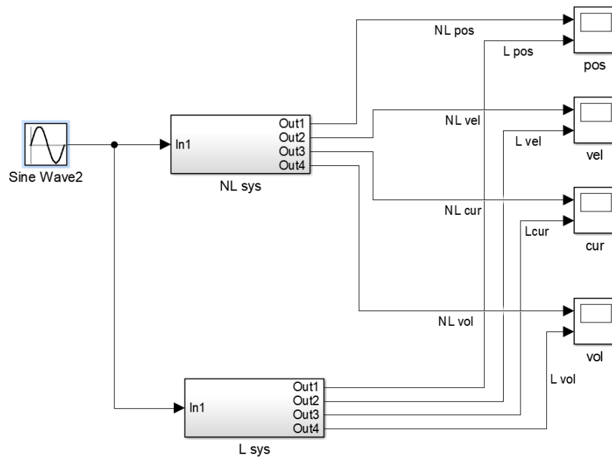
Figure 3-8 Simulink Model of SDOF Piezoelectric Patch under Harmonic Forcing
