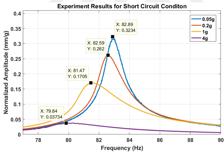
Figure 5-12 Short Circuit Condition Experiment Frequency Response Results
