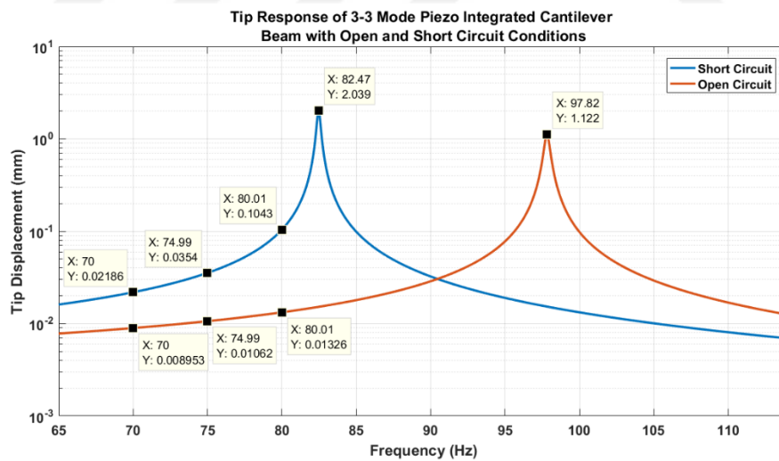
Figure 4-17 Matlab Results for Tip Response of 3-3 Mode Piezoelectric Material Integrated Cantilever Beam with Open and Short Circuit Conditions
