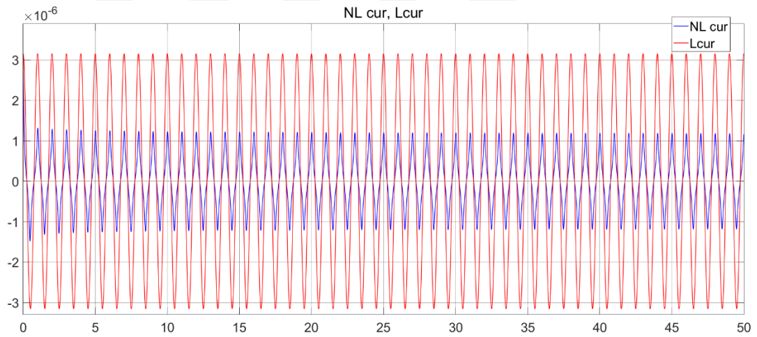
Figure 3-13 Current of SDOF Piezoelectric Patch under Harmonic Forcing in Simulink; Nonlinear Shunt (Blue), Linear Shunt (Red)
