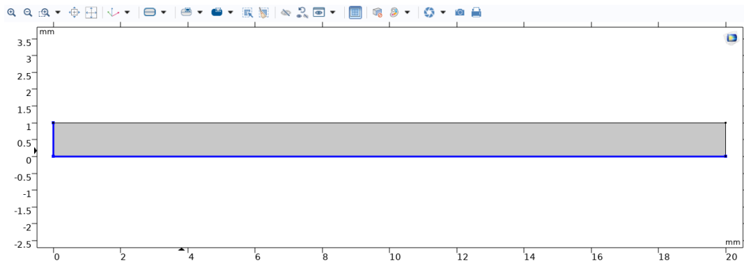
Figure 3-5 Roller Boundary Regions in Comsol For Quasi Static Loaded Piezoelectric Patch Analysis
