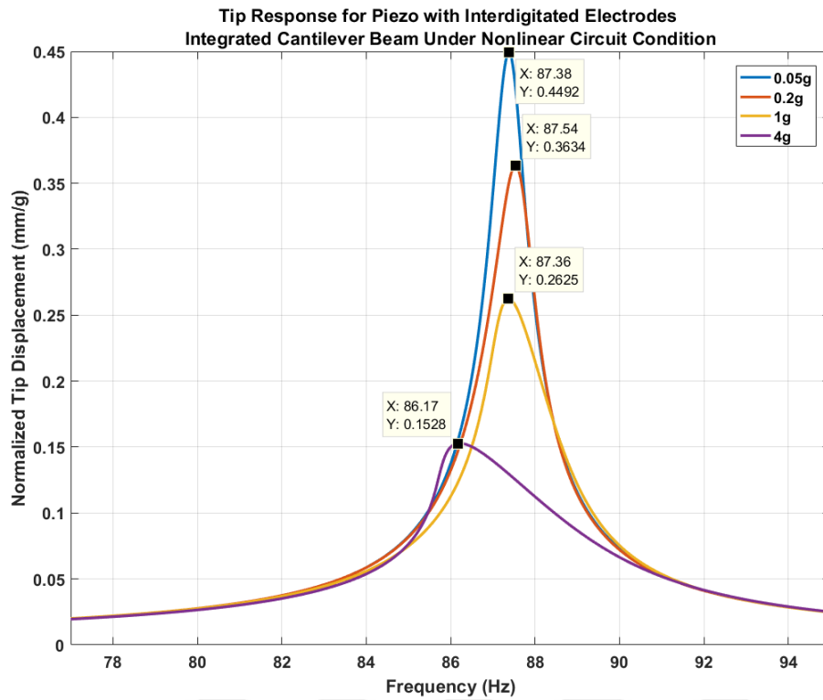
Figure 4-25 Matlab Result for Piezoelectric Patch with Interdigitated Electrodes Integrated Cantilever Beam under Nonlinear Capacitor Shunt Circuit Condition
