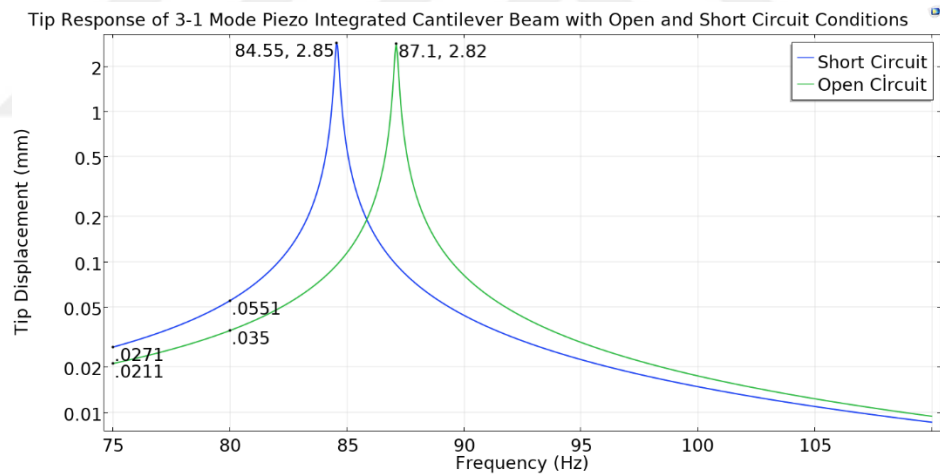
Figure 4-16 FEM Result for Tip Response of 3-1 Mode Piezoelectric Material Integrated Cantilever Beam with Open and Short Circuit Conditions
