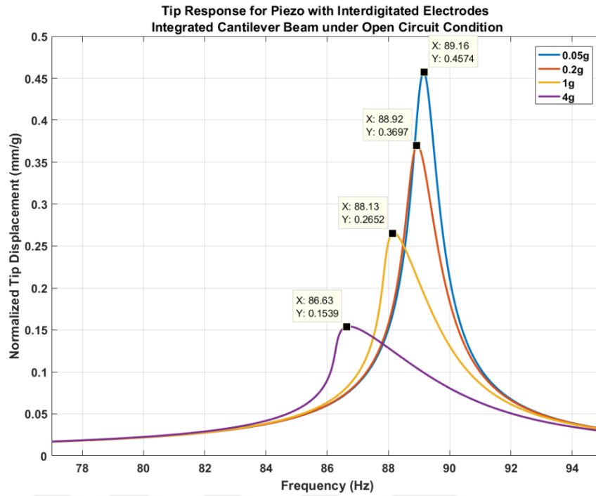
Figure 4-24 Matlab Result for Piezoelectric Patch with Interdigitated Electrodes Integrated Cantilever Beam under Open Circuit Condition
