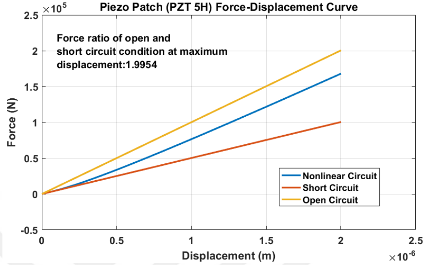
Figure 3-3 Force vs. Displacement Curve for PZT-5H piezoelectric patch with cubic curve fit to 10000 number of parallel connected Toko KV1471
