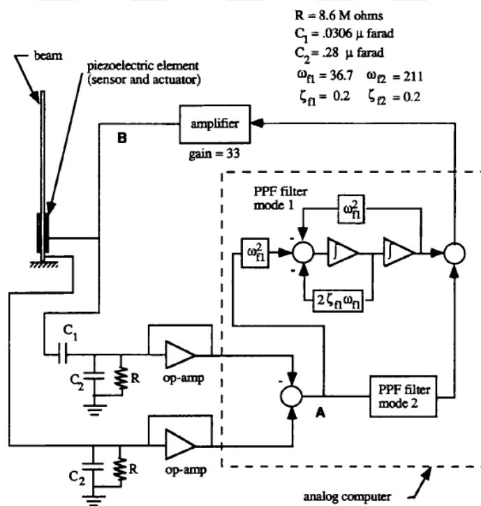
Figure 2-20 Self Sensing Position Feedback Sensor/Actuator System in [46]
