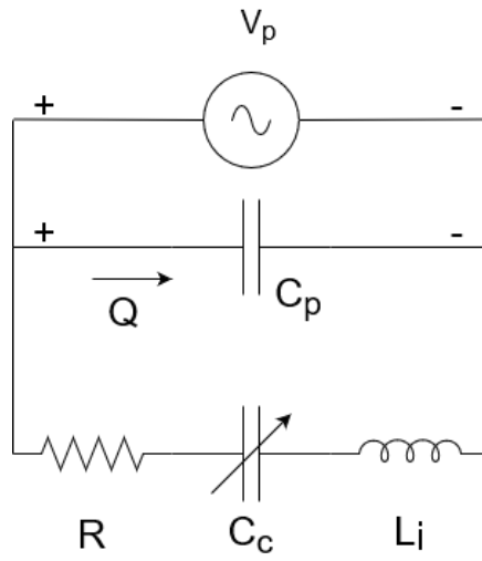
Figure 4-3 Piezoelectric Shunt circuit
