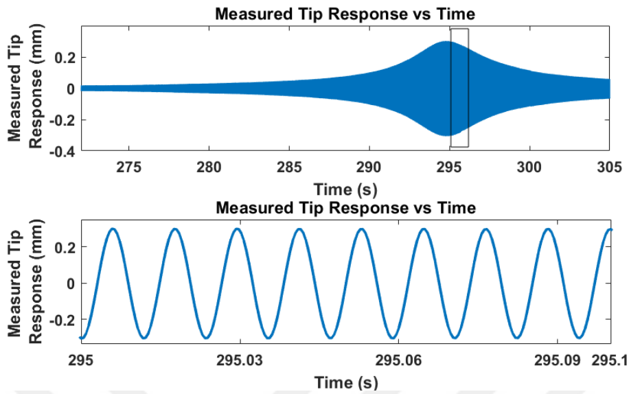
Figure 5-9 Sample Time Domain Data of Nonlinear Shunt Circuit condition Excited at 0.2g
