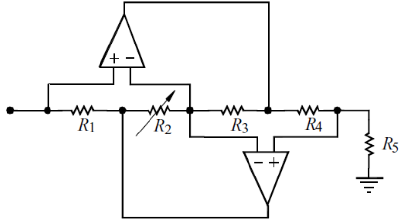
Figure 2-15 Synthetic Inductor in [20]
