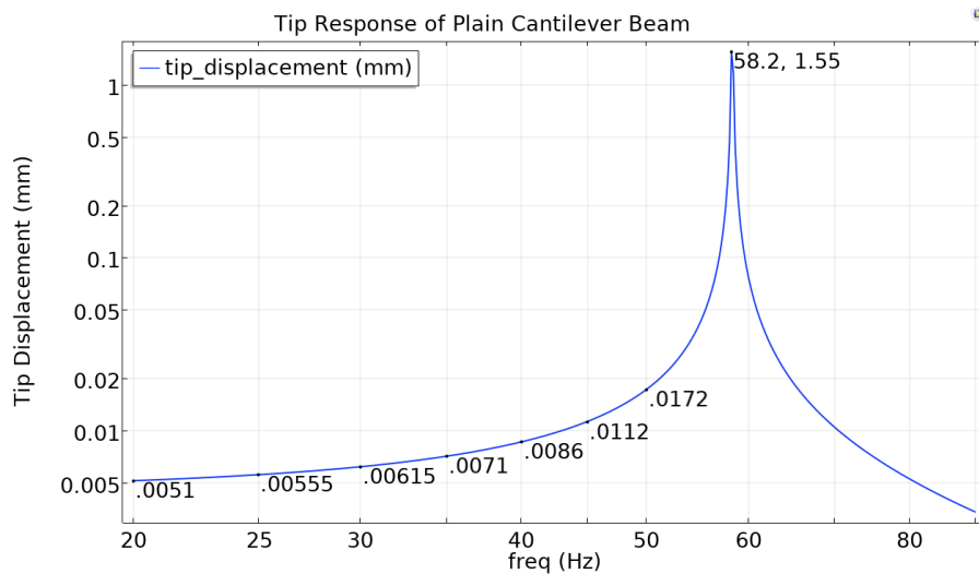
Figure 4-10 FEM Result for Tip Response of Plain Cantilever Beam
