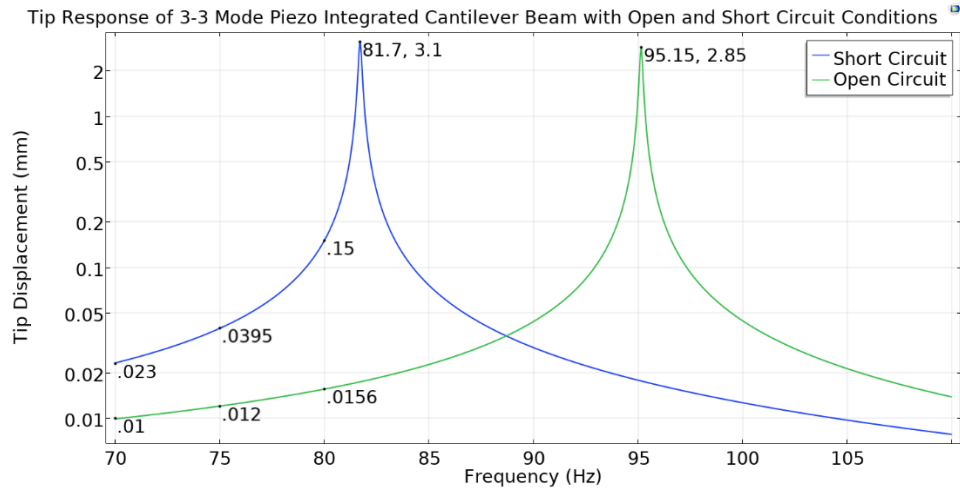
Figure 4-18 FEM Result for Tip Response of 3-3 Mode Piezoelectric Patch Integrated Cantilever Beam with Open and Short Circuit Conditions
