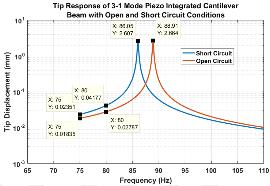
Figure 4-15 Matlab Result for Tip Response of 3-1 Mode Piezoelectric Material Integrated Cantilever Beam with Open and Short Circuit Conditions
