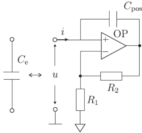
Figure 2-14 Negative Capacitance Offered by Han et al. [39]
