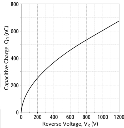
Figure 4-19 Q-V Curve of GeneSic GB2X100MPS12-227 [78]
