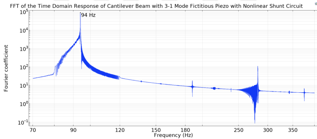
Figure 4-23 FFT of the Time Domain Response of Cantilever Beam with 3-1 Mode Fictitious Piezoelectric Patch with Nonlinear Shunt Circuit
