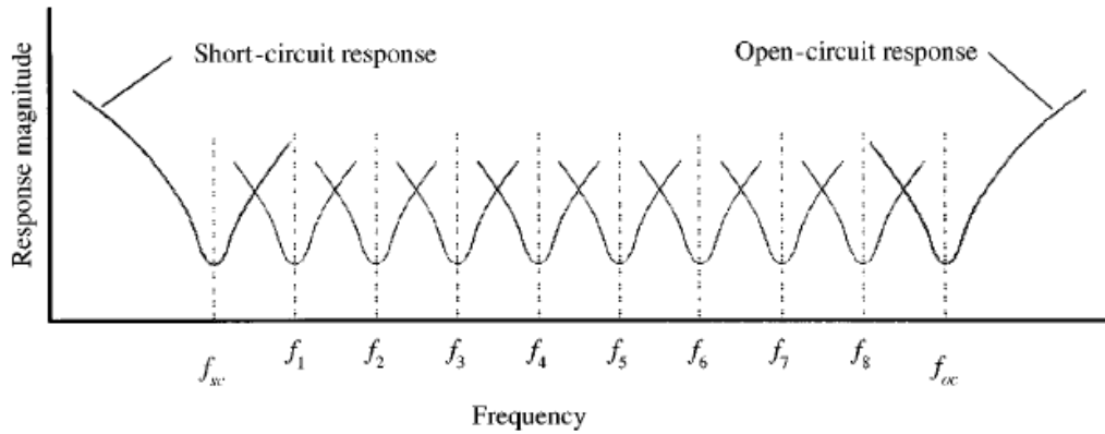
Figure 2-13 Response of the Piezoelectric Shunt System for Open Circuit and Short Circuit and Intermediate Tuned Capacitive Shunt [34]
