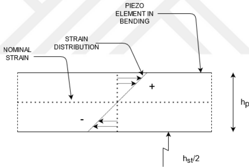
Figure 4-6 Piezoelectric Element on Bimorph Cantilever Beam. h_{st}/2 is Distance from Neutral Axis and h_p is Height of the Piezoelectric Patch
