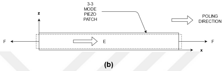
Figure 4-5 Piezoelectric Patch Poled in the z-direction (a) and in the x-direction (b)
