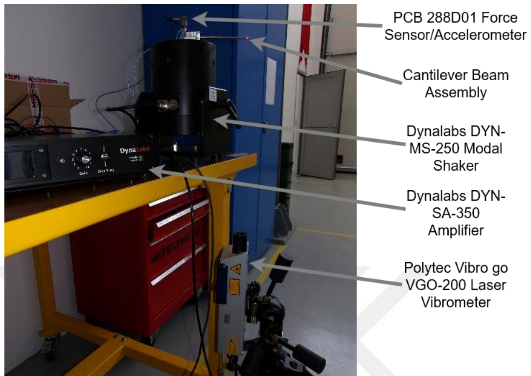
Figure 5-8 Test Setup
