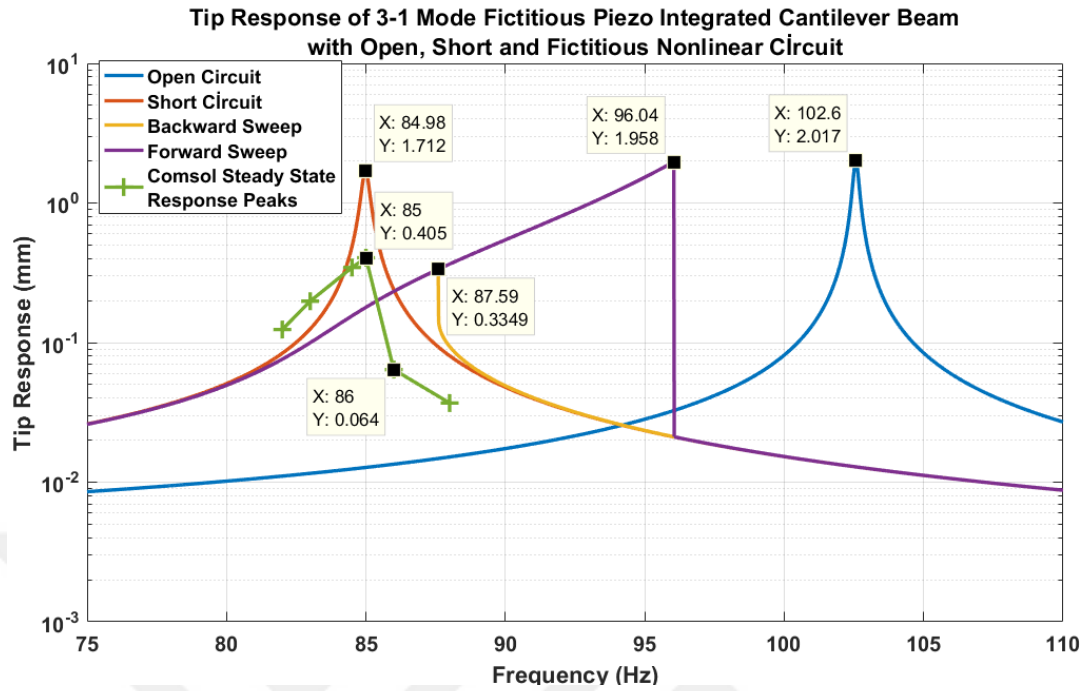
Figure 4-21 Matlab Results for Tip Response of 3-1 Mode Fictitious Piezoelectric Patch Integrated Cantilever Beam and Comsol Steady State Simulation Results for Low Frequency Jump
