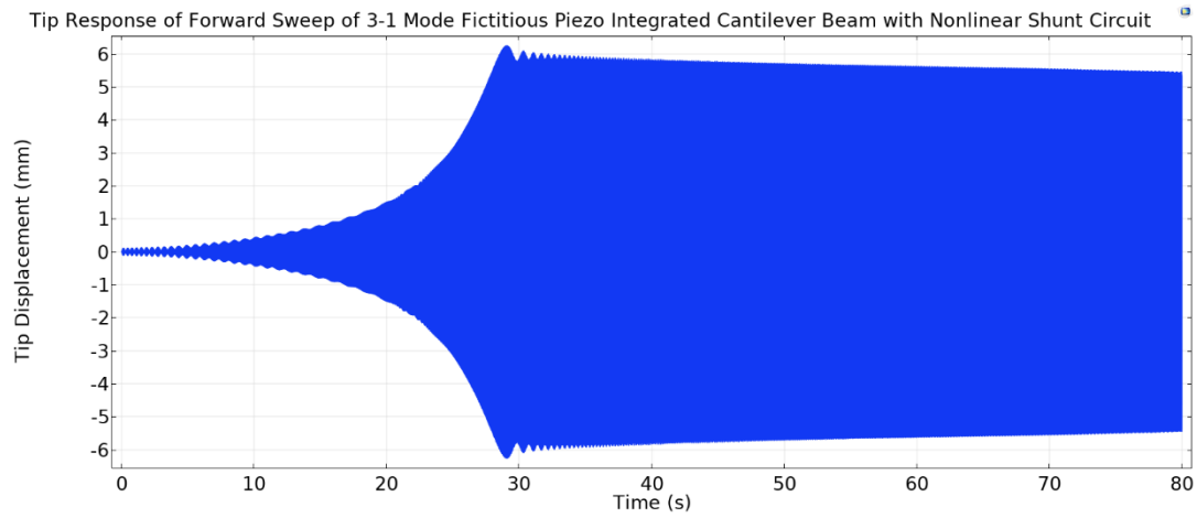
Figure 4-22 Time Domain Simulation of Forward Sweep of 3-1 Mode Fictitious Piezoelectric Patch Integrated Cantilever Beam with Nonlinear Shunt Circuit
