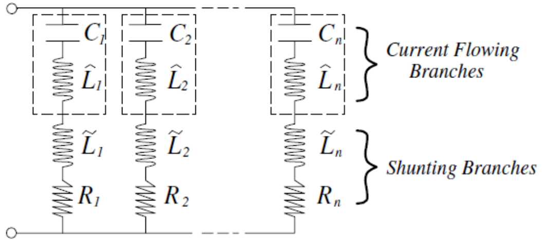
Figure 2-7 An Example of Multi Mode Vibration Absorber Shunt Circuit
