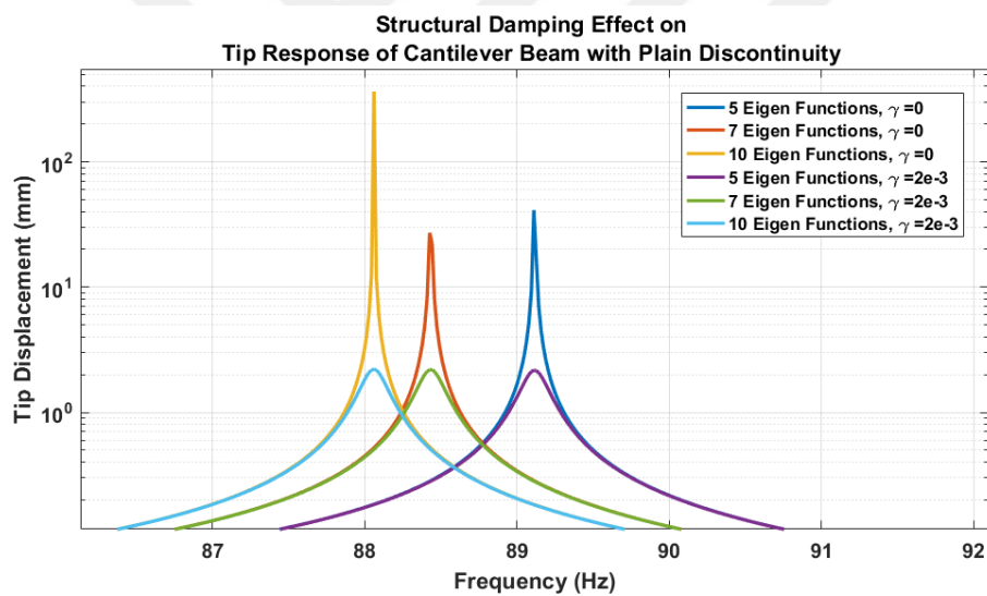
Figure 4-13 Damped and Undamped Response Comparison of Calculated Tip Response of Cantilever Beam with Plain Discontinuity
