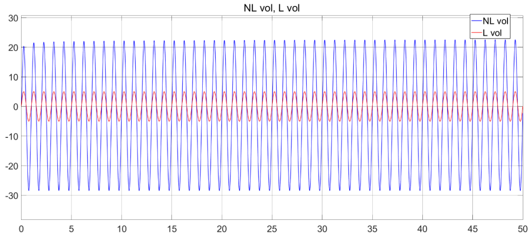
Figure 3-12 Terminal Voltage of SDOF Piezoelectric Patch under Harmonic Forcing in Simulink; Nonlinear Shunt (Blue), Linear Shunt (Red)
