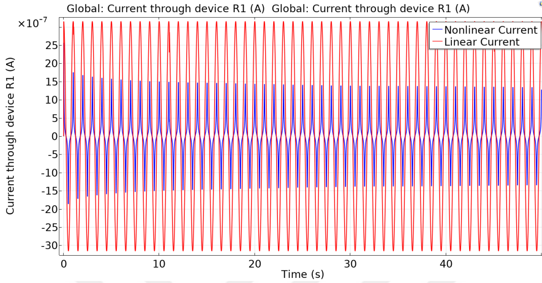
Figure 3-16 Current of SDOF Piezoelectric Patch under Harmonic Forcing in Comsol 5.4; Nonlinear Shunt (Blue), Linear Shunt (Red)
