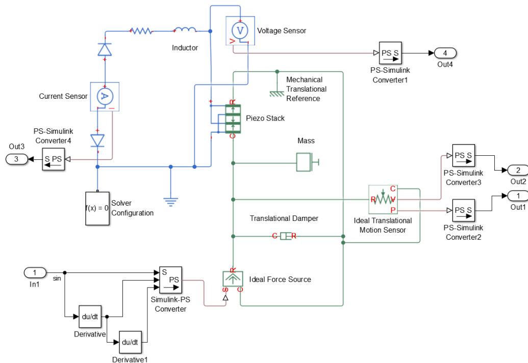
Figure 3-9 Nonlinear System Block in Figure 3-8
