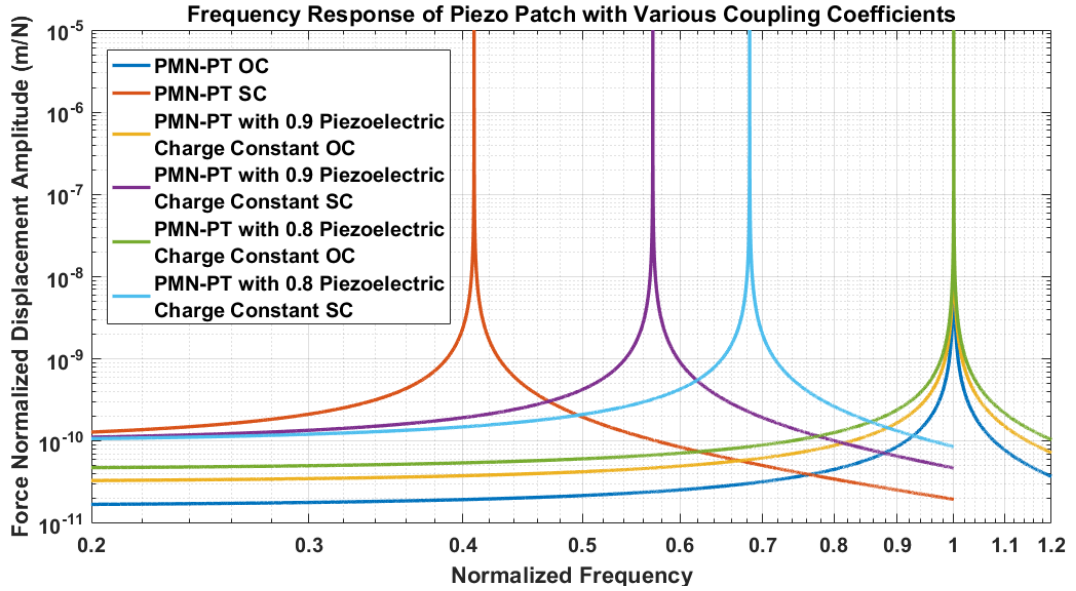
Figure 3-18 Displacement Frequency Response of Original and Weakened Charge Constant Piezoelectric Patches for Open and Short Circuit Conditions Only
