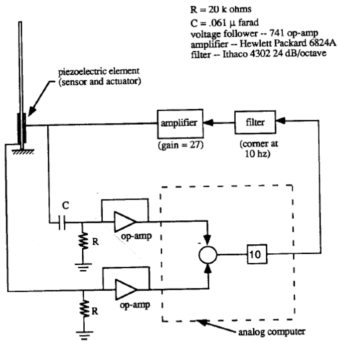
Figure 2-19 Self Sensing Rate Feedback Sensor/Actuator System in [46]
