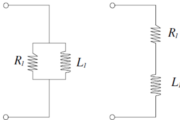
Figure 2-6 Single Mode Vibration Isolation Shunt Circuit [21]
