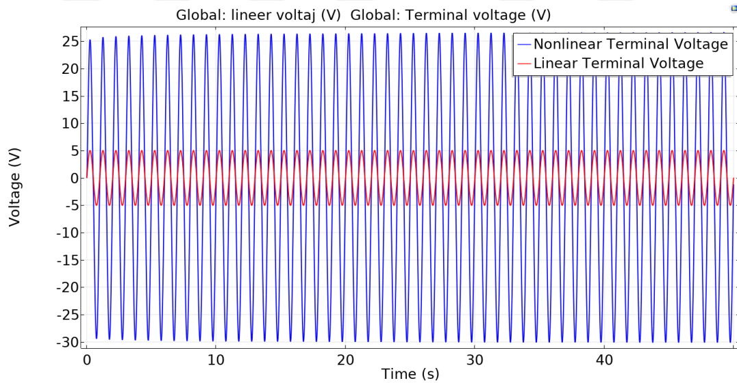
Figure 3-15 Terminal Voltage of SDOF Piezoelectric Patch under Harmonic Forcing in Comsol 5.4; Nonlinear Shunt (Blue), Linear Shunt (Red)
