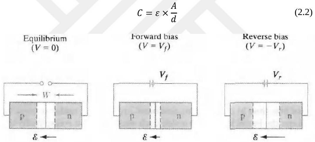
Figure 2-2 P-N Junction Biasing and Junction Reaction [12]
