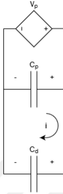
Figure 3-2 Circuit Diagram of Capacitance C_d Connected to Terminals of Piezoelectric Patch
