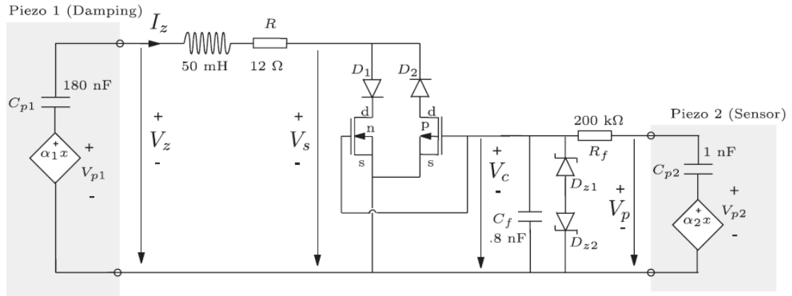
Figure 2-10 Nonlinear Shunt Circuit Introduced by Niederberger et al. [27]
