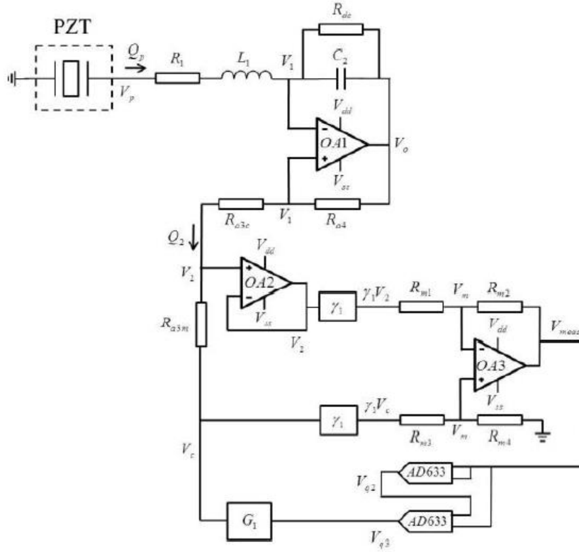
Figure 2-21 Nonlinear Piezoelectric Shunt Circuit Studied in [50]
