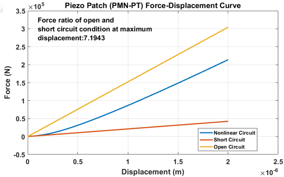
Figure 3-4 Force vs. Displacement Curve for PMN-PT single crystal piezoelectric patch with cubic curve fit to 10000 number of parallel connected Toko KV1471
