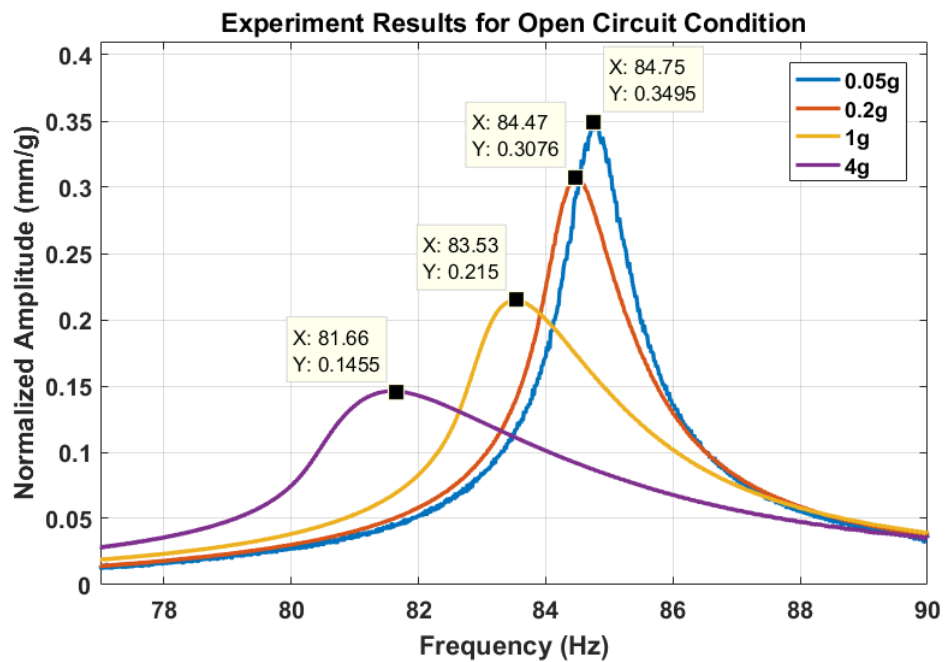
Figure 5-10 Open Circuit Condition Experiment Frequency Response Results
