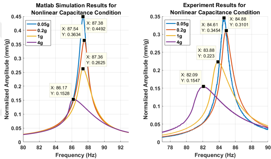
Figure 5-13 Comparison of Matlab Simulation Results and Experiment Results for Nonlinear Capacitance Condition
