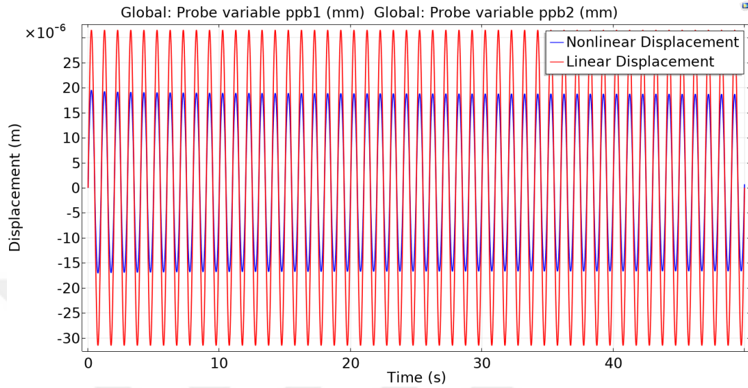
Figure 3-14 Displacement of SDOF Piezoelectric Patch under Harmonic Forcing in Comsol 5.4; Nonlinear Shunt (Blue), Linear Shunt (Red)
