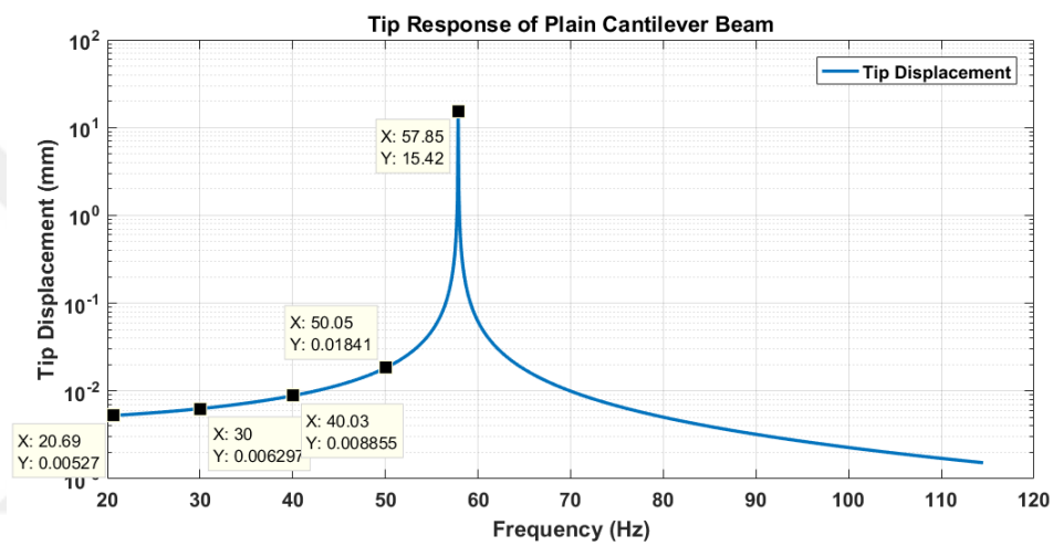
Figure 4-9 Matlab Result for Tip Response of Plain Cantilever Beam
