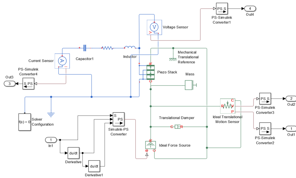
Figure 3-10 Linear System Block in Figure 3-8
