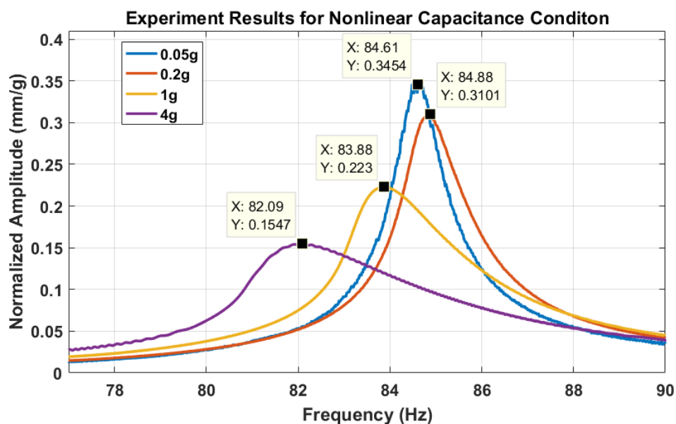
Figure 5-11 Nonlinear Capacitor Circuit Condition Experiment Frequency Response Results
