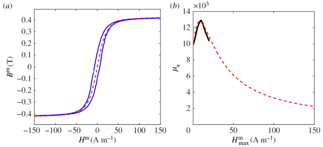
Figure 2-9 Saturating Inductor Material Data Used in [26]: (a) Magnetic Field vs. Magnetic Field Intensity of the Material (blue line) Polynomial Approximation (red line) (b) Relative Magnetic Permeability vs. Magnetic Field Intensity of the Material (black line) Polynomial Approximation (red line)
