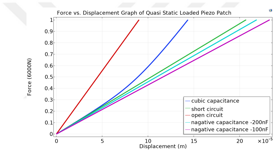
Figure 3-7 Force vs. Displacement Graph of Quasi Static Loaded Piezoelectric Patch with 5 Different Shunt Circuits; Open Circuit, Short Circuit, Nonlinear Capacitor, and Two Negative Capacitance Capacitors
