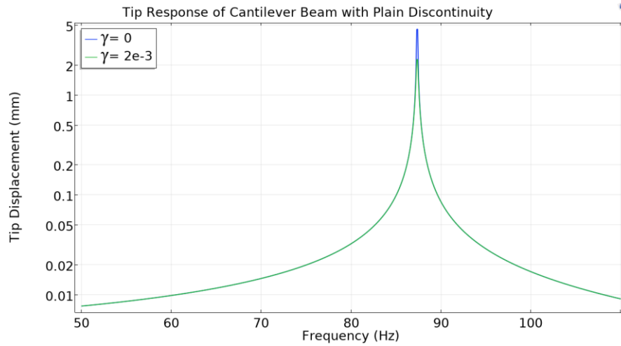
Figure 4-14 Damped and Undamped FEM Response Comparison of Tip Response of Cantilever Beam with Plain Discontinuity
