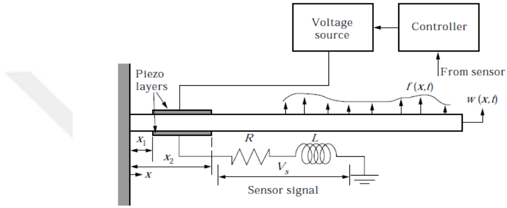
Figure 2-18 Active Passive Piezoelectric Vibration Absorber System in [45]
