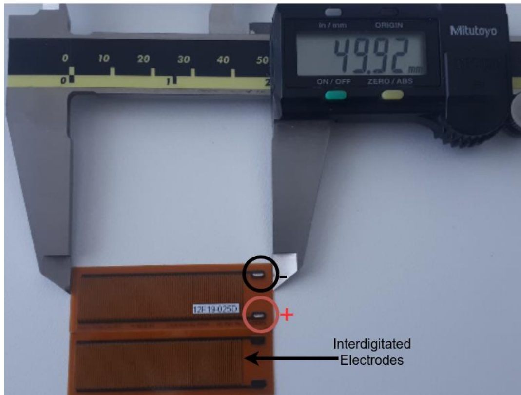
Figure 5-1 MFC4010 P1
