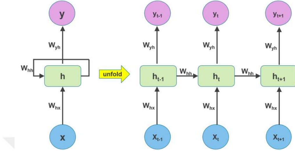
Figure 2.4: Structure of an RNN [59].
