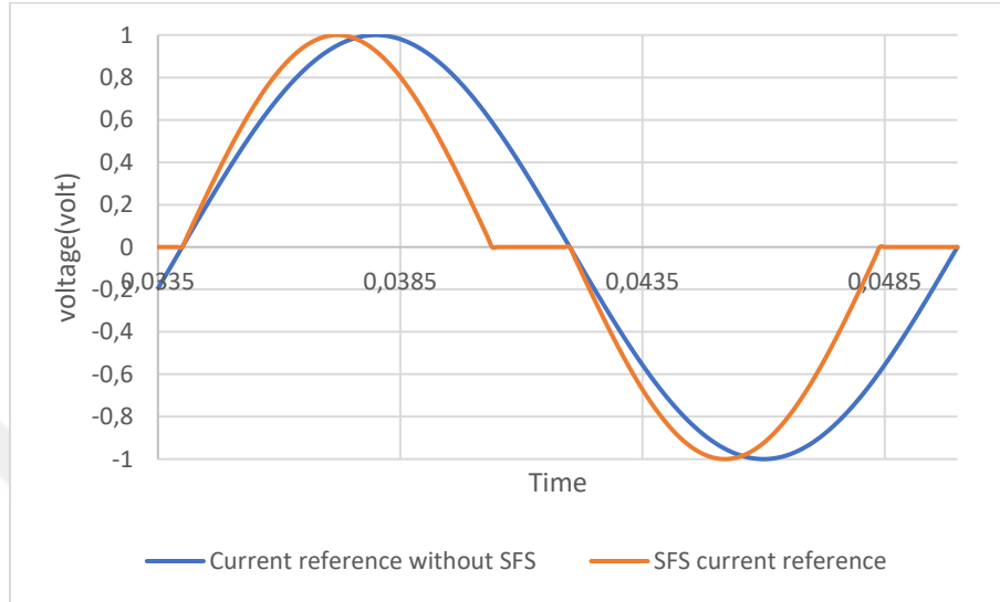
Figure 2.1: Sandia frequency-shift.
