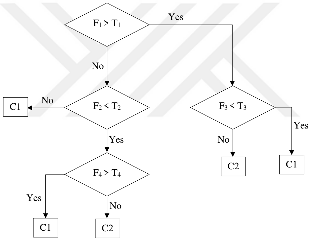
Figure 2.2: Sample decision tree.
