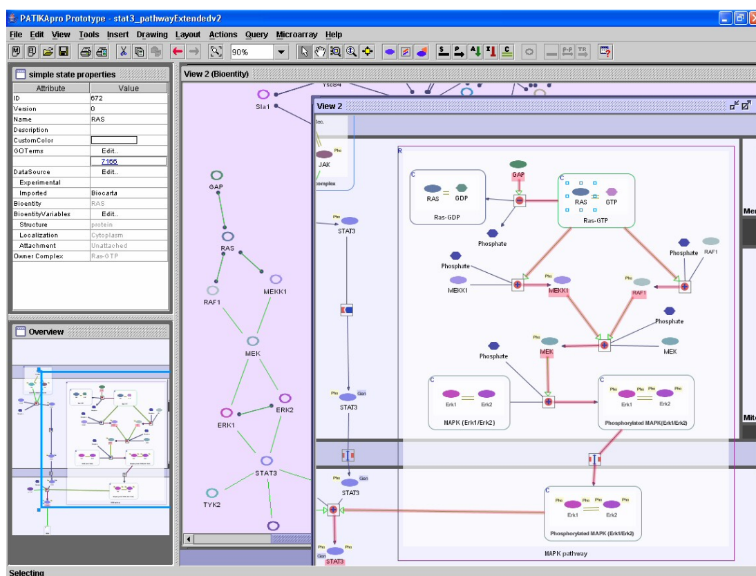
Figure 2.1: Screenshot from PATIKapro
