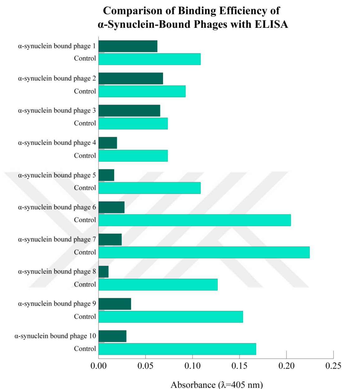
Figure 54: ELISA of \alpha -synuclein and empty pETcon-expressing yeast cells by using \alpha -synuclein-bound phages.
