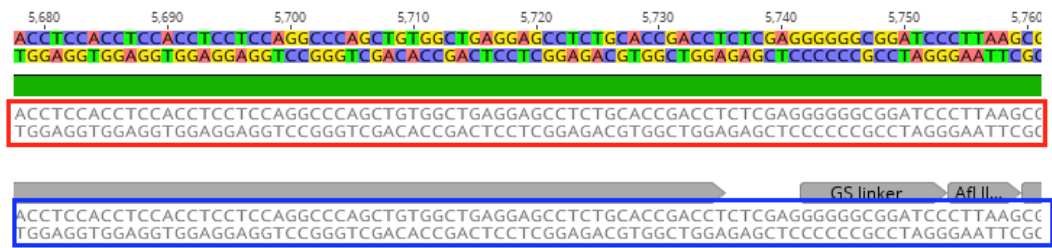
Figure D.7: Sequencing result of 25Q-Htt from pET22b_Ag43_160N_25Q-Htt
