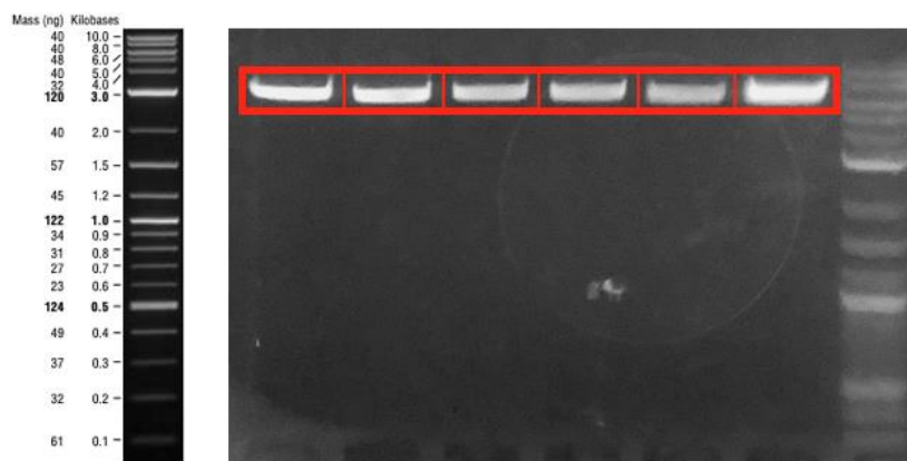
Figure 5: BamHI digestion reactions image. The lane was loaded with digested pETcon vector oh which 25Q-Htt, 46Q-Htt, 103Q-Htt, Amyloid \beta_{40} , Amyloid \beta_{42} , \alpha -synuclein genes expressed respectively.
