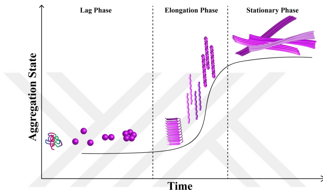
Figure 2: Aggregation phases and amyloid fibril formation mechanism
