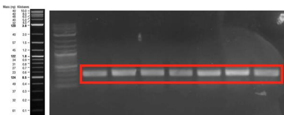
Figure 9: PCR product of 25Q-Htt fragment which was amplified by Gibson assembly primers. The expected band size was 333 bp-long.
