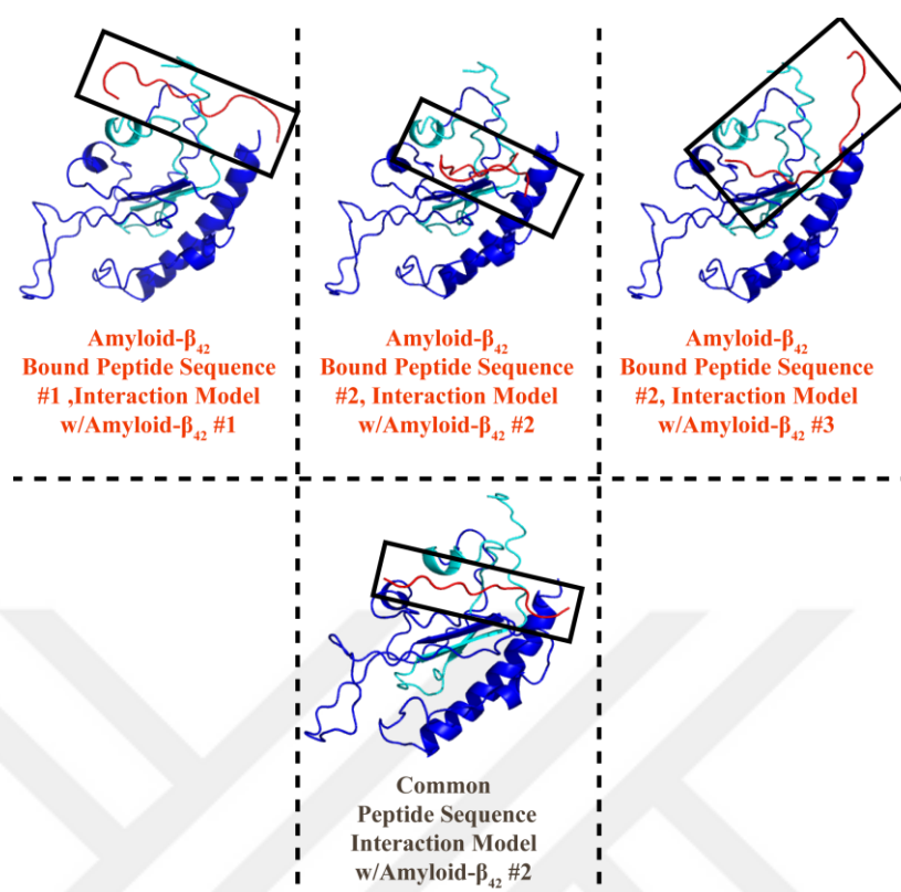
Figure 49: Prediction of docking amyloid- \beta_{42} -bound peptides and common peptide on amyloid- \beta_{42} . The blue region on the model represents Aga2, and cyan region on the model represents amyloid- \beta_{42} . The peptide is indicated with red color and black boxes.
