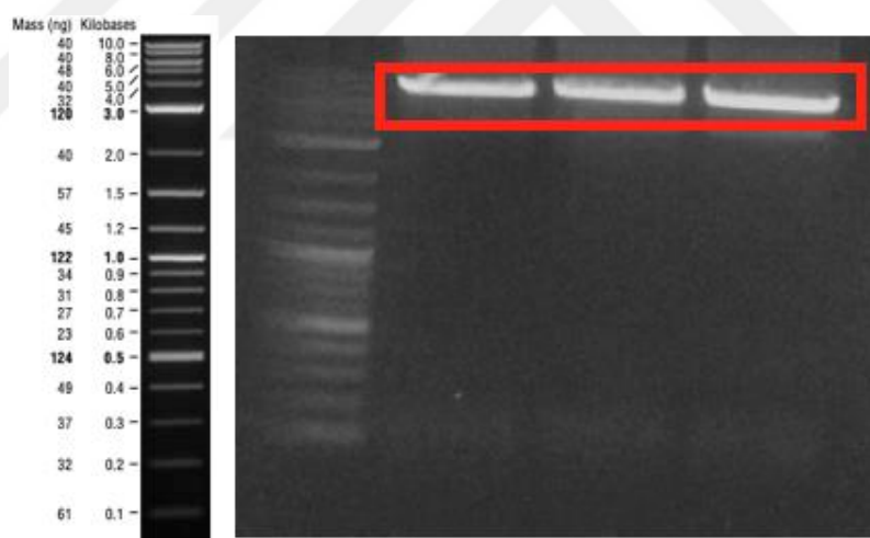
Figure 21: PCR product of M13 genome which was amplified by Gibson assembly primers. The expected band size was 7317 bp-long.
