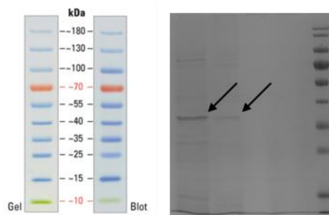
Figure 19: SDS-PAGE gel image result of BL21 cells expressing amyloid- \beta_{40} on surface with fusion of Ag43 autotransporter. First indicated band was from heat release-applied sample which was precipitated with acetone, second indicated band was from heat release-applied sample. Third and fourth lanes were loaded with controls prepared with empty BL21 cells by applying same preparation steps for the first sample and the second sample respectively. The expected band size was 38 kDa.
