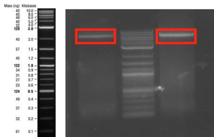
Figure 30: Digestion reaction results of M13 genome PCR product. The expected size was 7227 bp-long.
