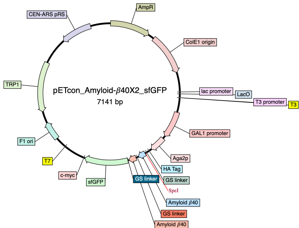
Figure C5: Plasmid map representation of pETcon_Aga2_ Amyloid-β 40 X 2 _sfGFP vector
