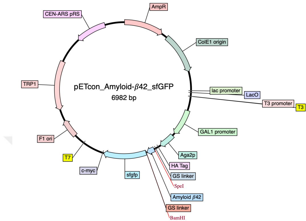
Figure C6: Plasmid map representation of pETcon_Aga2_ Amyloid-β 42 _sfGFP vector
