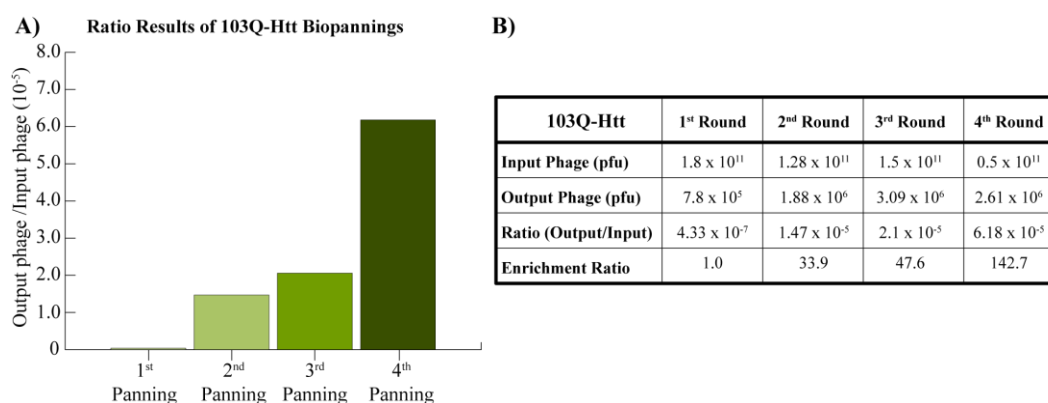
Figure 34: Phage ratio calculations and enrichment ration results from biopanning of 103-Htt. A) Ratio calculations obtained from ‘output phage (pfu)/ input phage (pfu)’ of 103Q-Htt biopanning results. B) Table for input phage amount, output phage amount, ratio and enrichment ratio obtained from 103Q-Htt biopanning.
