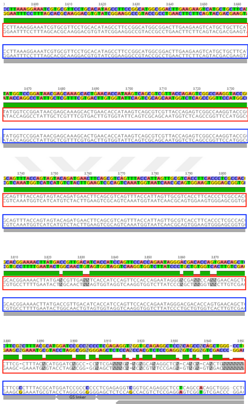
Figure D.1: Sequencing result of sfGFP from pETcon_25Q-Htt_sfGFP
