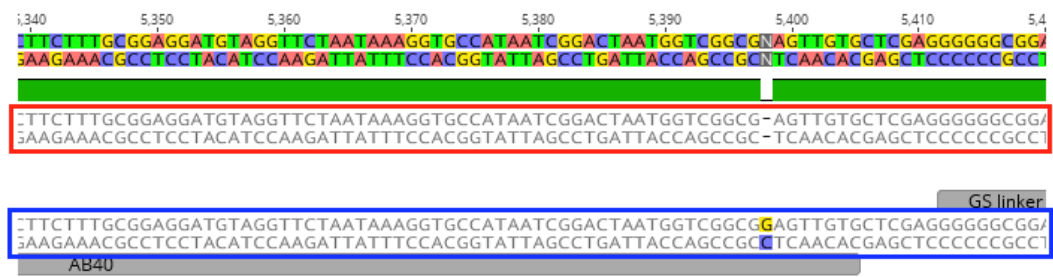
Figure D.10: Sequencing result Amyloid- \beta_{40} from pET22b_Ag43_160N_Amyloid- \beta_{40}
