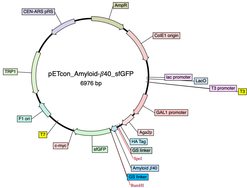
Figure C4: Plasmid map representation of pETcon_Aga2_ Amyloid-β 40 _sfGFP vector
