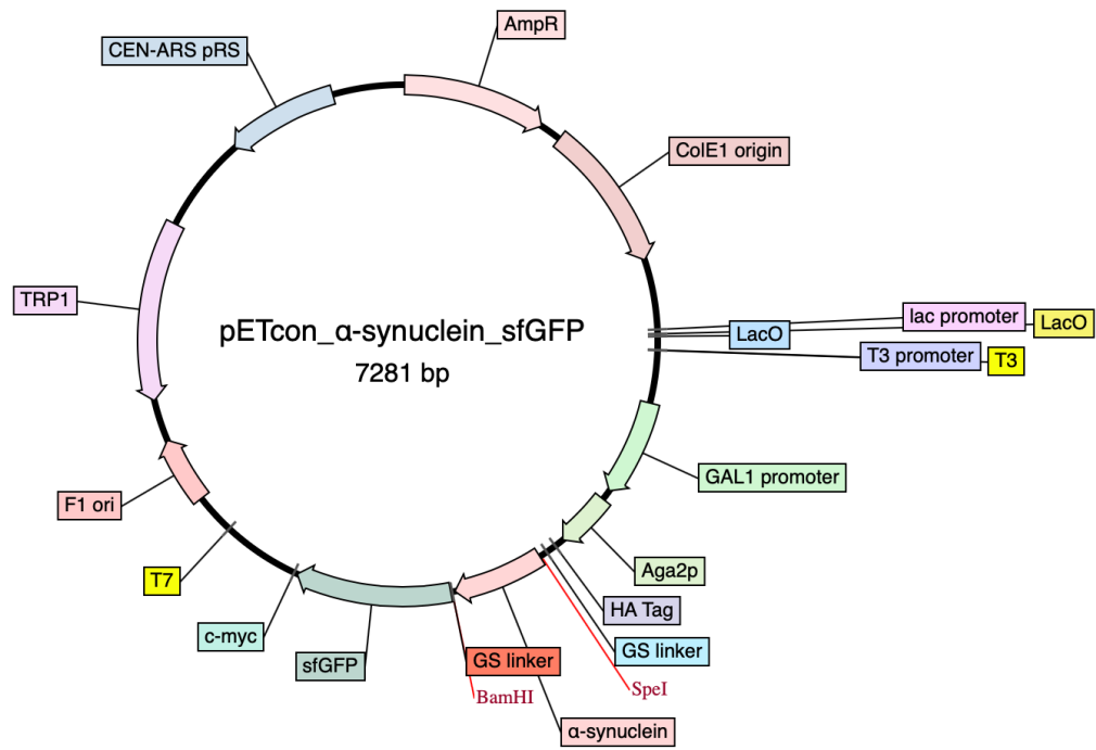
Figure C7: Plasmid map representation of pETcon_Aga2_ \alpha -Synuclein_sfGFP vector
