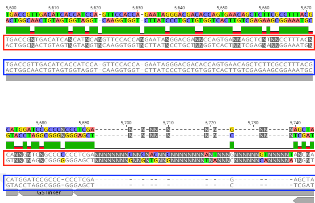
Figure D.5: Sequencing result of sfGFP from pETcon_Amyloid-β 42 _sfGFP
