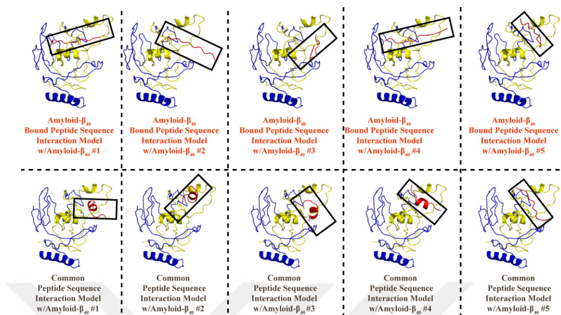
Figure 48: Prediction of docking amyloid- \beta_{40} -bound peptide and common peptide on amyloid- \beta_{40} . The blue region on the model represents Aga2, and yellow region on the model represents amyloid- \beta_{40} . The peptide is indicated with red color and black boxes.
