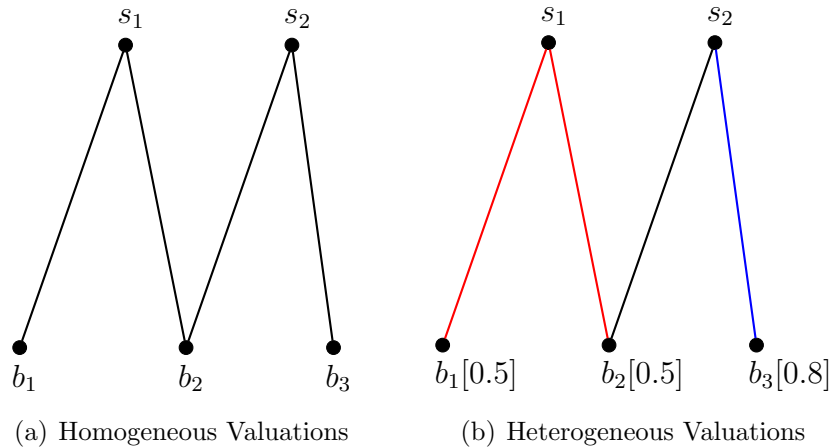
Figure 3.1: Two Sided Supply Chain Network G
