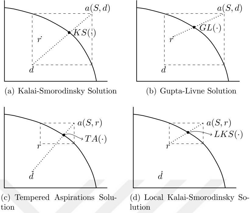
Figure 5.2: Four Bargaining Solutions as Members of the (\alpha, \beta) -Family
