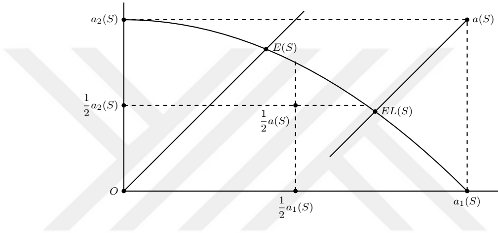
Figure 6.1: E and EL violate MD
