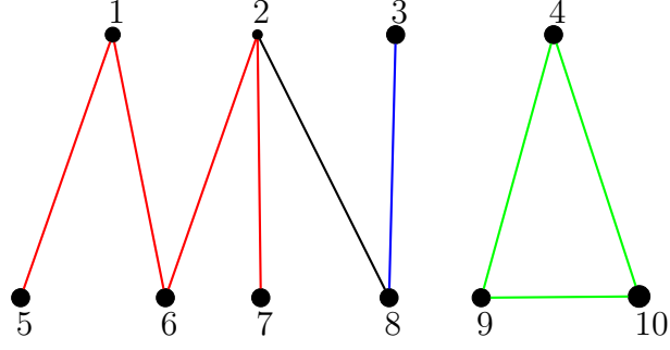
Figure 2.1: Network G
