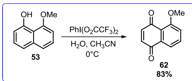
Scheme 25. Preliminary study of oxidation of the phenol 53 .
