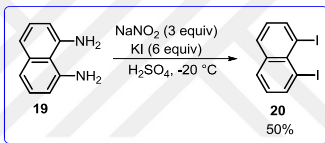
Scheme 13. The synthesis of 1,8-diiodonaphthalene ( 20 ).
