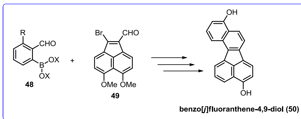
Scheme 19. Synthesis of benzo[j]fluoranthene-4,9-diol ( 50 ).
