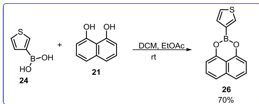
Scheme 16. The synthesis of boronic ester (26).
