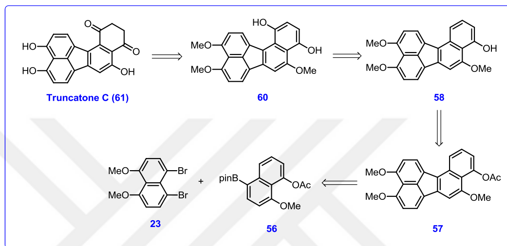
Scheme 21. Retrosynthetic analysis of truncatone C ( 61 ).
