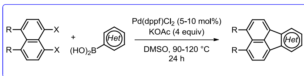
Scheme 11. The synthesis of heteroaromatic fluoranthene analogues.
