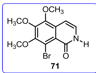
Figure 13. Hydrolysis product 71 .
