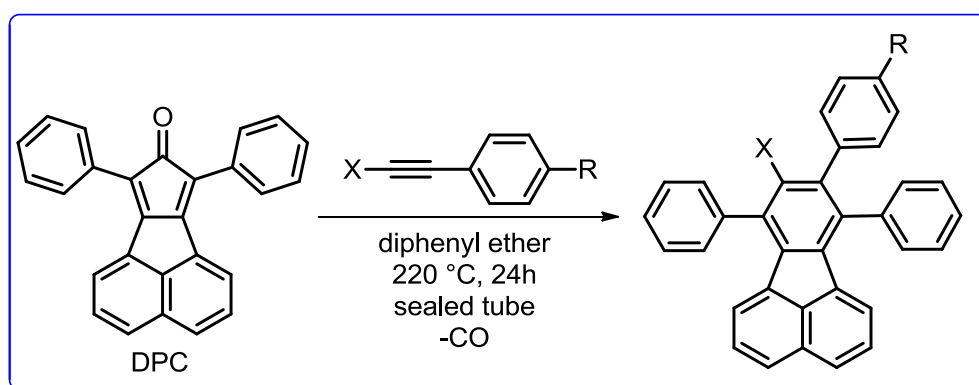
Scheme 3. Synthetic route for preparation of fluoranthene derivatives.
