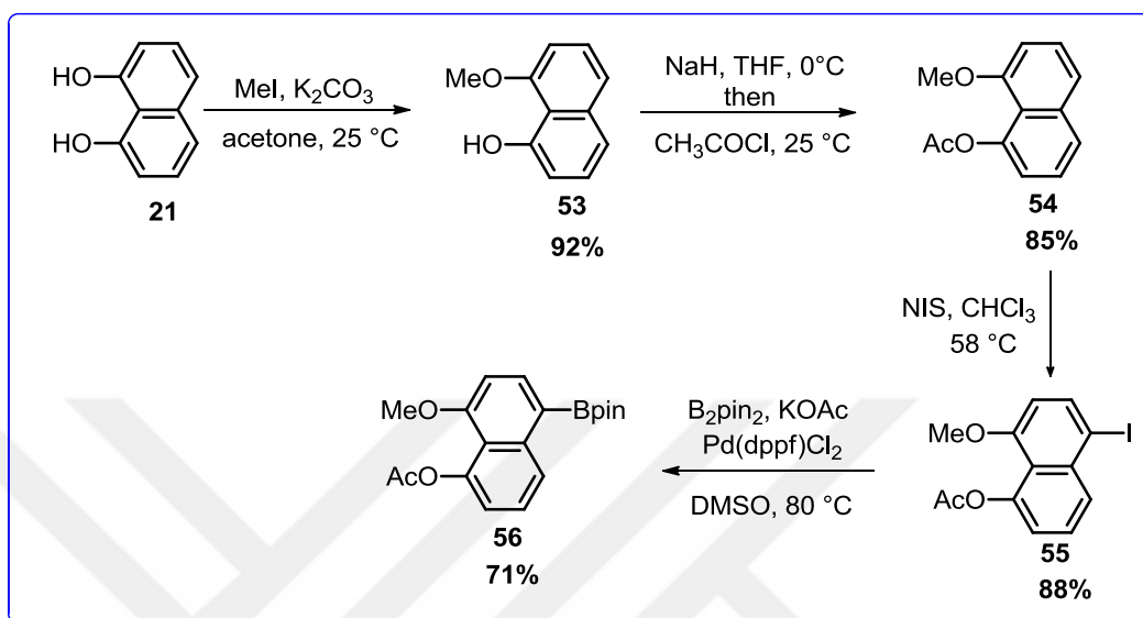
Scheme 22. Synthesis of arylboronic ester.
