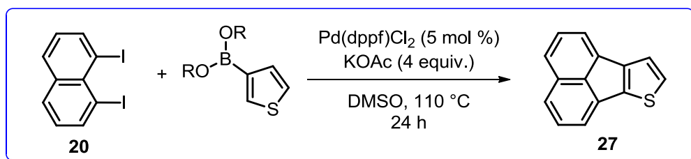
Scheme 17. The synthesis of compound 27 from boronic esters.
