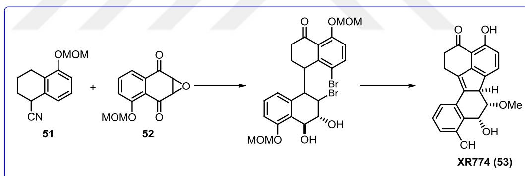
Scheme 20. The synthesis of XR774 ( 53 ).
