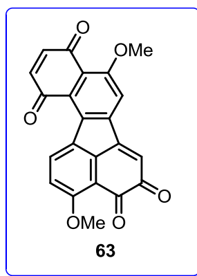
Figure 12. Overoxidation product 63 .
