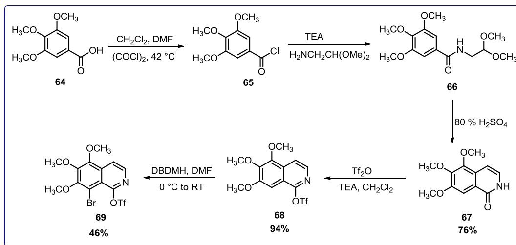
Scheme 26. The synthesis of the starting material of imeluteine.
