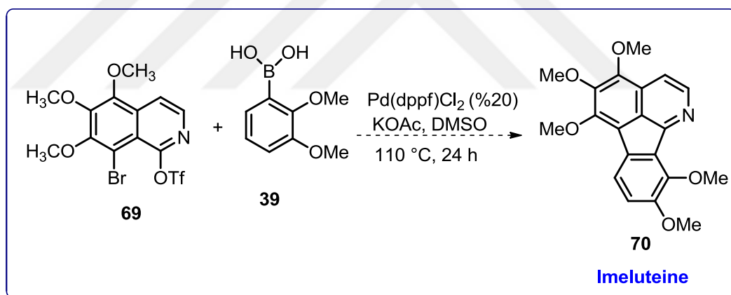
Scheme 27. Planned imeluteine synthesis.
