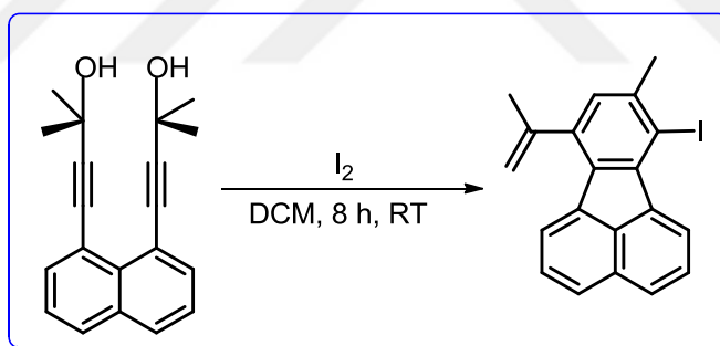
Scheme 7. Synthesis of a fluoranthene via iodine-mediated cyclizations.
