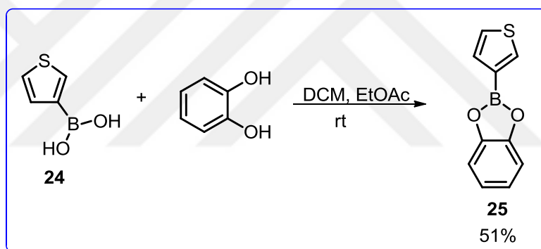
Scheme 15. The synthesis of catechol boronic ester ( 25 ).
