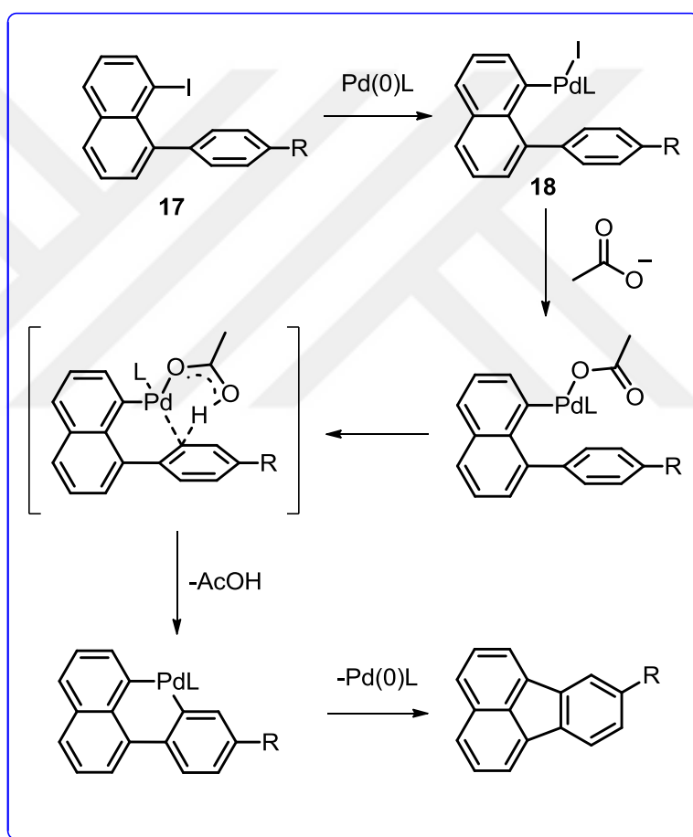
Scheme 12. Proposed reaction mechanism.
