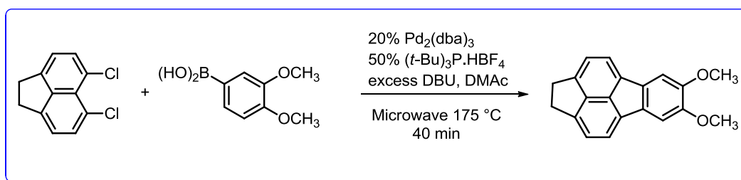
Scheme 8. Fluoranthene synthesis by a Suzuki-Heck-type coupling cascade.
