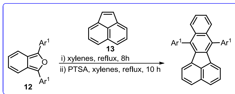
Scheme 1. Diels-Alder reaction of benzo[ c ]furans ( 12 ) with acenaphthylene ( 13 ).
