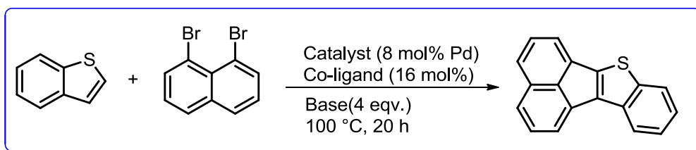
Scheme 4. Pd-catalyzed C-H activation reaction of benzo[ b ]thiophene with 1,8-dibromonaphthalene.
