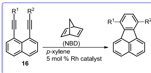
Scheme 6. Preparation of fluoranthenes from Diynes and NBD.
