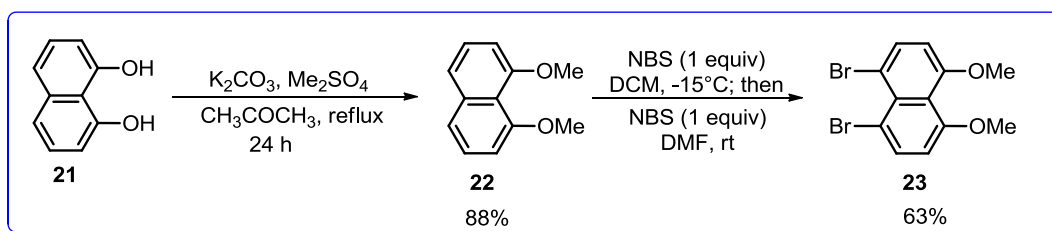
Scheme 14. The synthesis of 1,8-dibromo-4,5-dimethoxynaphthalene ( 23 ).
