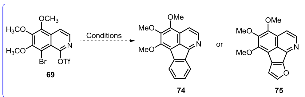
Scheme 28. Planned fluoranthene syntheses.
