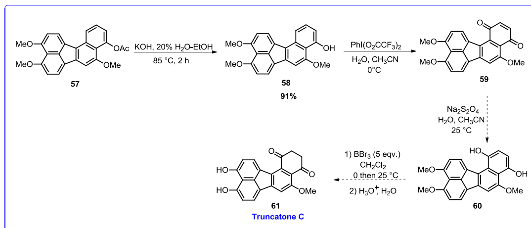
Scheme 24. The planned synthesis of truncatone C.
