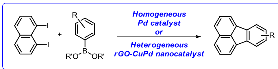
Scheme 10. Synthesis of fluoranthene derivatives via tandem Suzuki-Miyaura and intramolecular C-H arylation.
