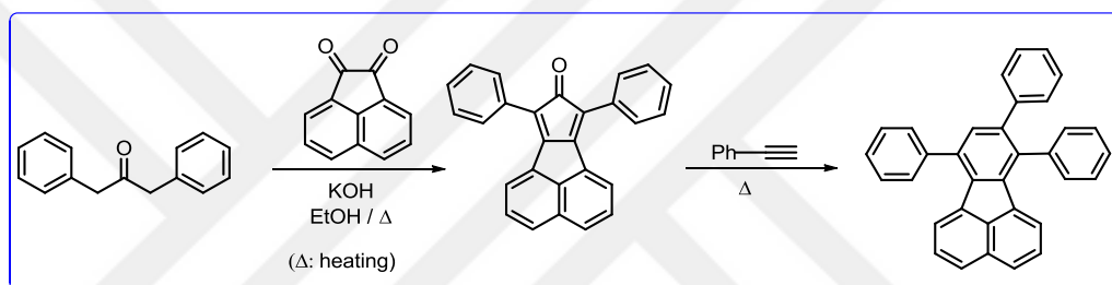
Scheme 2. The synthesis of 7,8,10-triphenylfluoranthene.
