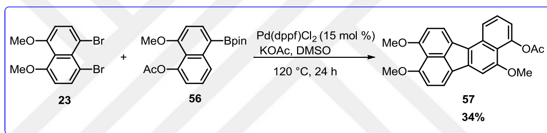
Scheme 23. Synthesis of benzo[j]fluoranthene.
