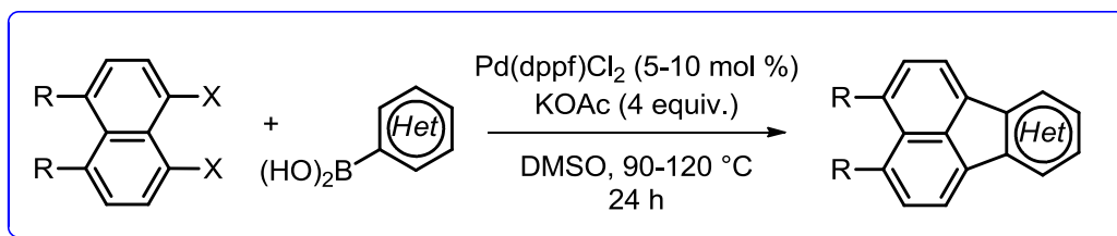
Scheme 18. The synthesis of fluoranthene analogues.
