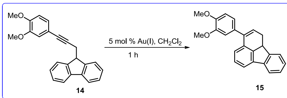
Scheme 5. Gold(I)-catalyzed hydroarylation of 14 to give 1,10b-dihydrofluoranthene ( 15 ).
