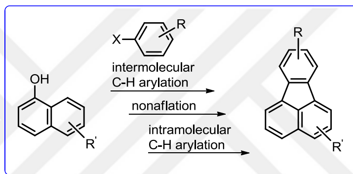
Scheme 9. Three step synthesis of fluoranthenes.
