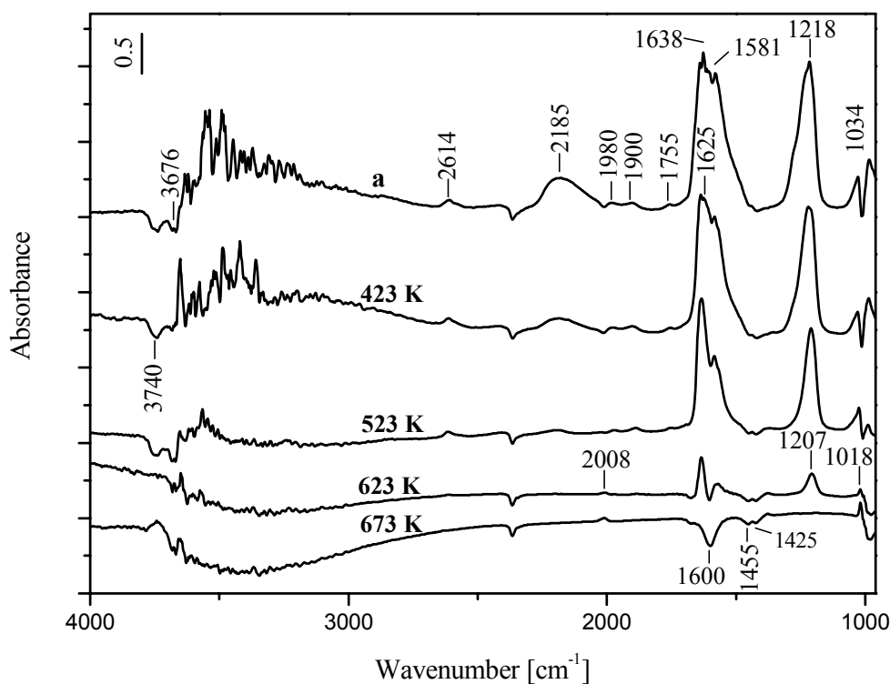
Figure 15. FT-IR spectra obtained after adsorption of NO/O 2 at RT followed by evacuation for 10 min (a), after heating the WZ sample containing adsorbed NO x species for 15 min in vacuum. The spectra are recorded after cooling of the IR cell to the room temperature. The spectrum of the activated sample is used as a background reference.
