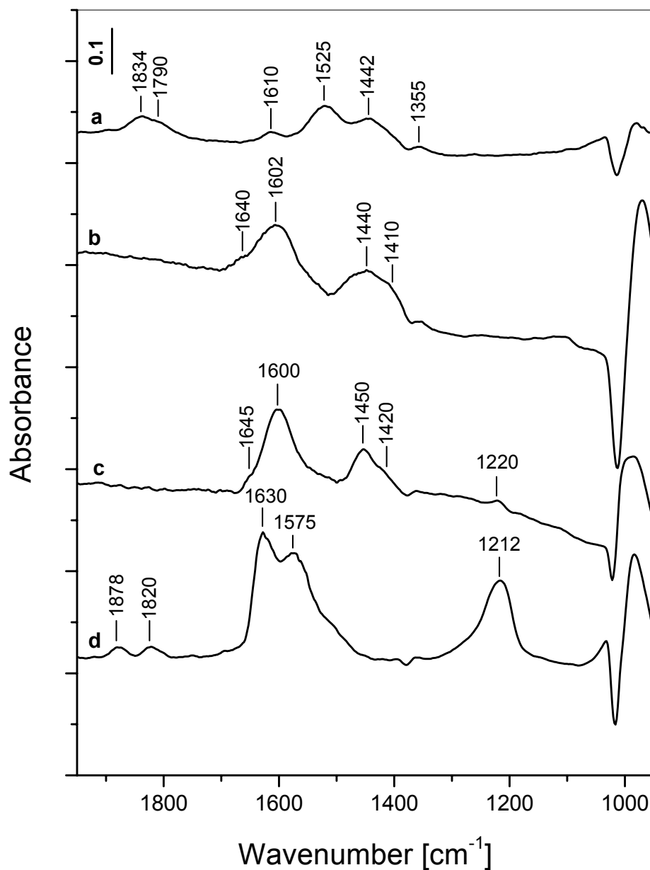
Figure 26. FT-IR spectra of the Pd/WZ catalyst taken from the interaction of the preadsorbed NO x with CH 4 at 673 K (a) and after evacuation at room temperature (b), the “Blank CH 4 ” (c), and the “Blank NO x ” (d) experiments after the final evacuation at room temperature. The spectrum of the activated sample is used as a background reference.
