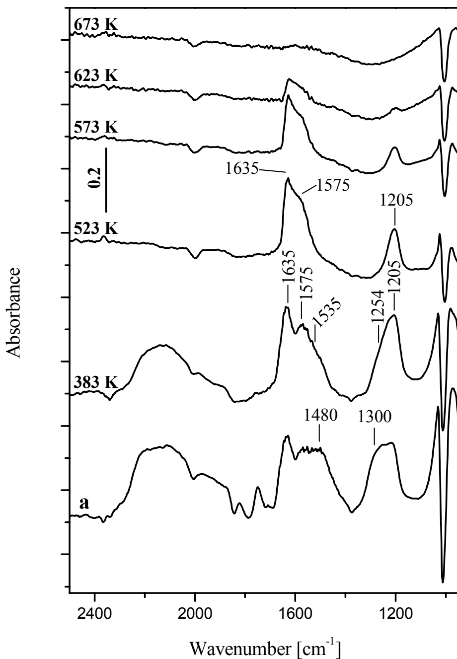
Figure 17. FT-IR spectra obtained after adsorption of \text{NO/O}_2 at RT followed by evacuation for 10 min (a), after heating the Pd/WZ sample containing adsorbed \text{NO}_x species for 10 min in vacuum. The spectrum of the activated sample is used as a background reference and the gas phase spectra are subtracted.
