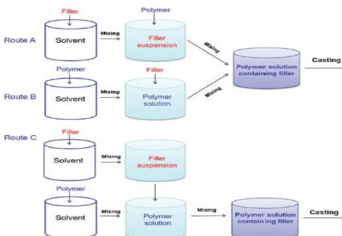
Figure 26. Possible methods to synthesize MMMs (Lin et al. 2018)
