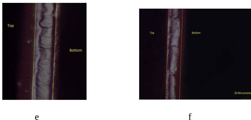
Figure 41. (cont'd) Keeping the solvent that mixed with pink dye on one-day cast membrane (M1.c) for a) 30 sec, b) 1 min, c) 5 min, d) 30 min e) 1-hour f) 2 hours
