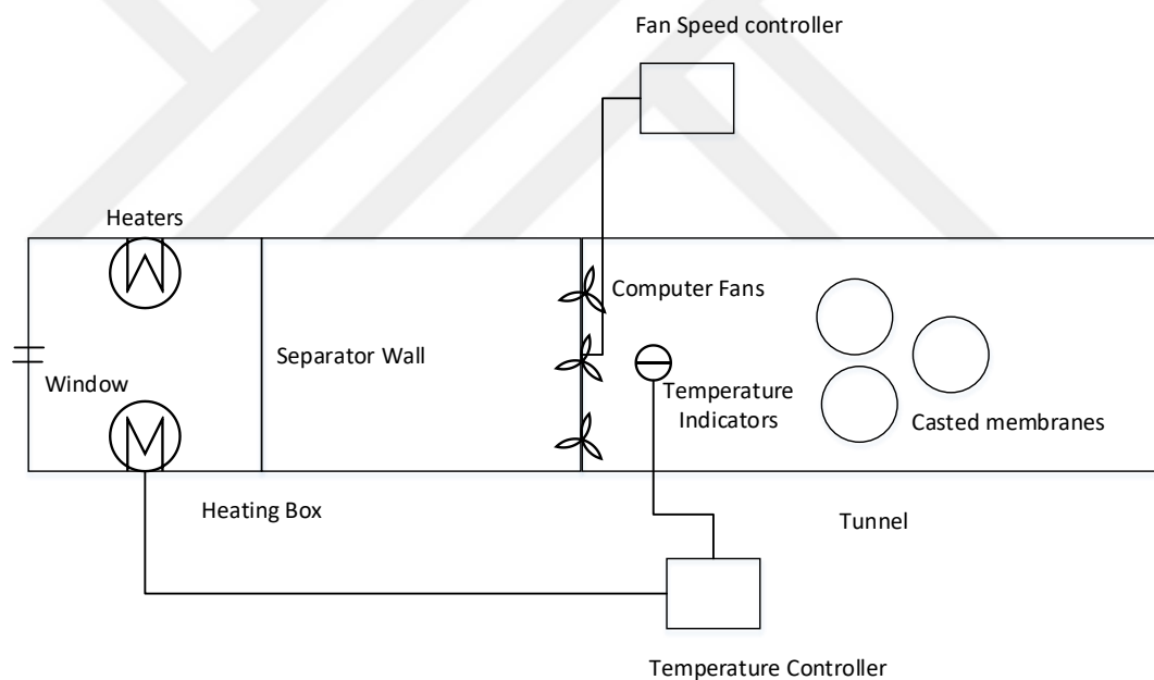
Figure 24. Casting system in 2D
