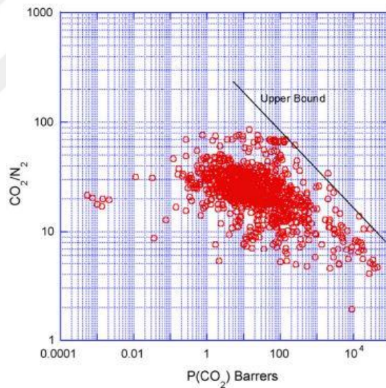
Figure 10. Upper bound correlation for CO 2 /N 2 separation (Robeson 2008)
