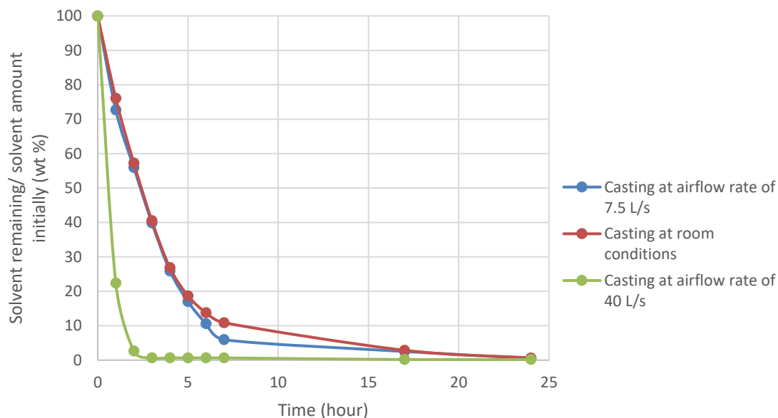
Figure 35. Evaporation rate of solvent in the casting step
