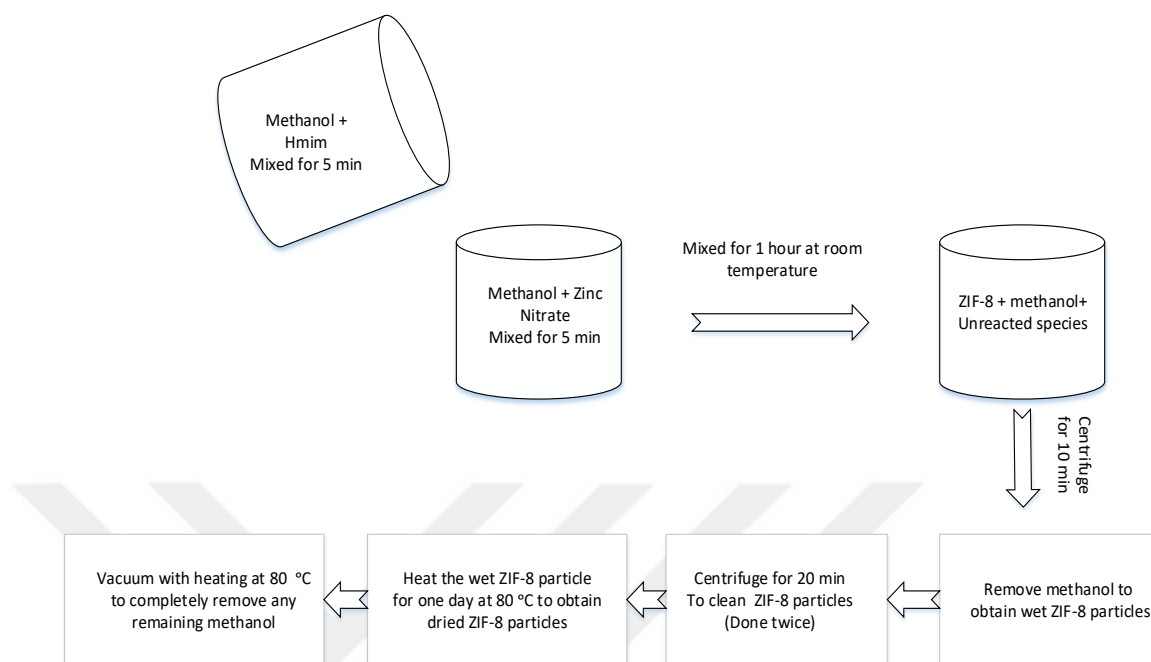
Figure 25. Synthesis procedure of ZIF-8
