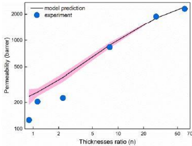
Figure 23. The variation of permeability results (by experiment and simulation) with a thickness ratio of (PDMS/PEBAX 1657) (Selyanchyn et al. 2018)
