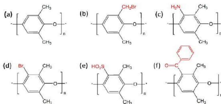
Figure 14. Structure of chemically modified PPO: (a) PPO; (b) BPPO; (c) PPO-NH 2 ; (d) PPOBr; (e) sulfonated PPO; (f) benzyloylated PPO (Yuan et al. 2016).
