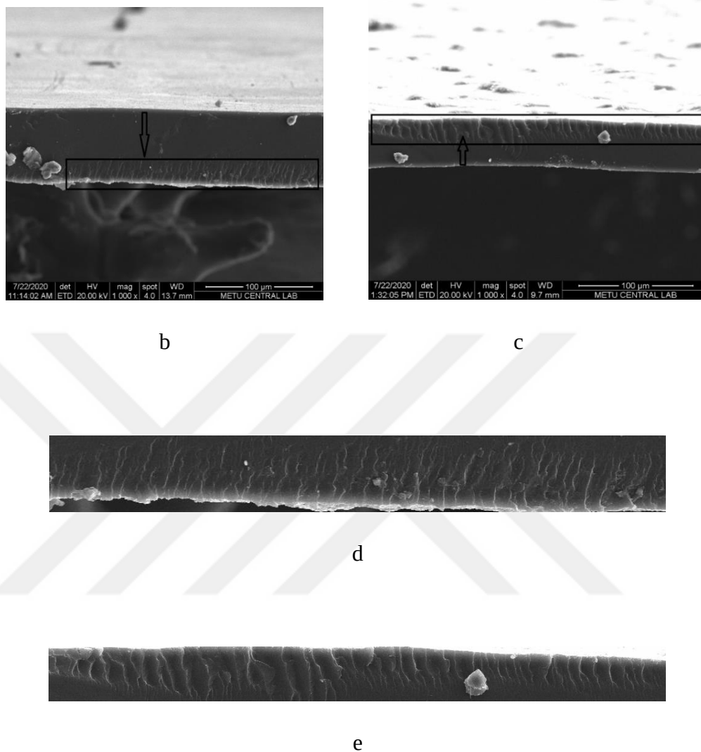
Figure 43. (cont'd) SEM analysis for synthesized membranes a) M1.a, b) M2, c) M3, d) M2 (modified part is magnified), and e) M3 (modified part is magnified)
