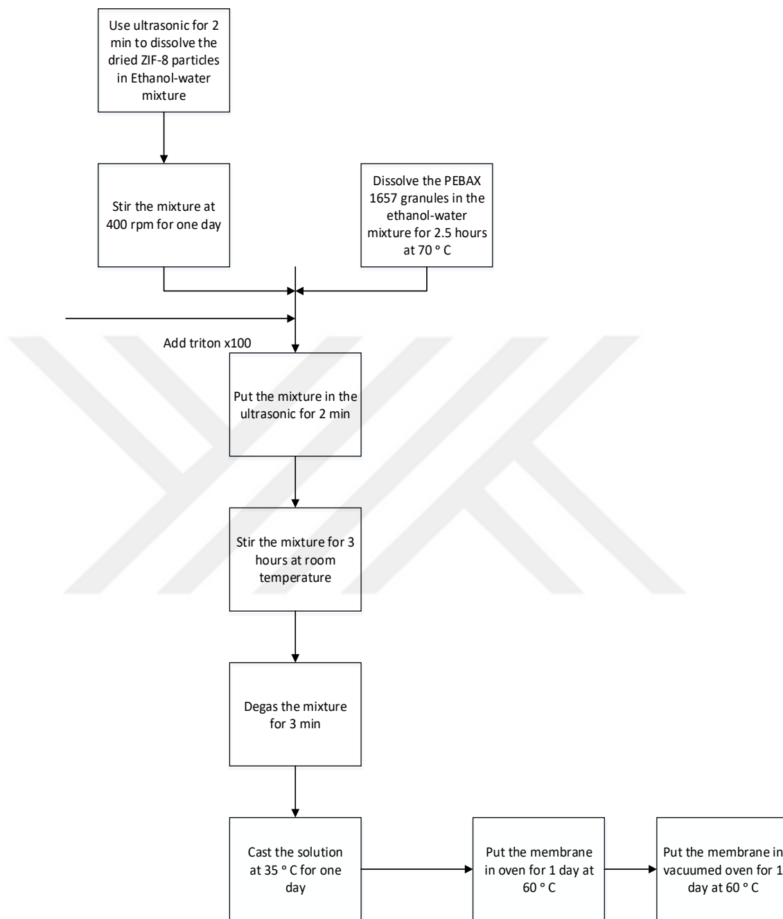
Figure 27. PEBAX 1657 + ZIF-8 MMM synthesis procedure
