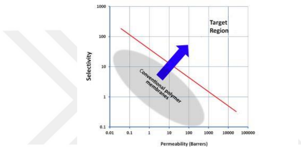
Figure 5. Robeson Upper Bound for polymeric membranes (Panapitiya et al. 2016)
