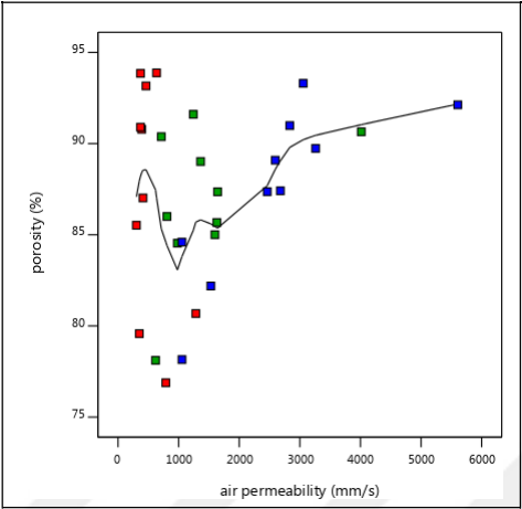
Figure 4.22 Relationship between porosity –air permeability
