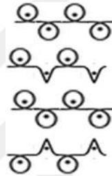
Figure 3.26 Half Cardigan fabric needle diagram
