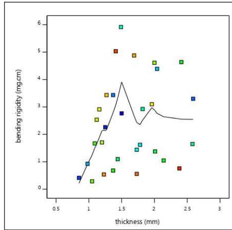
Figure 4.38 Relationship between bending rigidity-thickness
