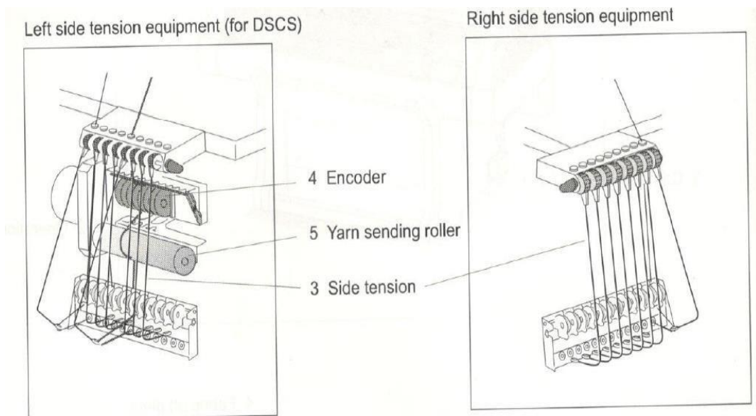
Figure 3.4 Left and right side tension equipments [18]
