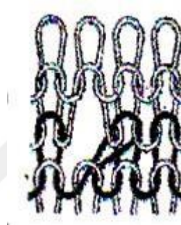
Figure 3.35 Lace fabric construction [26]
