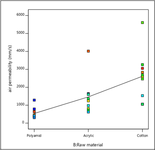
Figure 4.53 Effect of raw material on the air permeability of samples statistically
