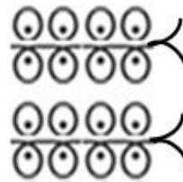
Figure 3.20 Interlock fabric needle diagram
