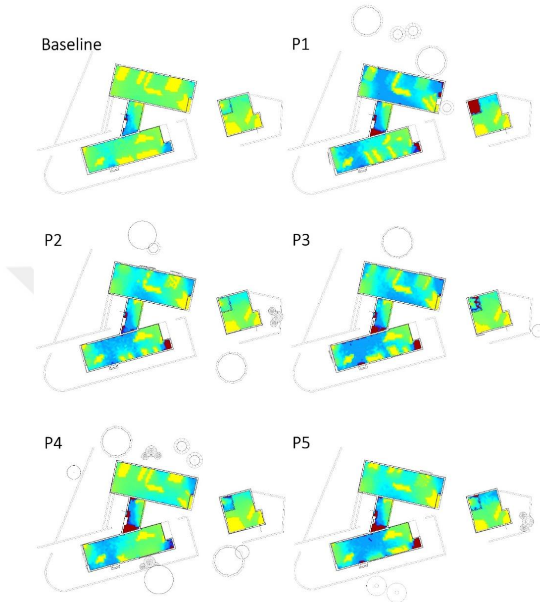
Figure 5.17. Daylighting analysis results of the design outputs (where yellow represents high lux values)
