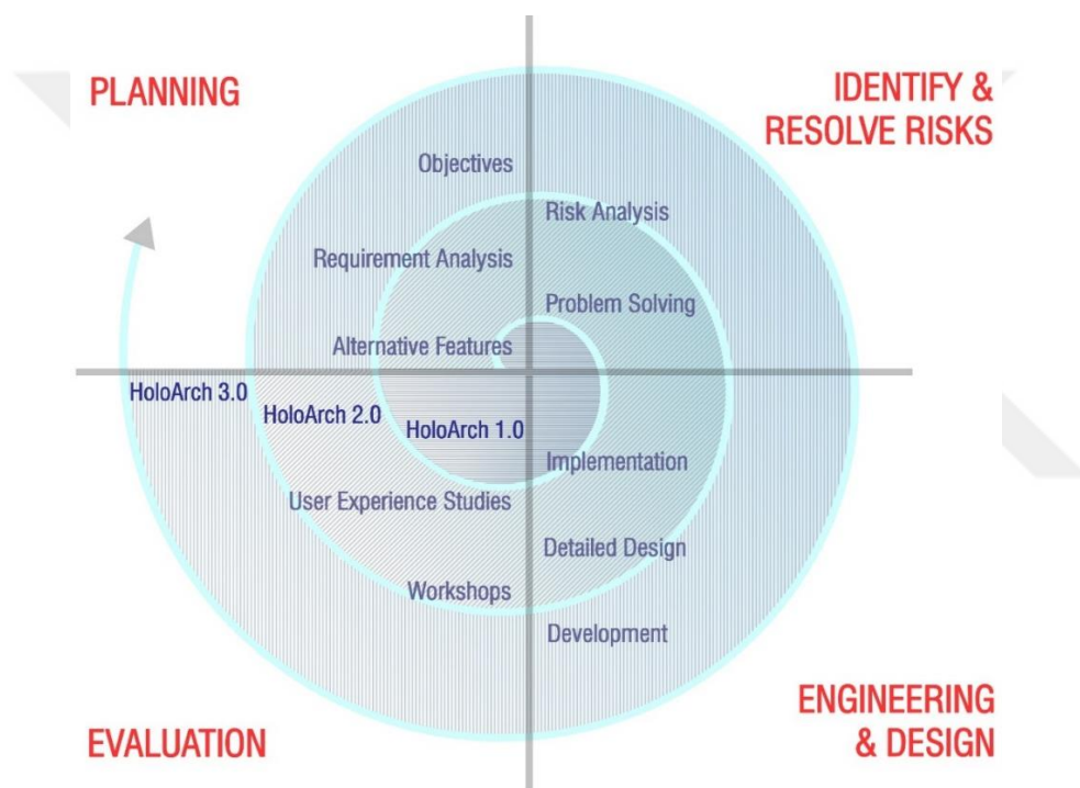
Figure 3.4. Spiral software development process model 92 for HoloArch
