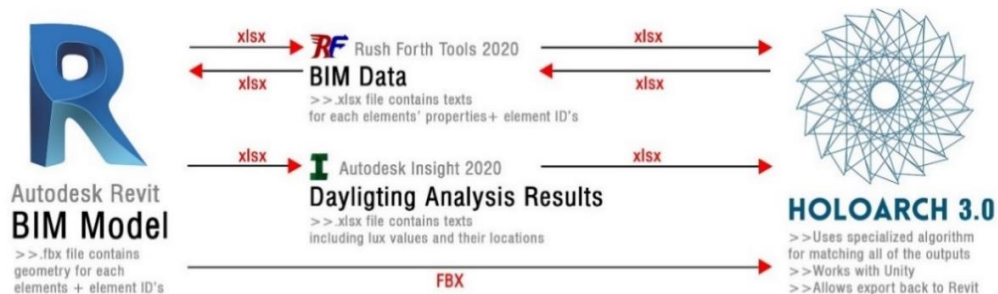
Figure 3.8. Communication between the involved tools
