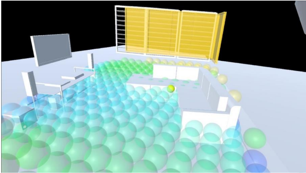
Figure 3.23. Space planning according to daylighting simulations
