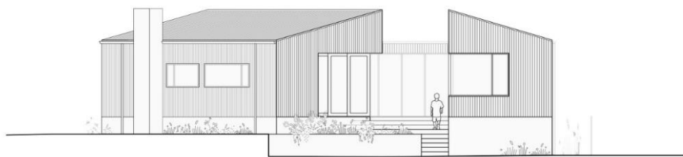
Figure 5.3. Elevation drawing of Three Piece House by TRIAS Studio 136
