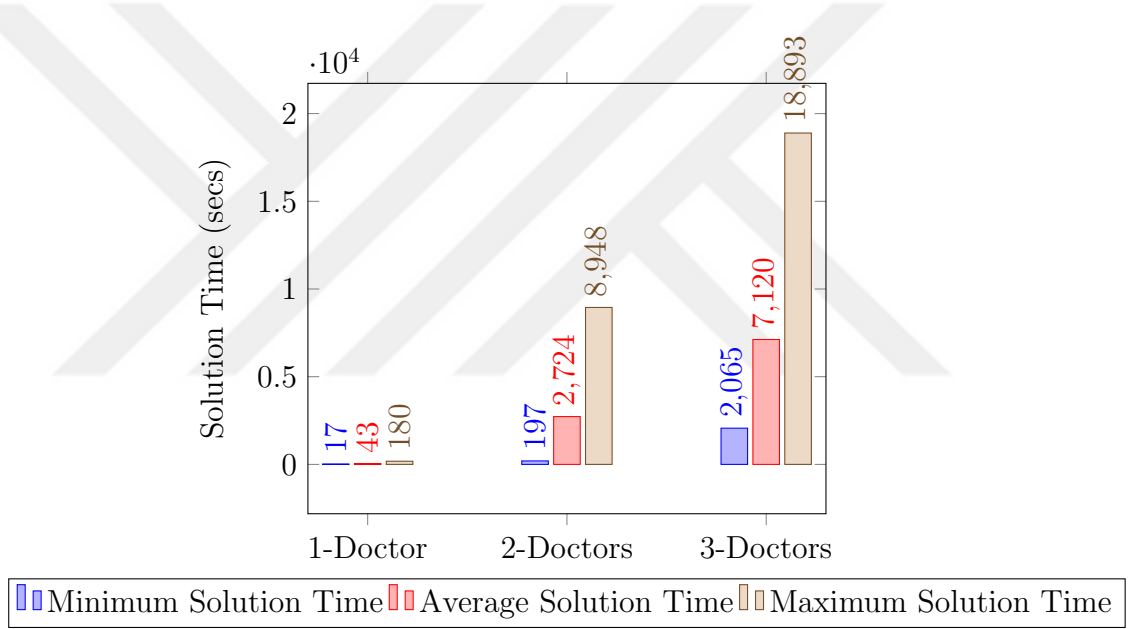
Figure 6.3: Solution Time Comparisons Based on Number of Doctors
