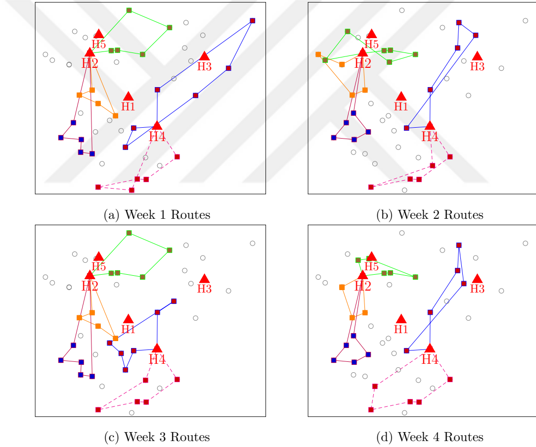
Figure 8.2: Large Data Set - Instance 1, Weekly Routes of Heuristic-2
