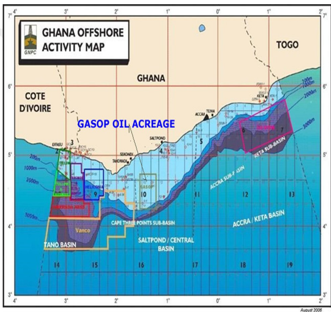
Figure 5.62. Ghana's offshore activity map (GASOP OIL, 2019).
