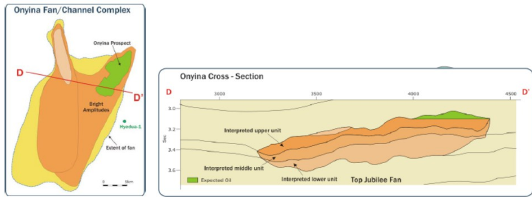
Figure 5.68. Onyina prospect of the Tano basin (Tullow oil, 2008).
