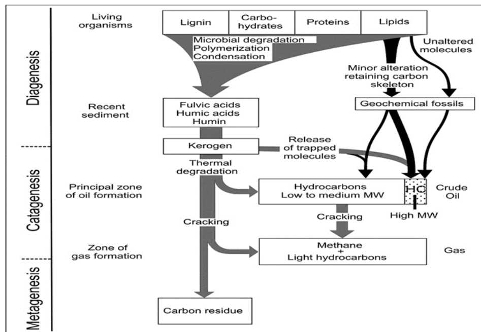
Figure 3.18 Petroleum formation in organic rich sediments (Tissot and Welte, 1984 as cited by Abay, 2017).
