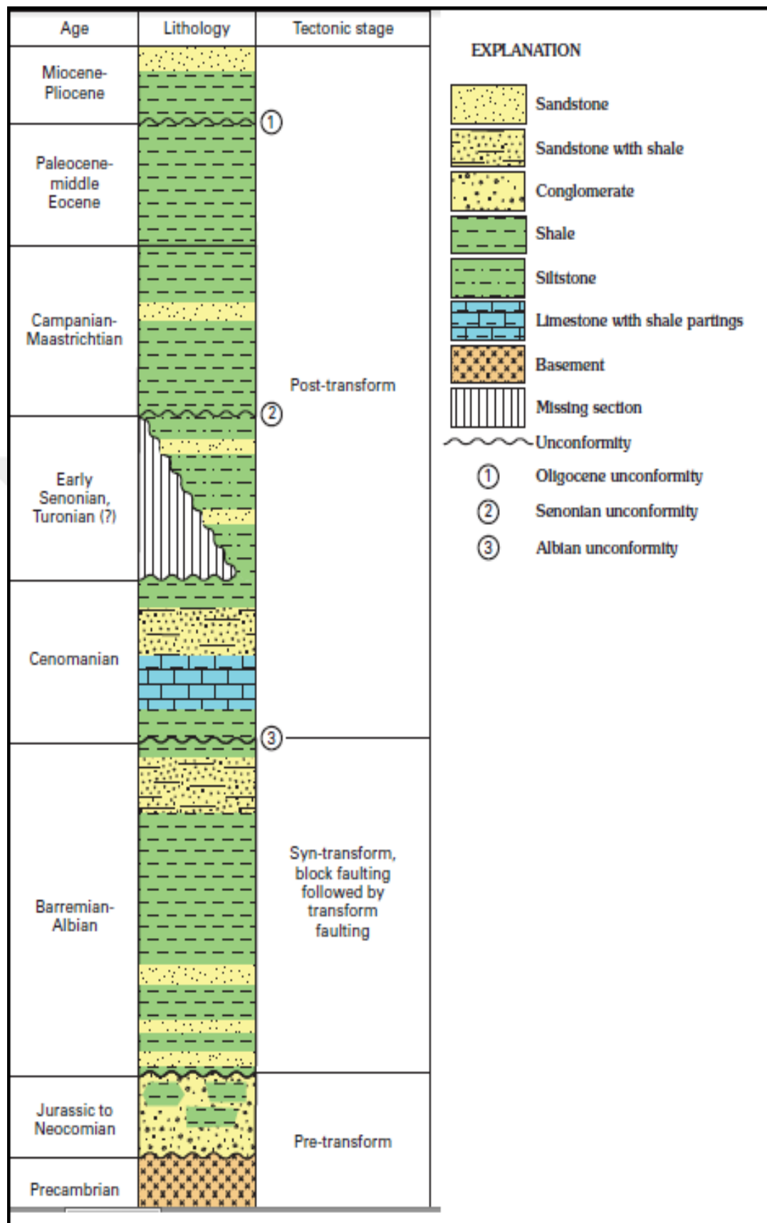
Figure 4.26. Stratigraphy of the Tano Cape Three Points Basin of Ghana (Doku, 2015).
