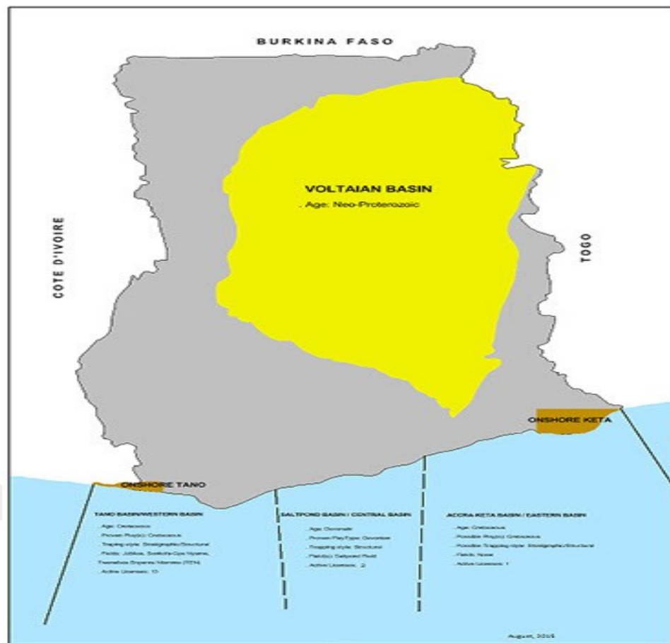
Figure 4.23. Sedimentary basins in Ghana (Petroleum Commission, 2019).
