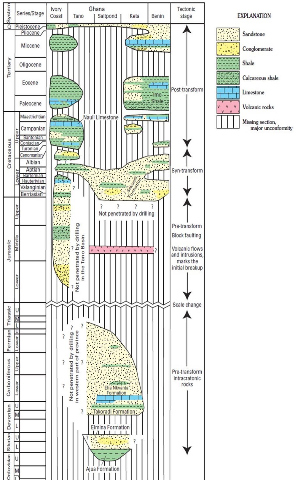
Figure 4.24. Stratigraphic section of the Basins in Ghana along the Gulf of Guinea (Brownfield, 2016).
