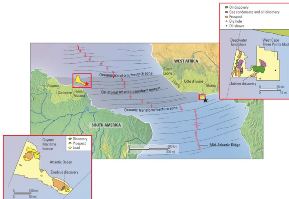
Figure 5.70. The Jubilee field of Ghana and French Guyana (adopted from Tullow oil cited in Bryant et al., 2012).
