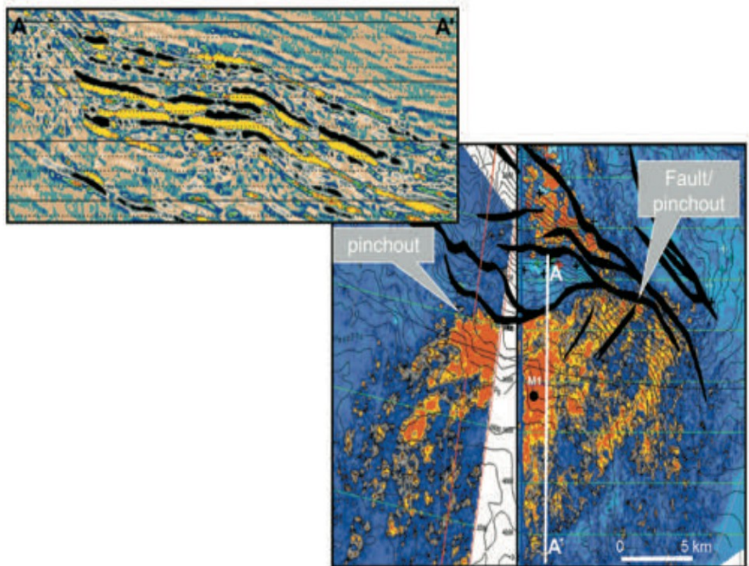
Figure 5.35. Mahogany-1 well in Jubilee field of the Tano basin (N-S seismic line and RMS far amplitude map), # obtained from Dailly et al., 2017.
