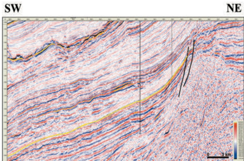
Figure 5.38. NE-SW 2D dip line through Mahogany showing the up-dip trapping, obtained from Dailly et al., 2017).
