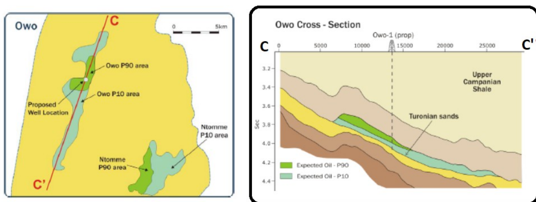
Figure 5.67. Ntomme and Owo prospects of the Tano basin (Tullow oil, 2008).
