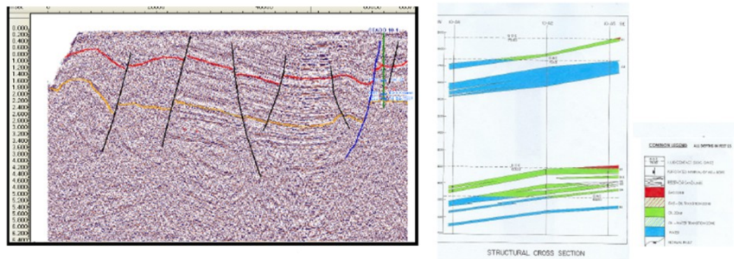
Figure 5.54. Seismic section of the Saltpond basin (Aryeetey, 2014).
