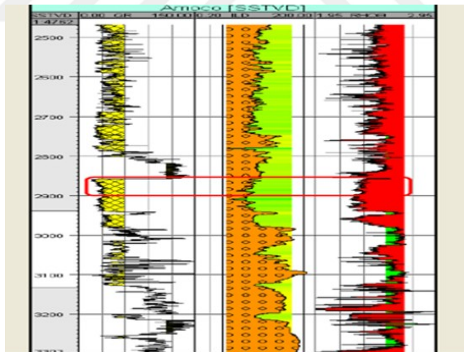
Figure 5.58. Gamma ray log, density and resistivity log used to determine the hydrocarbon saturation zones (Arku, 2012).
