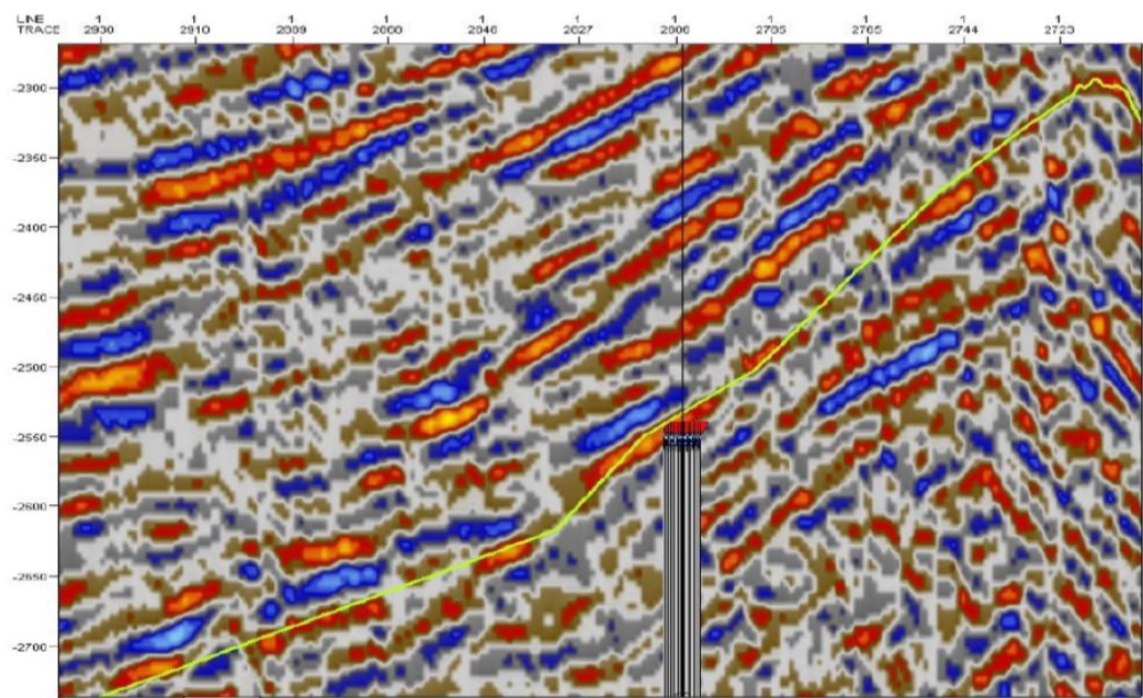
Figure 5.59. Seismic section of synthetic ties with horizon H1 picked (Arku, 2012).
