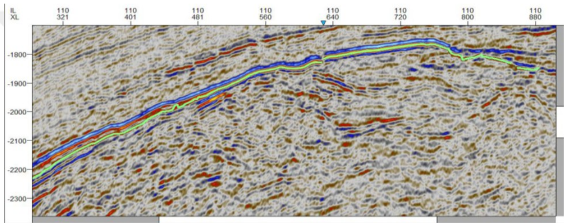
Figure 5.50. Horizontal interpretation made from the seismic section attained (Obtained from Fontem, 2019).
