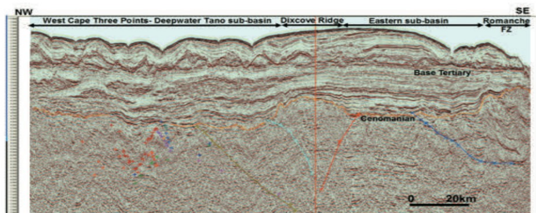
Figure 5.33. Seismic section of the Tano basin displaying some structural features and some fault zones. Obtained from Dailly et al., 2019.
