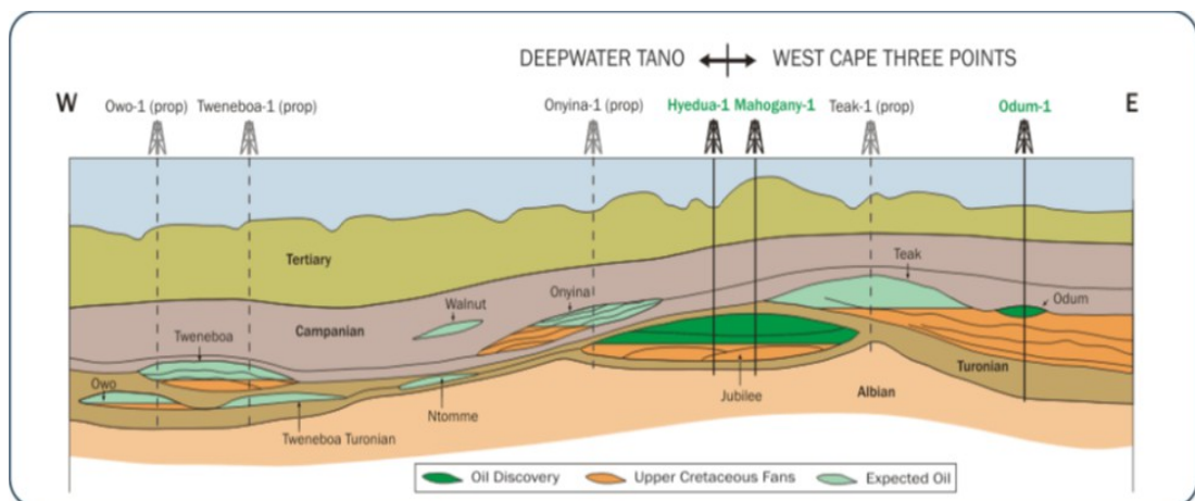
Figure 5.64. W-E cross section of prospects in the Tano basin (Tullow oil, 2008).
