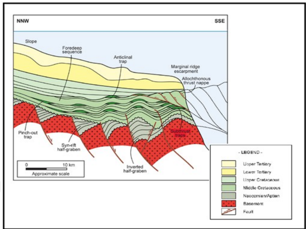
Figure 4.25. Cross section of offshore Tano basin showing the play types present (IHS Report, 2011 as cited by Tetteh, 2016).
