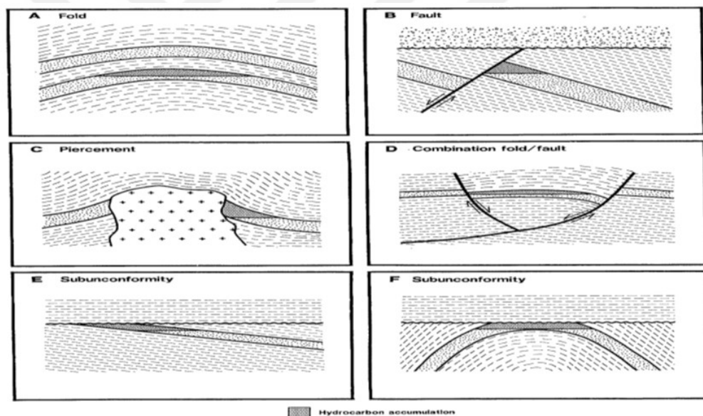
Figure 3.12. Common types of Structural traps in a hydrocarbon system (Magoon and Dow, 1994).
