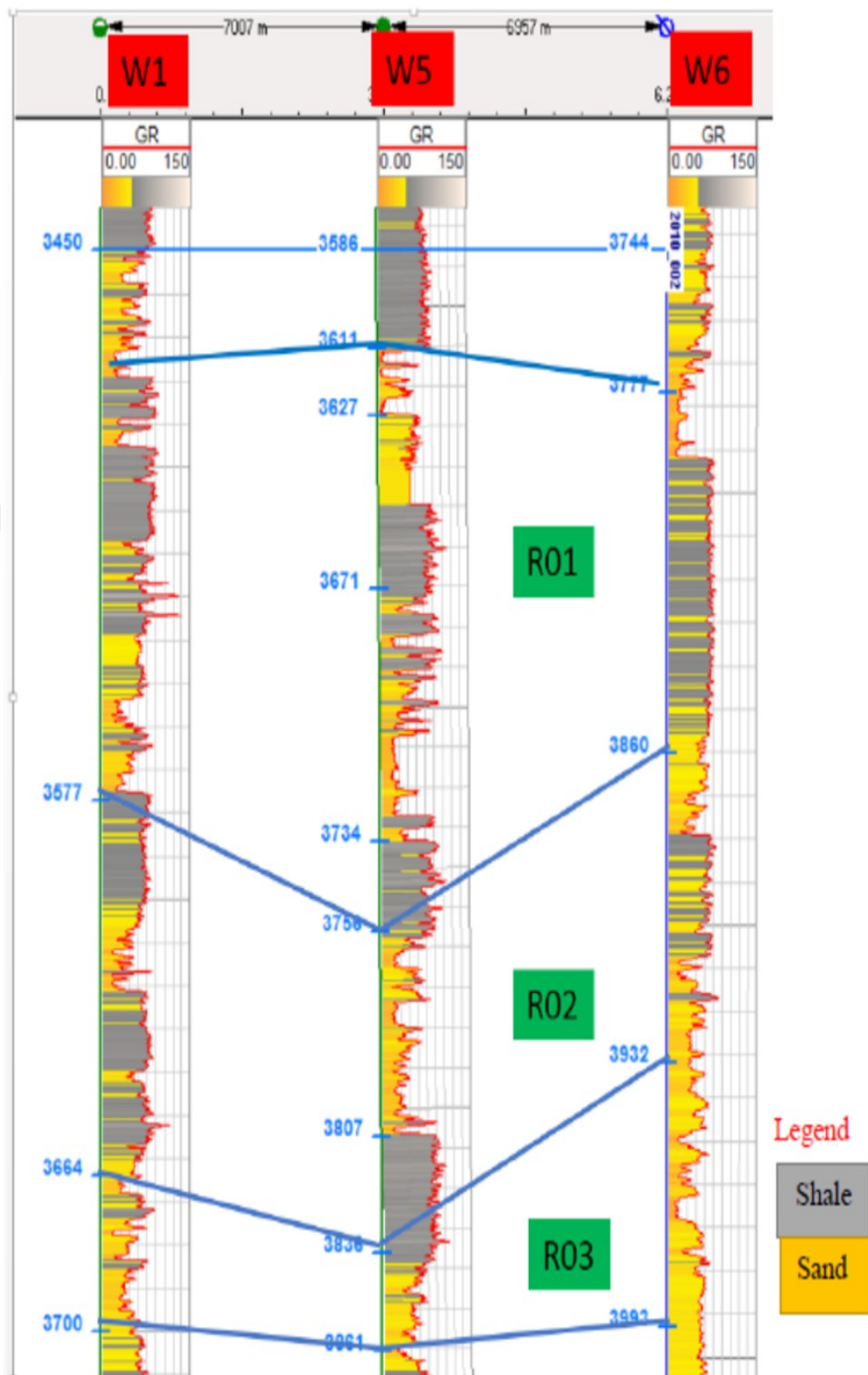
Figure 5.42. Well correlation within the Sovereign 1, obtained from Ablordeppey, 2016.
