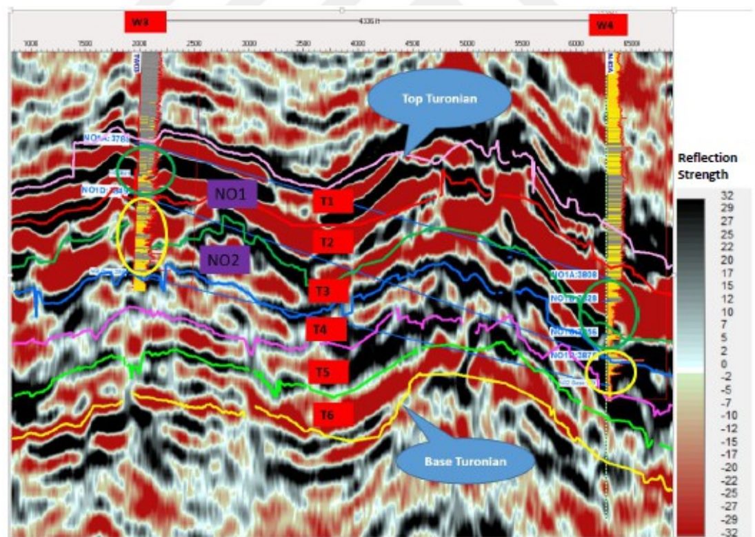
Figure 5.45. The behaviour of sands and shales units from Well to Seismic (EEI Data) tie and ISO-Proportional Intervals - B, obtained from Ablordeppey, 2016.
