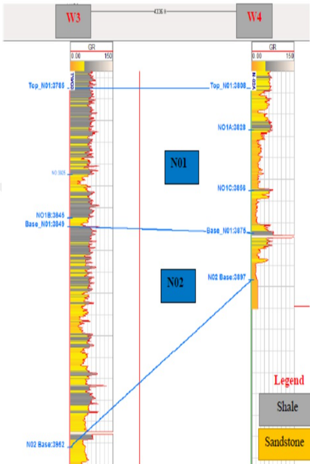
Figure 5.43. Well correlation within the Sovereign 2, obtained from Ablordeppey, 2016.
