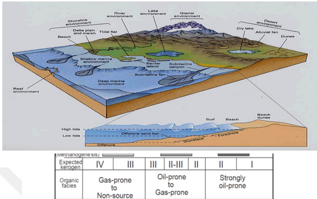
Figure 3.14. Depositional conditions (oxic and anoxic) (Abay, 2017).
