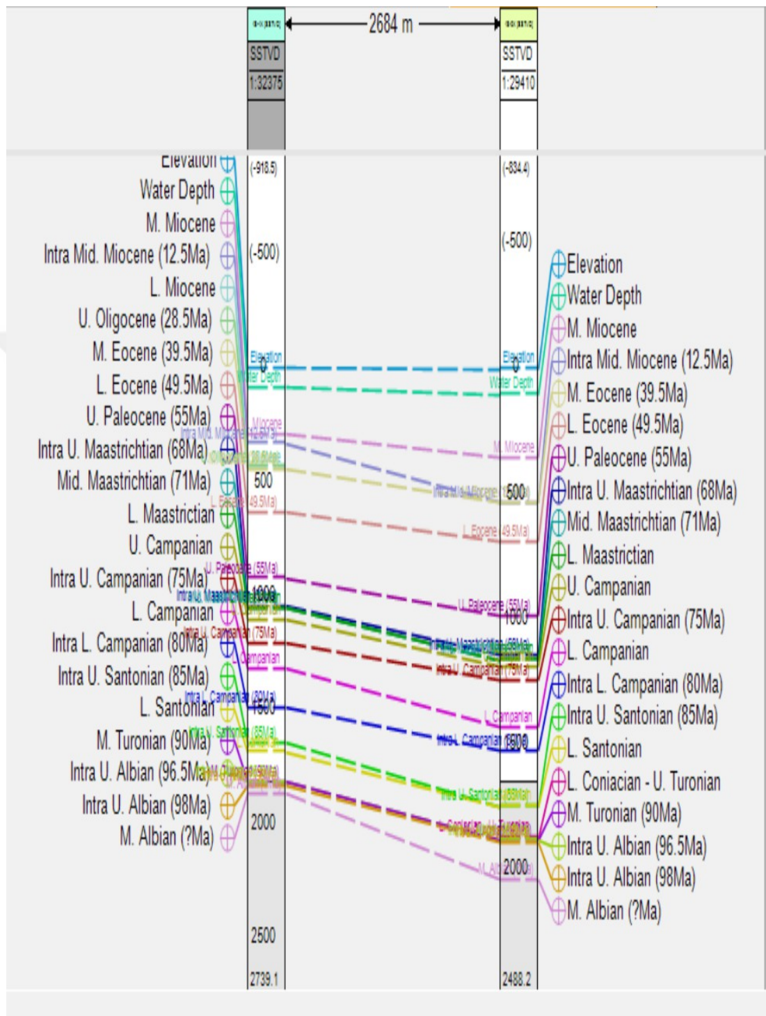
Figure 5.47. Well section window showing the depth of the wells from top to both (obtained from Fontem, 2019).
