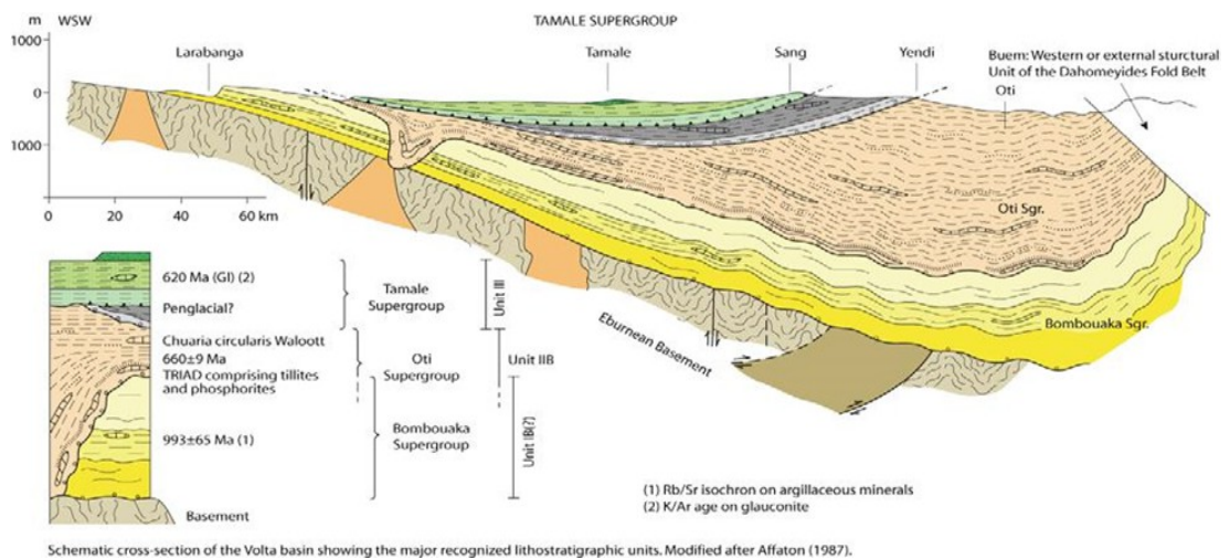
Figure 4.32. Cross-section of the Voltaian Basin in Ghana (modified by Affaton, 1990 as edited by Kalsbeek, 2008).
