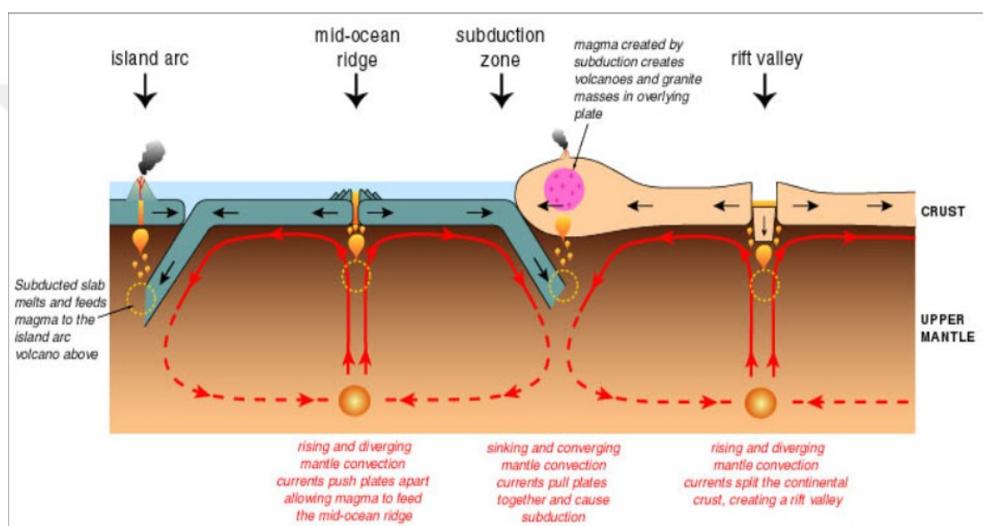
Figure 3.2. An illustration of the concept of plate tectonics theory ongoing on the earth's surface (Dar, 2013).
