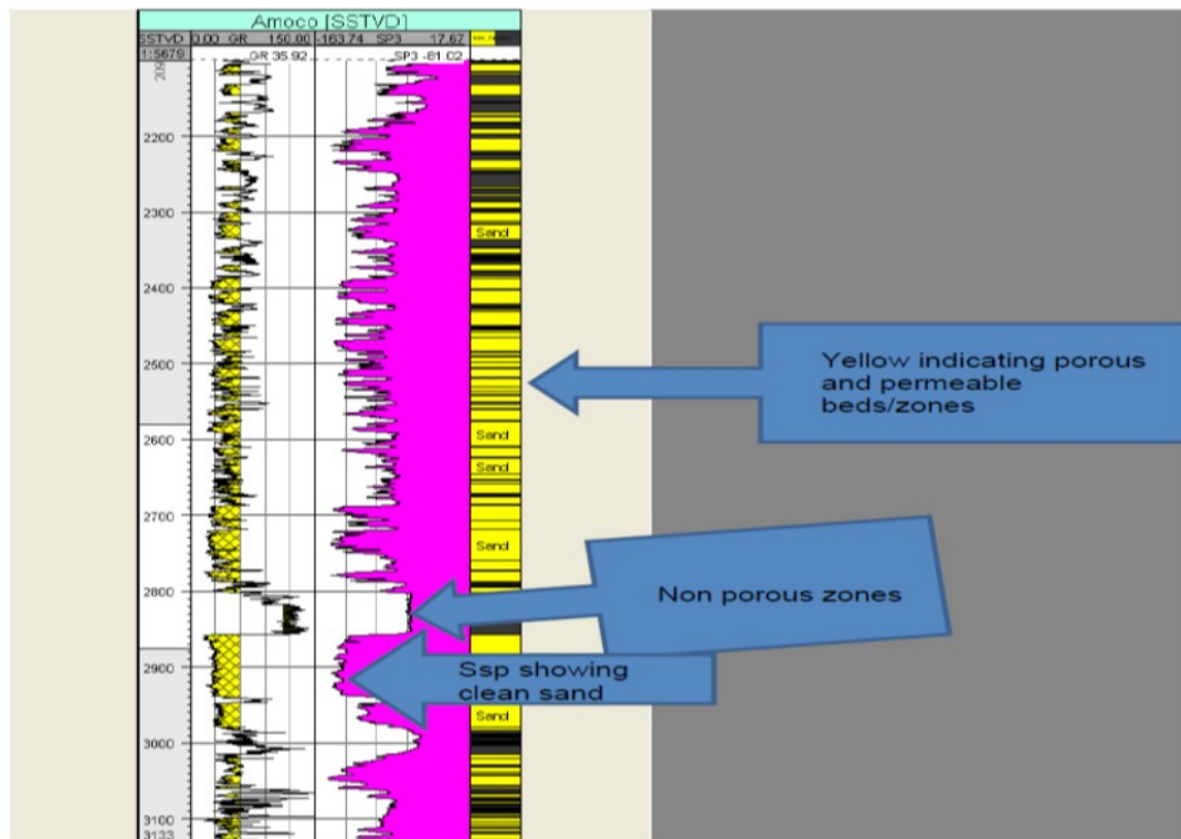
Figure 5.57. Well log of facies (Arku, 2012).
