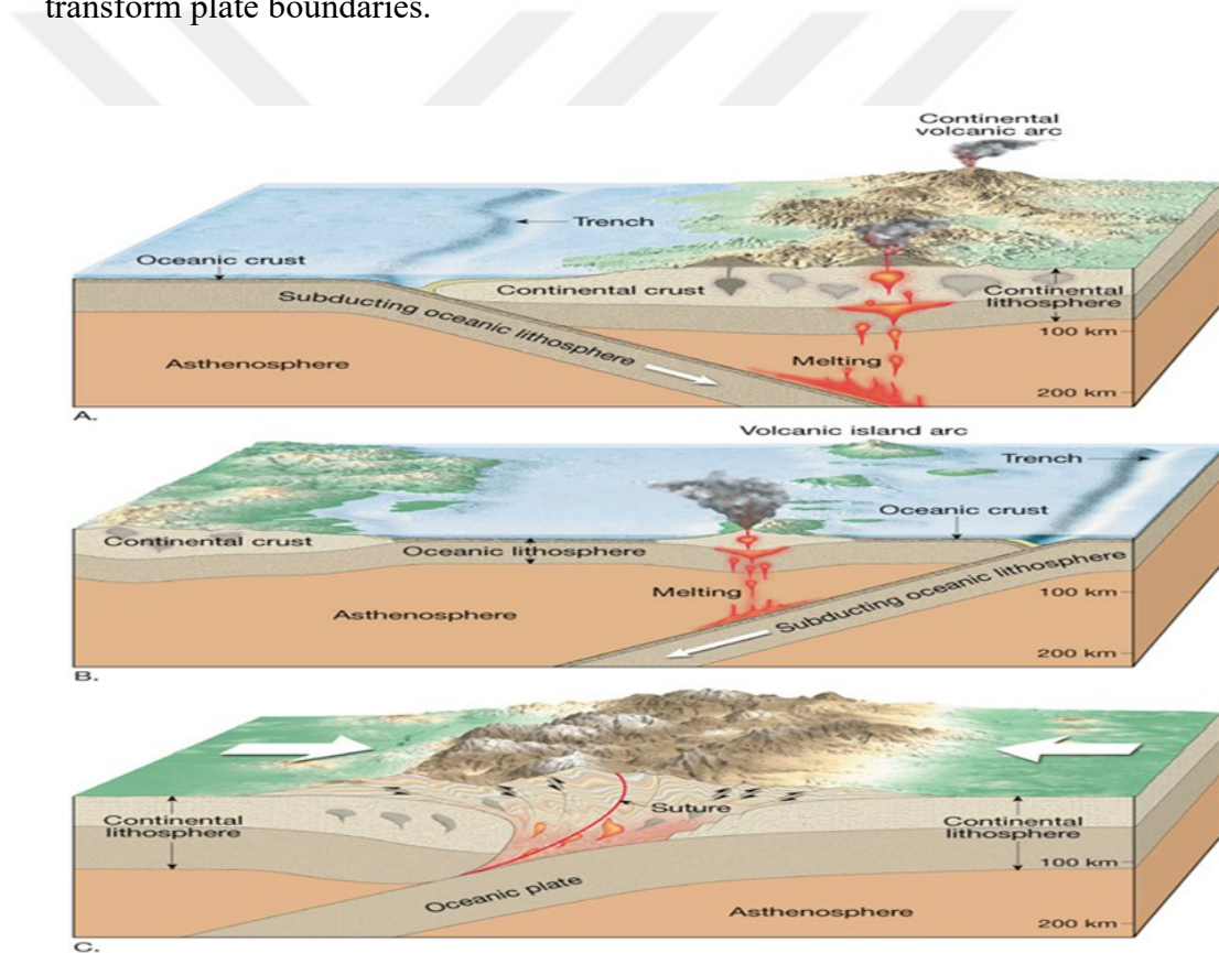
Figure 3.6. Types of convergent plate with the processes they undergo. A. Ocean-Continent. B. Ocean-Ocean and C. Continent-Continent convergent plate boundaries (Leyva, 2015).
