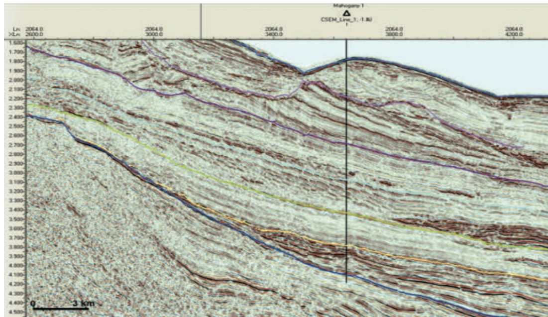
Figure 5.39. North-South line showing Mahogany 1 location and pinch out of Mahogany fan to the north, obtained from Dailly et al., 2017.
