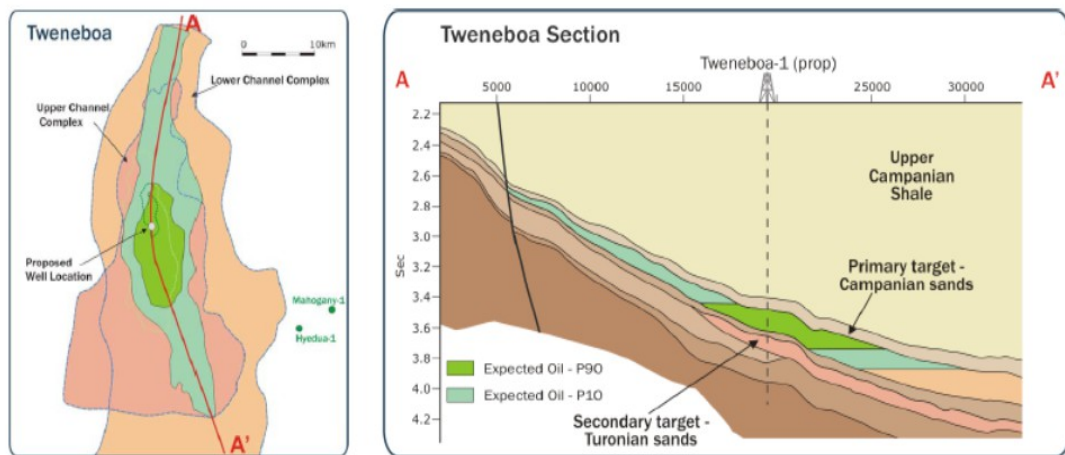
Figure 5.65. Tweneboa prospect of the Tano basin (Tullow oil, 2008).
