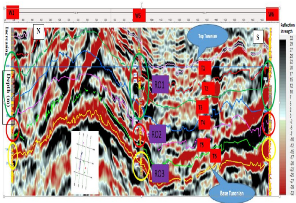
Figure 5.44. The behaviour of sands and shales units from Well to Seismic (EEI Data) tie and ISO-Proportional Intervals - A, obtained from Ablordeppey, 2016.
