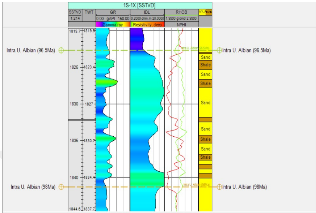
Figure 5.52. Combination of facies log, resistivity log and neutron density log to delineate reservoir zone (Obtained from Fontem, 2019).
