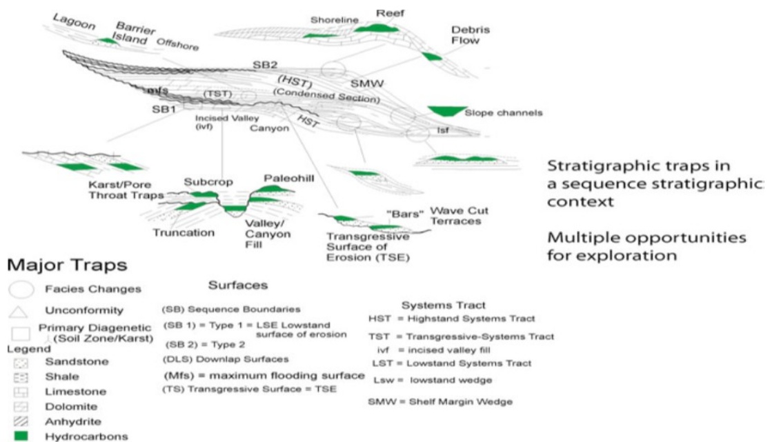
Figure 3.11. Common types of Stratigraphic traps found in various hydrocarbon systems (Modified from Dolson et al., 1999 in Dolson 2016).
