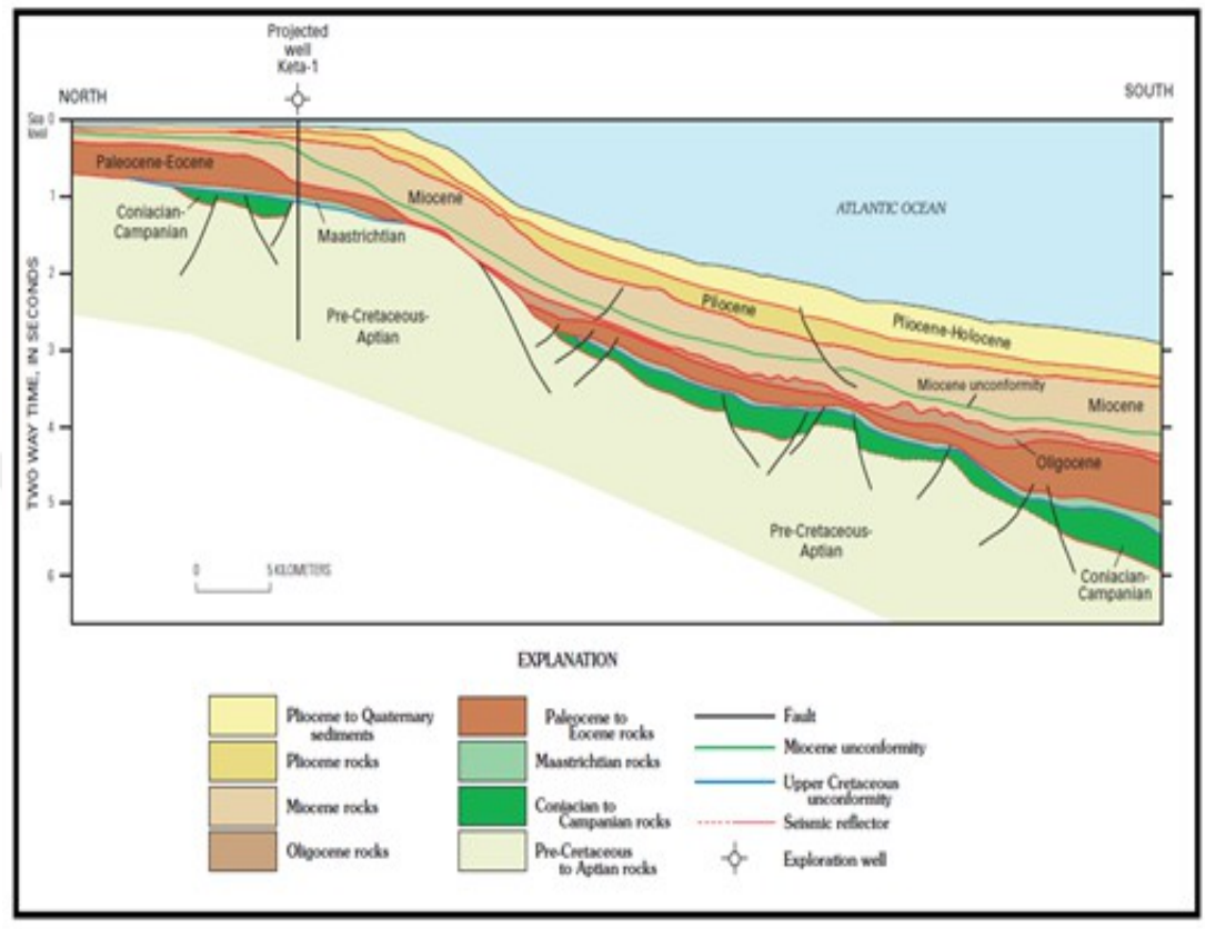
Figure 4.27. Cross-section of the Accra- Keta Basin in Ghana (Kjemperude et al., 1992 as cited by Brownfield, 2016).
