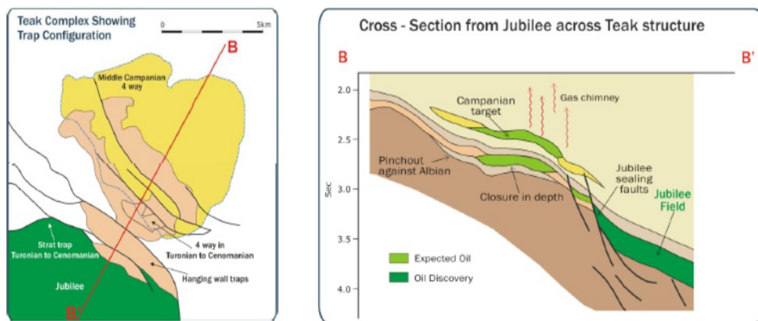
Figure 5.66. Teak prospect of the Tano basin (Tullow oil, 2008).
