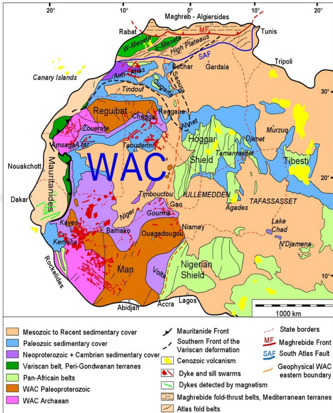
Figure 4.21. Regional Geology of the West Africa (Fabre, 2005; Liegeois et al., 2005; Ennih and Liegeois, 2008 as cited in Youbi, 2011).
