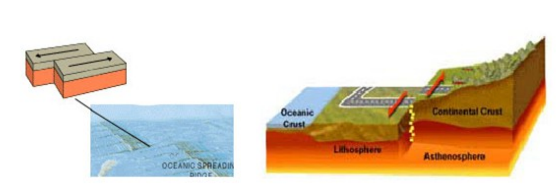
Figure 3.7. Figure 3.7. Transform plate boundary (Dar, 2013).
