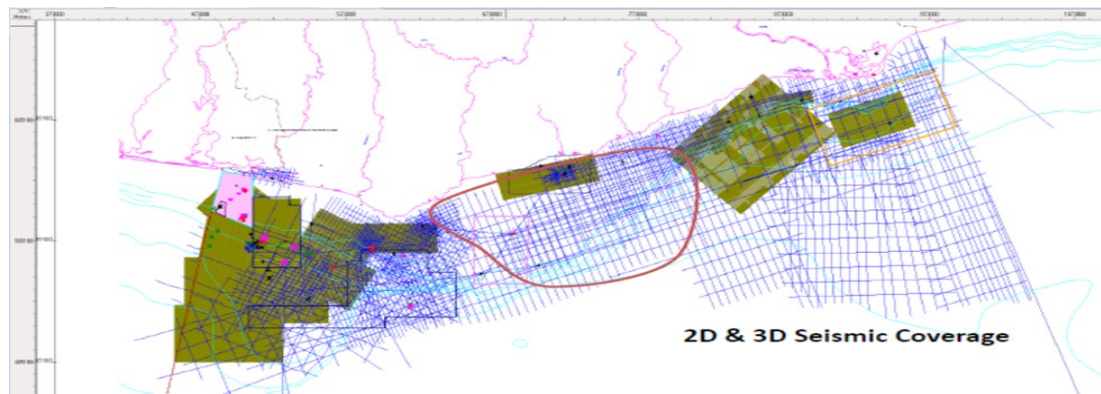
Figure 5.53. A 2D and 3D seismic survey data coverage of the Saltpond basin (Aryeetey, 2014).
