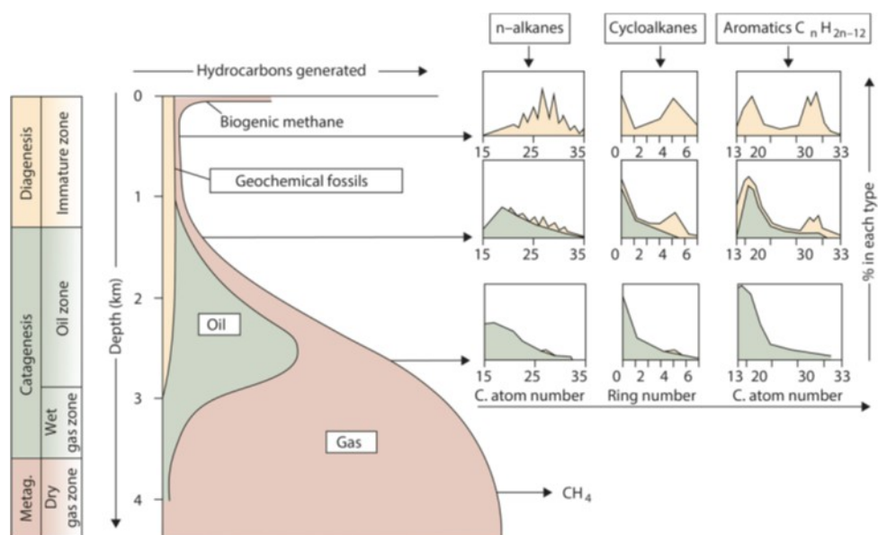
Figure 3.19. The stages of diagenesis, catagenesis and metagenesis (Abay, 2017).
