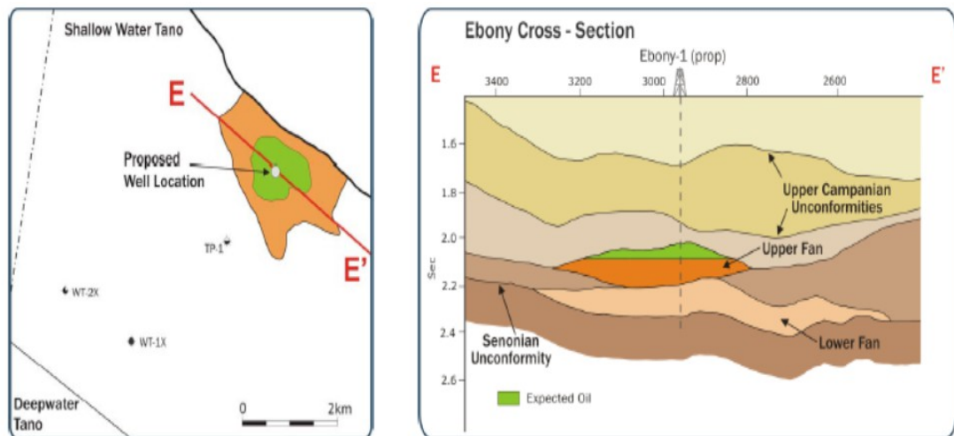
Figure 5.69. Ebony prospect of the Tano basin (Tullow oil, 2008).
