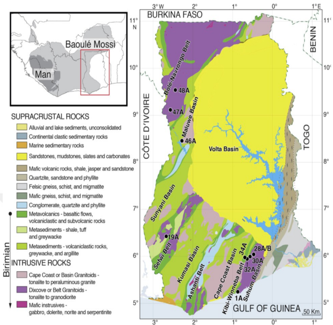
Figure 4.22. Geological provinces of Ghana (Peterson et al., 2008).
