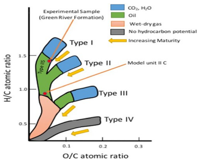
Figure 3.17. The four types of kerogens illustrated by Van Krevelen diagram (Type I, II, III and IV) with the associated products given off from kerogen (Pathak et al., 2017).
