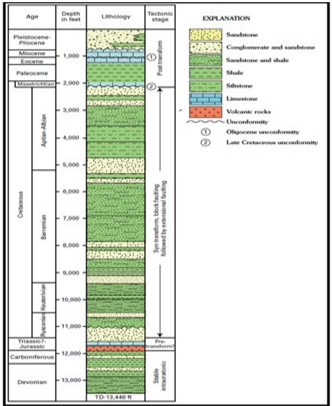
Figure 4.28. Stratigraphic section of the Keta Basin in Ghana (modified by Kjemperude et al., 1992 as cited by Brownfield, 2016).
