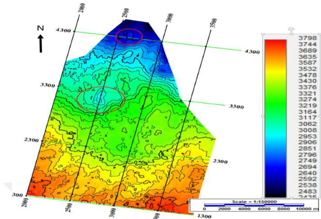
Figure 5.46. Structural map of the upper Santonian, obtained from Ablordeppey, 2016.
