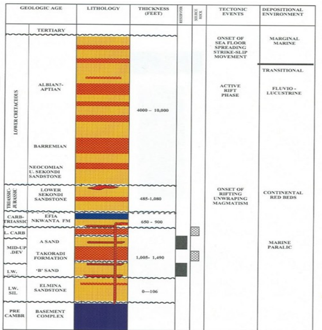
Figure 4.30. Stratigraphic section of the Saltpond- Central Basin in Ghana (Aryeetey, 2014).
