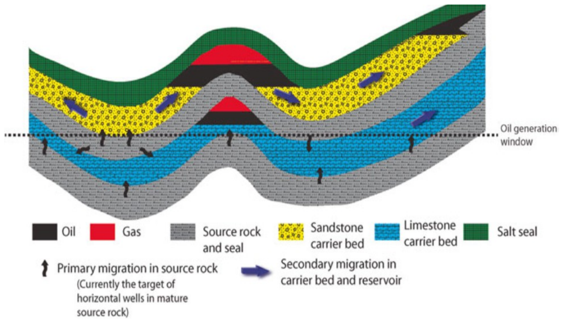
Figure 3.9. Migration pathways in a hydrocarbon system (Modified from England et al. 1991 as cited in Dolson, 2016).
