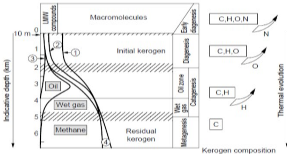
Figure 3.15. Hydrocarbon formation in stages from the breakdown of kerogens (Durand, 2003).
