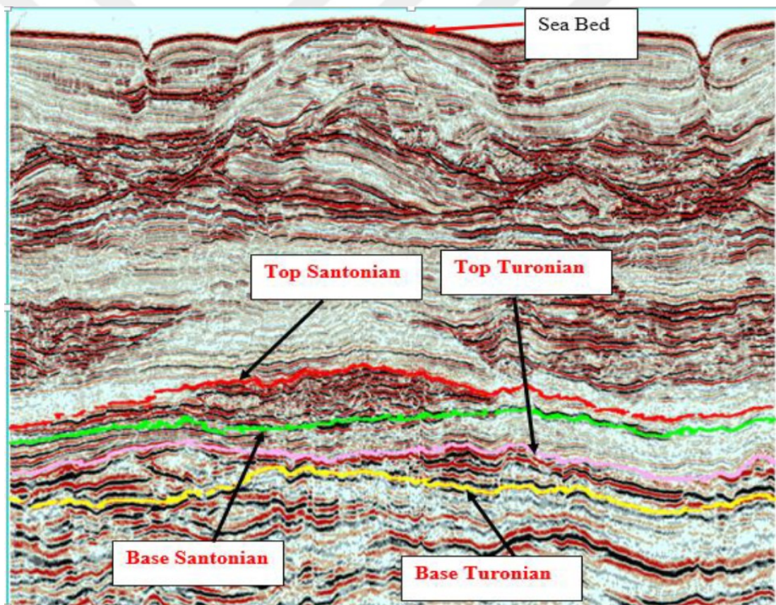
Figure 5.40. Mapped horizons of TEN field of the Santonian and Turonian, obtained from Ablordeppey, 2016.
