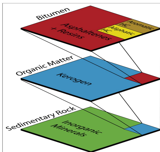
Figure 3.16. Stages of organic matter preservation in the source rock until the maturation stage where hydrocarbons are expelled (Abay, 2017).
