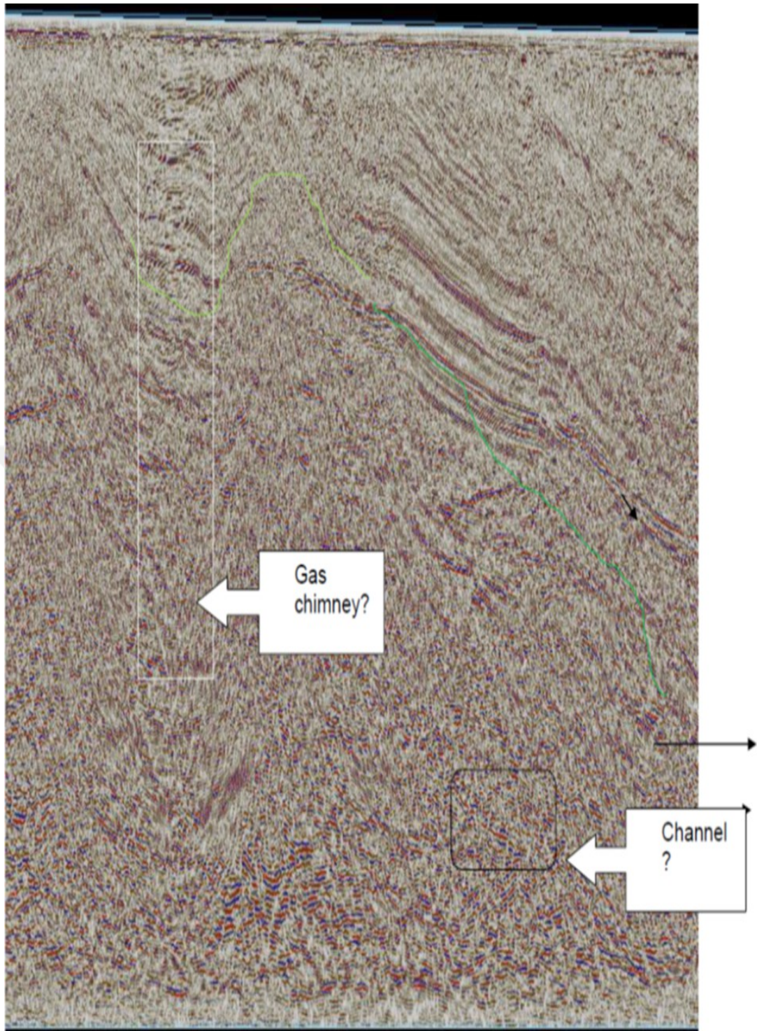
Figure 5.61. Gas chimneys and channel system of the horizons (Arku, 2012).
