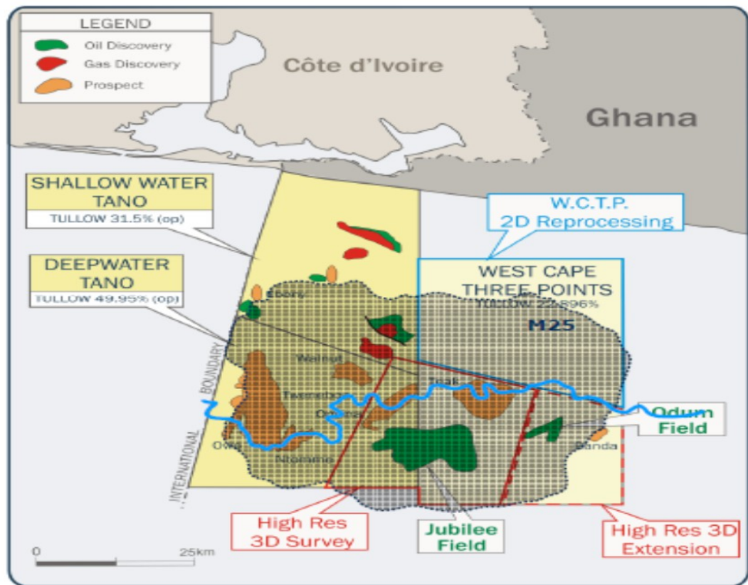
Figure 5.63. Map of the various potential prospects in the Tano basin (Tullow oil, 2008).
