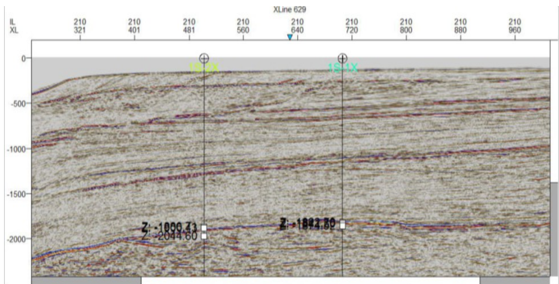
Figure 5.49. Seismic section delineating the major fault zones observed in the horizons (Fontem, 2019).
