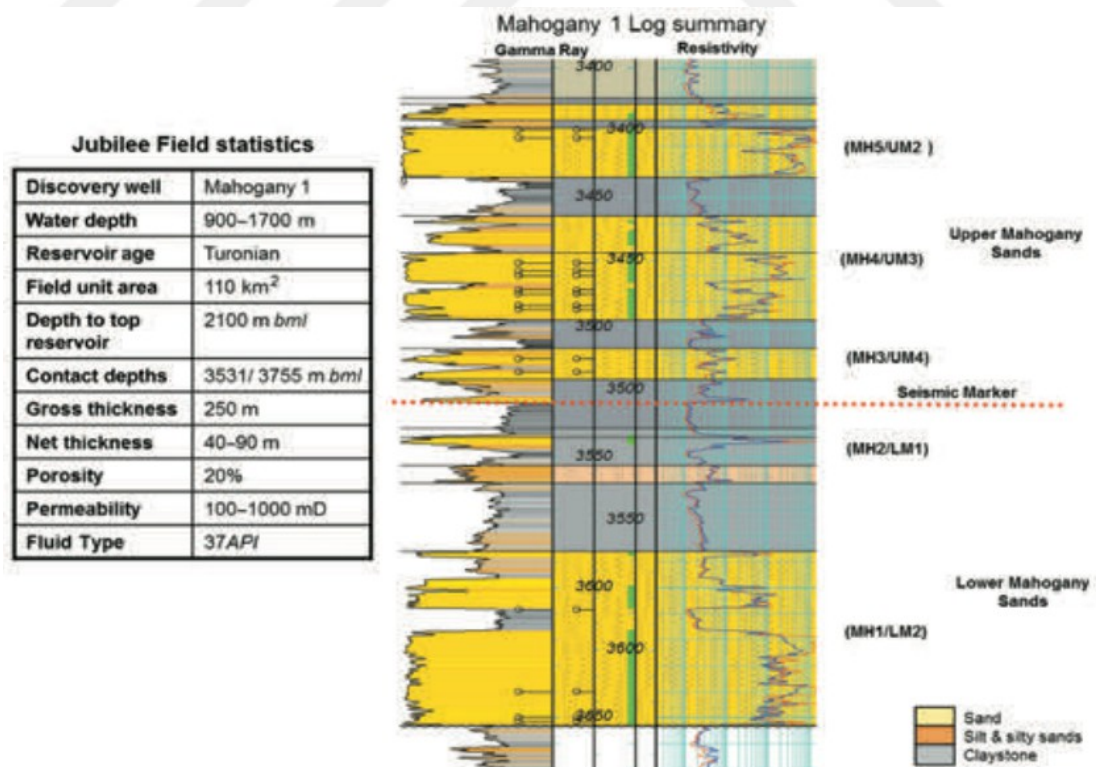
Figure 5.36. Well log summary of the Turonian section of the Mahogany-1 well, obtained from Dially et al., 2017.
