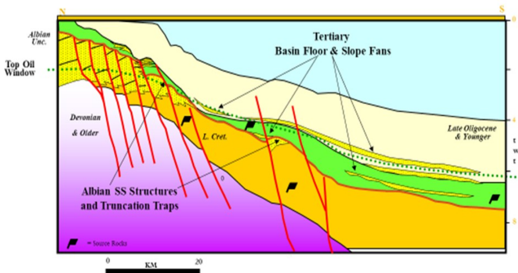
Figure 5.72. Cross section of the possible play systems in the Accra- Keta basin (Asiedu, 2012)
