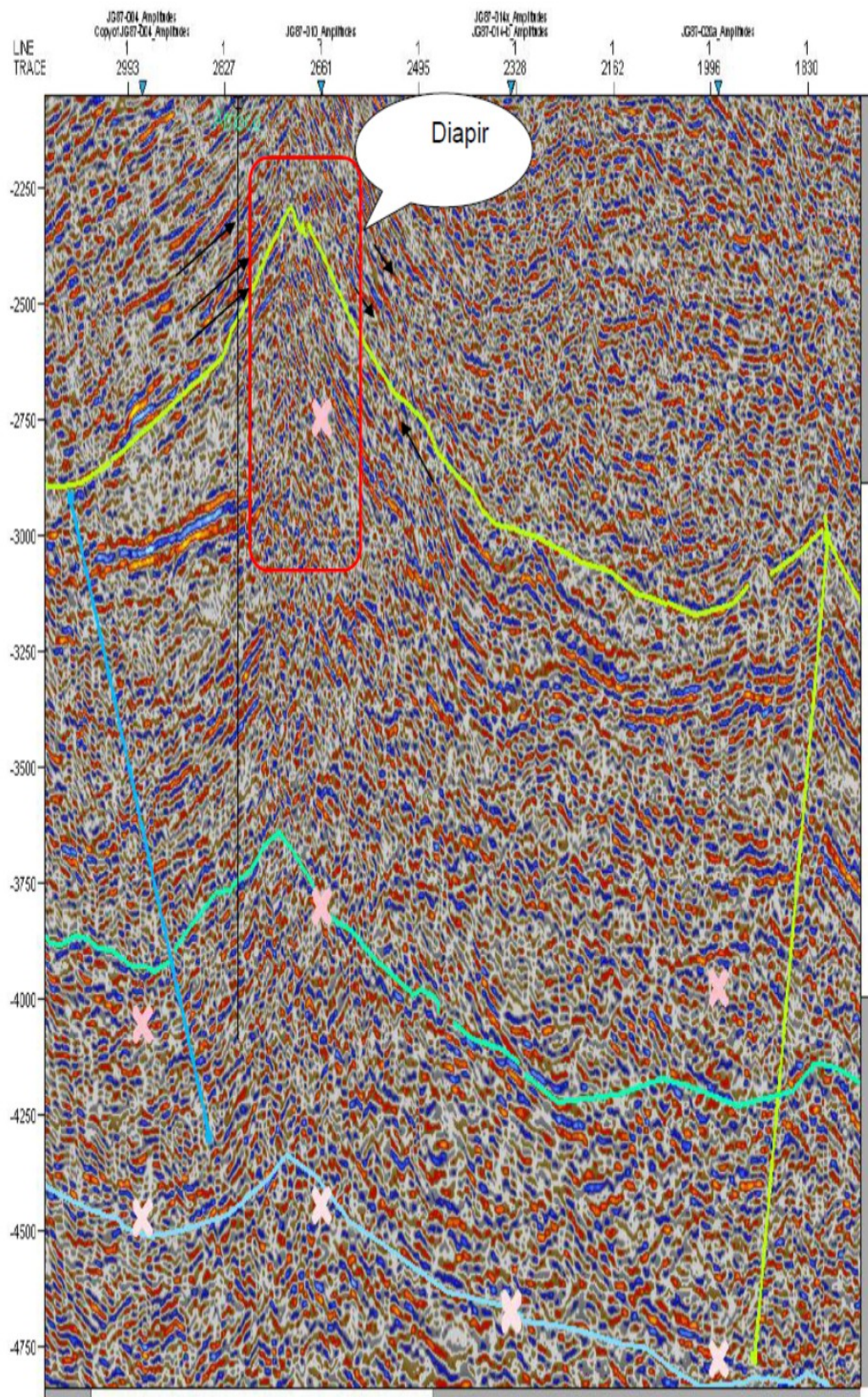
Figure 5.60. Seismic section of the horizons showing the various displacements and types of faults present (Arku, 2012).
