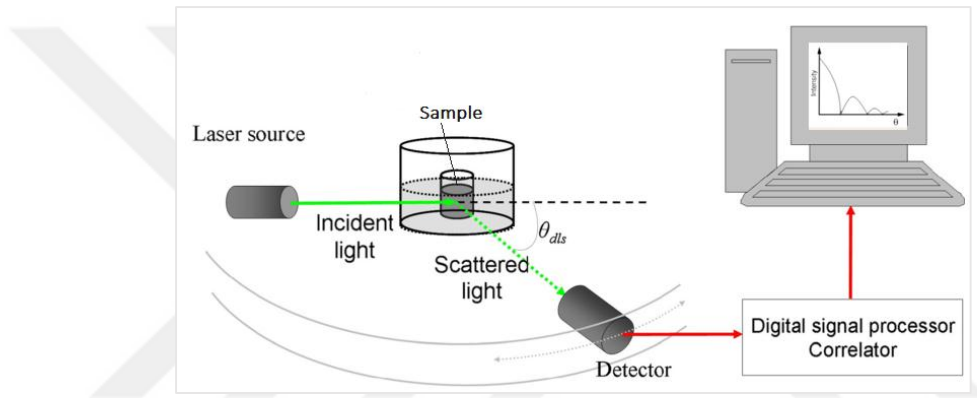
Figure 3.6. Block diagram of the dynamic light scattering measurements [73].
