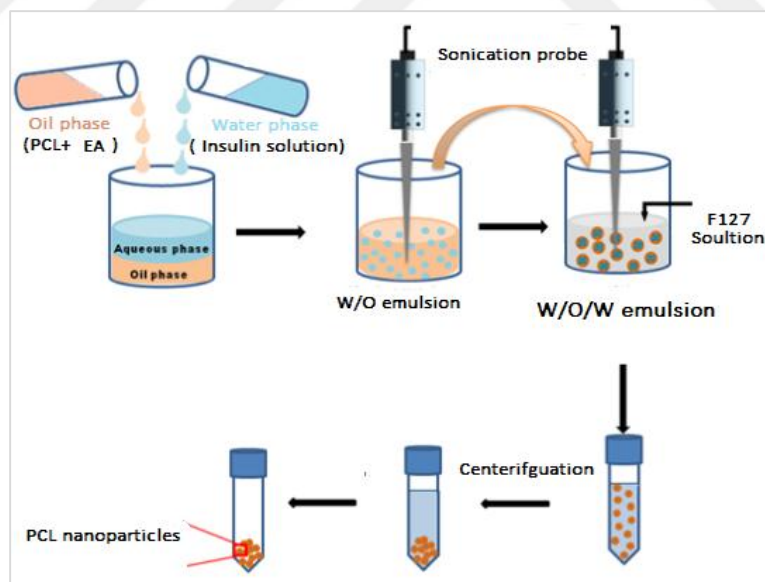
Figure 3.1. Preparation of the PCL nanoparticles using the double emulsion method.
