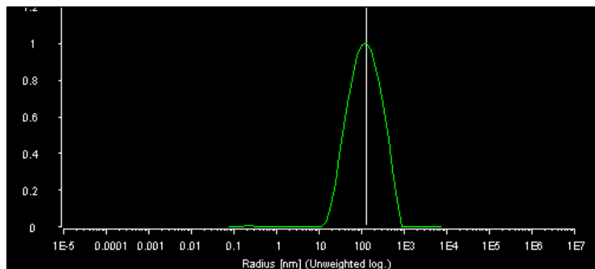
Figure 4.2. Dynamic light scattering image of PCL nanoparticles.
