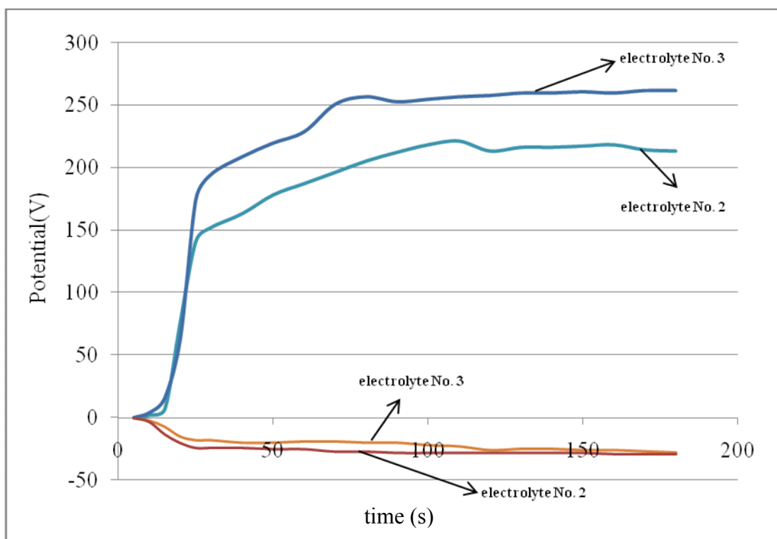
Figure 6.7 Potential variations of MgO coated samples as a function of time during MAO process run at 1 Amps for 3 minutes in electrolyte No.2 and No. 3.
