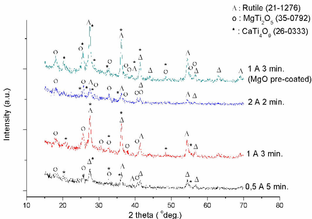
Figure 6.15 XRD analyses of electrolyte No. 3 group surfaces.
