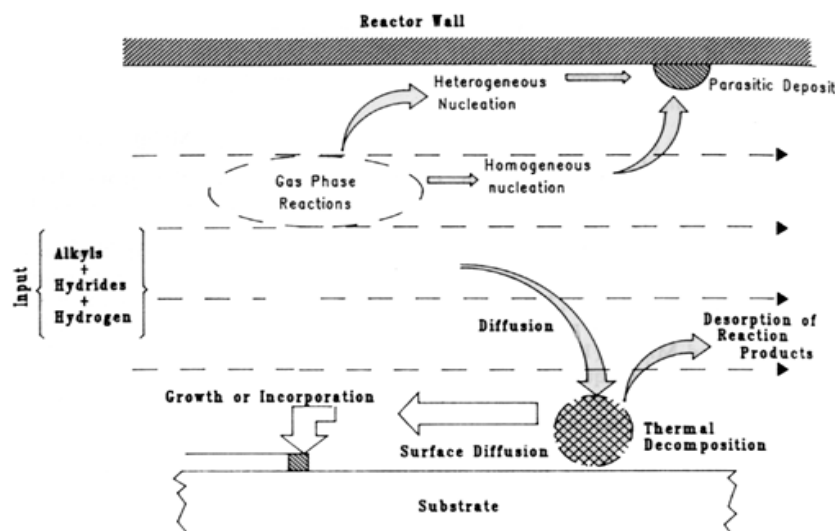
Figure 4.7 Principle of Chemical Vapor Deposition Process (Moon, Houn, 1993)
