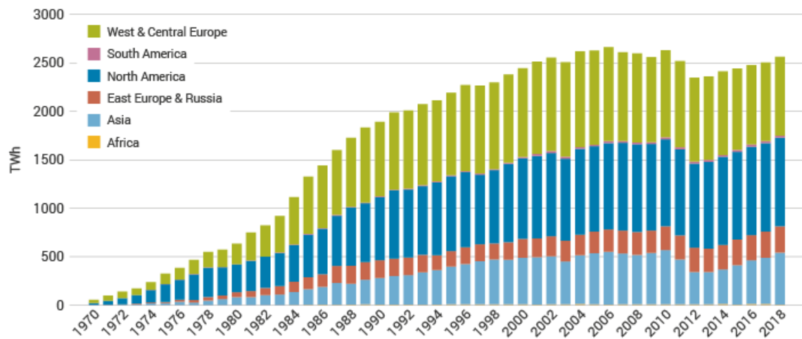
Graph 5. Nuclear Electricity Production of Continents
