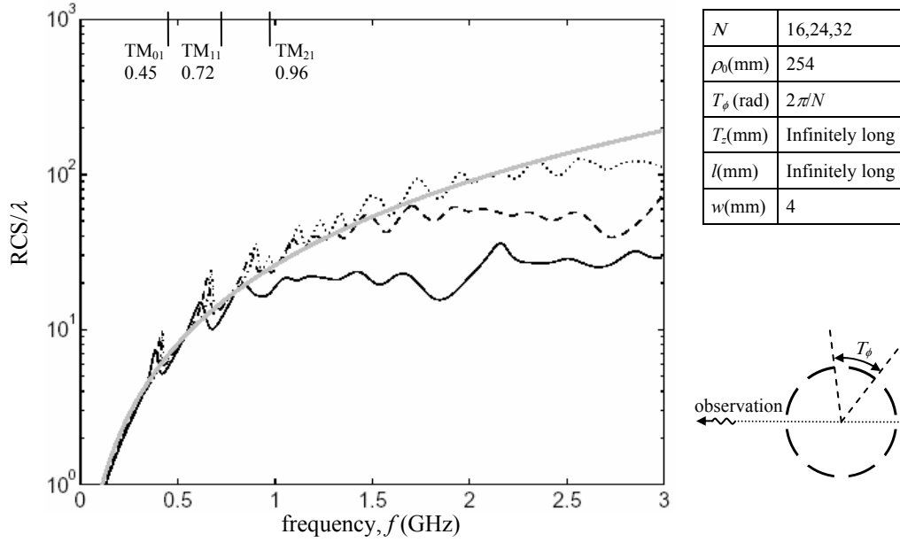
Figure 5.6 RCS versus frequency for free-standing and infinitely long strips. The number of elements ( N ) in the circumferential direction is varied. A TM plane wave is normally incident ( \phi^{inc}=0^\circ ) and the scattered fields are computed in the back side ( \phi=180^\circ ) of the structure.
