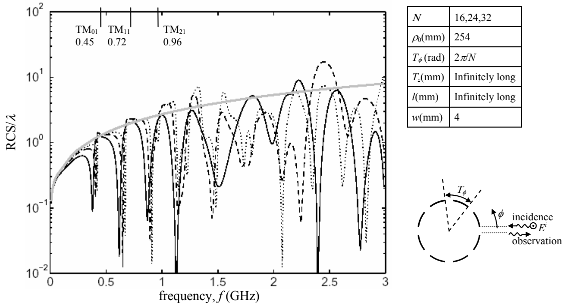
Figure 5.7 RCS of the structure considered in Figure 5.6 when the scattered fields are computed in the front side ( \phi=0^\circ ).
