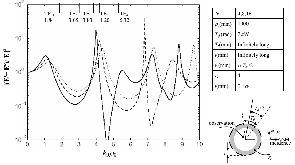
Figure 5.3 The field couplings at the origin versus the electrical length of the radius ( k_0\rho_0 ) for infinitely long strips located on a dielectric shell. The number of elements ( N ) in the circumferential direction is varied. The cylinder radius ( \rho_0 ) is kept constant. A TE plane wave is normally incident ( \phi^{inc}=0^0 ) and the scattered fields are computed at the origin ( \rho=0 ) of the cylindrical structure.
