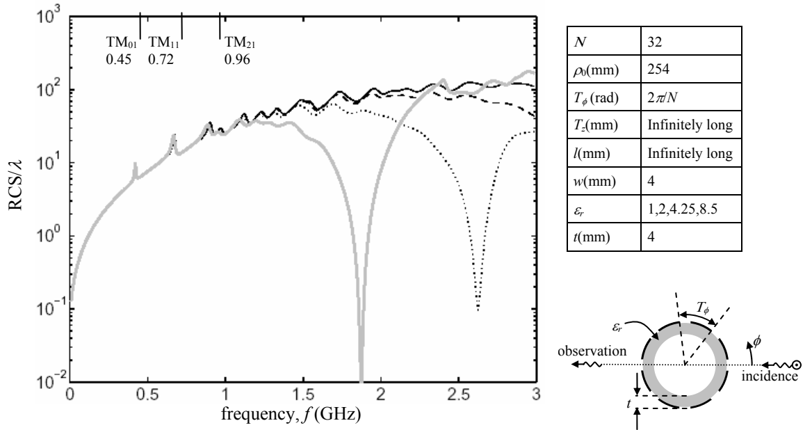
Figure 5.16 RCS versus frequency for infinitely long strips located on a dielectric shell. The relative dielectric constant ( \epsilon_r ) is varied and other parameters are as shown in the inset. A TM plane wave is normally incident ( \phi^{inc}=0^0 ) and the scattered fields are computed in the back side ( \phi=180^0 ) of the cylindrical structure.
