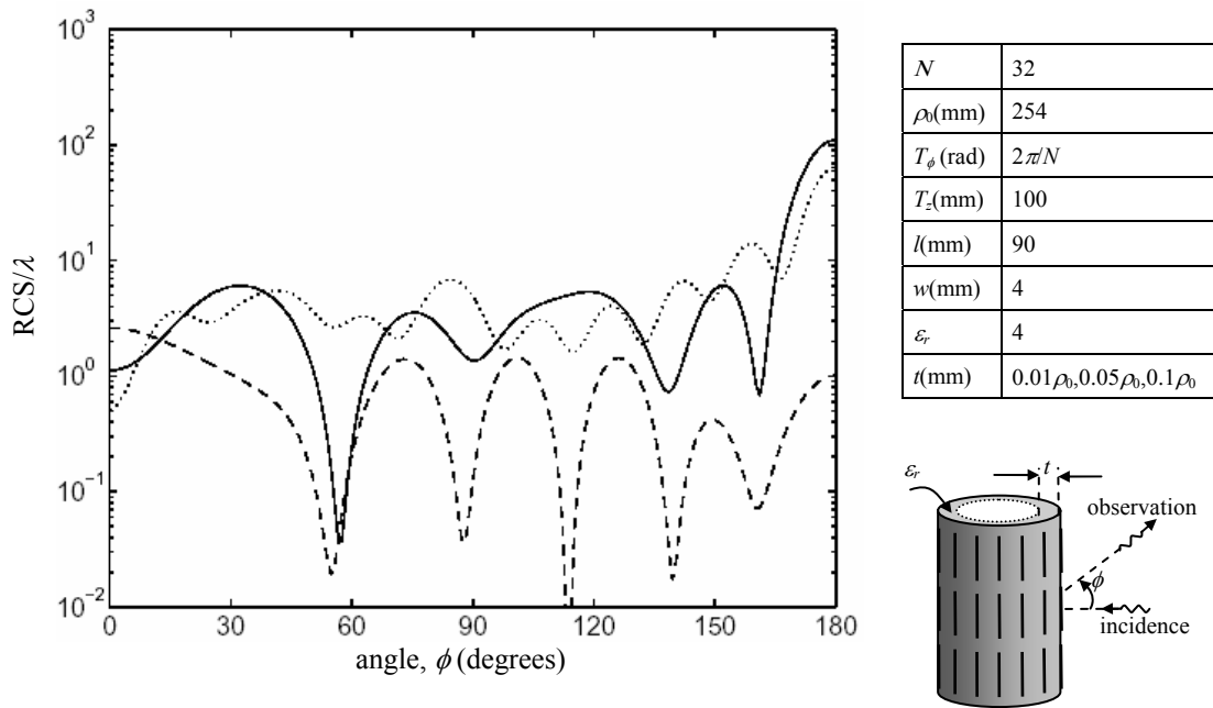
Figure 5.21 RCS versus observation angle ( \phi ) for rectangular strips located on a dielectric shell. The dielectric thickness ( t ) is varied. A TM plane wave is normally incident ( \phi^{inc}=0^\circ ) and the scattered fields are computed at the resonant frequency ( f=1.76\text{GHz} ) of Figure 5.18.
