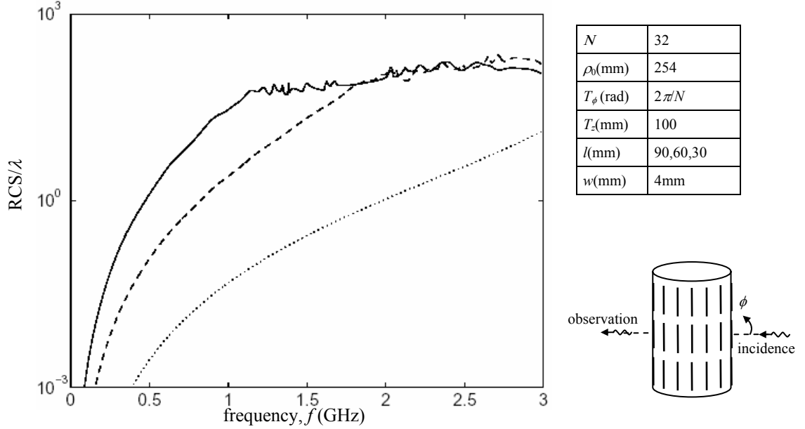
Figure 5.8 RCS versus frequency for free-standing rectangular strips. The length of strips ( l ) is varied and other parameters are as shown in the inset. A TM plane wave is normally incident ( \phi^{inc}=0^0 ) and the scattered fields are computed in the back side ( \phi=180^0 ) of the cylindrical structure.
