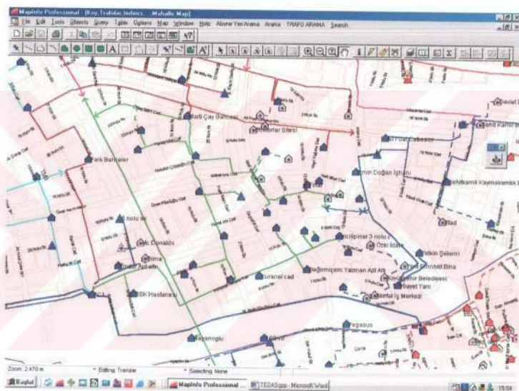
Figure 4.19 Transformer layer
