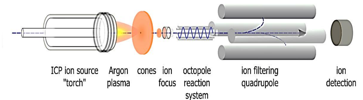
Figure 3.8. Schematic diagram of ICP-MS/MS, showing major components of the instrument
