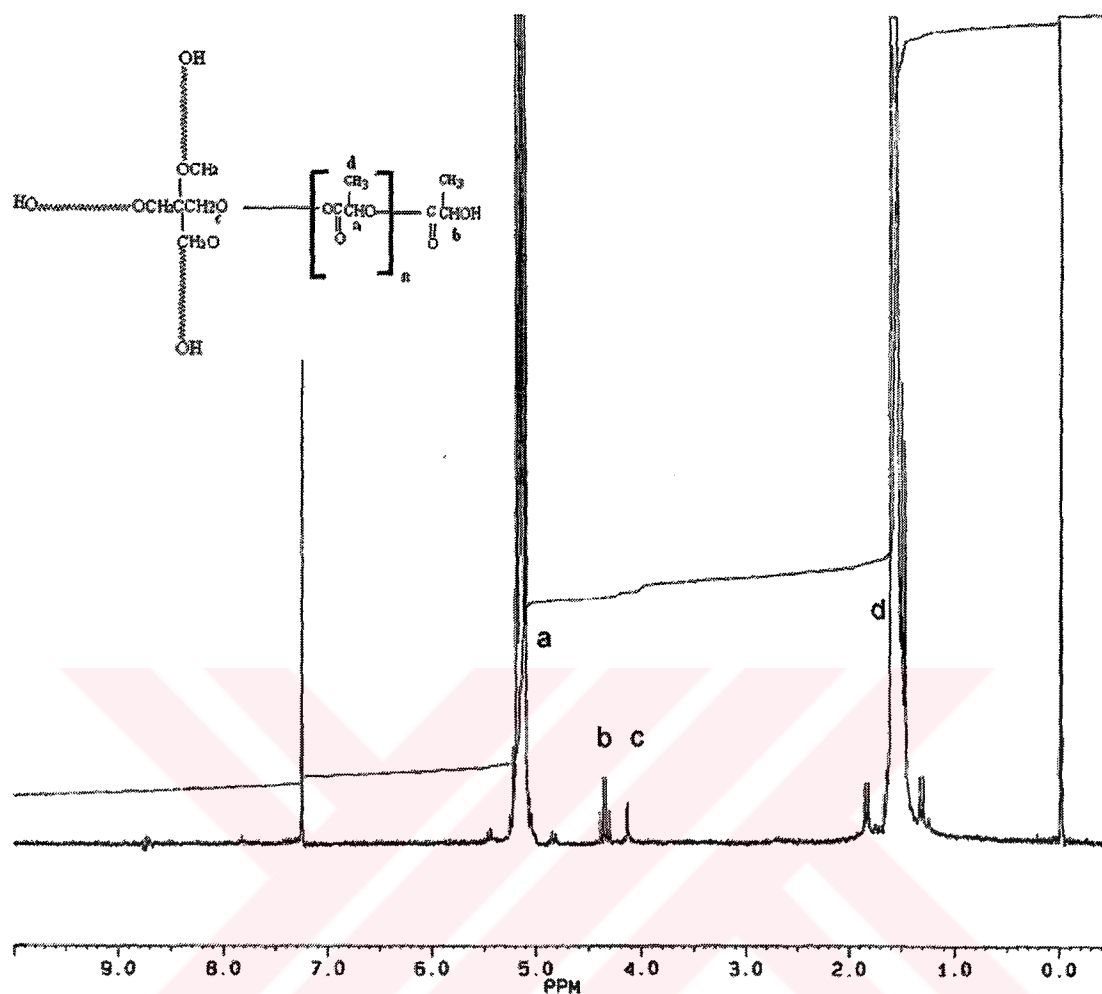
Figure 4.6: ^1\text{H} -NMR Spectrum of 4-armed OH-PL.
