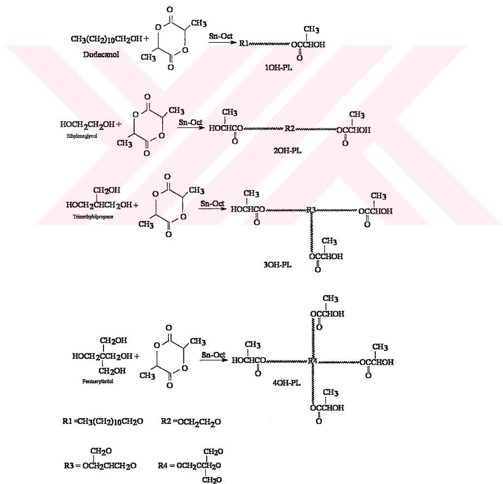
Figure 4.1: Synthesis of 1, 2, 3 and 4-armed OH-PL.
