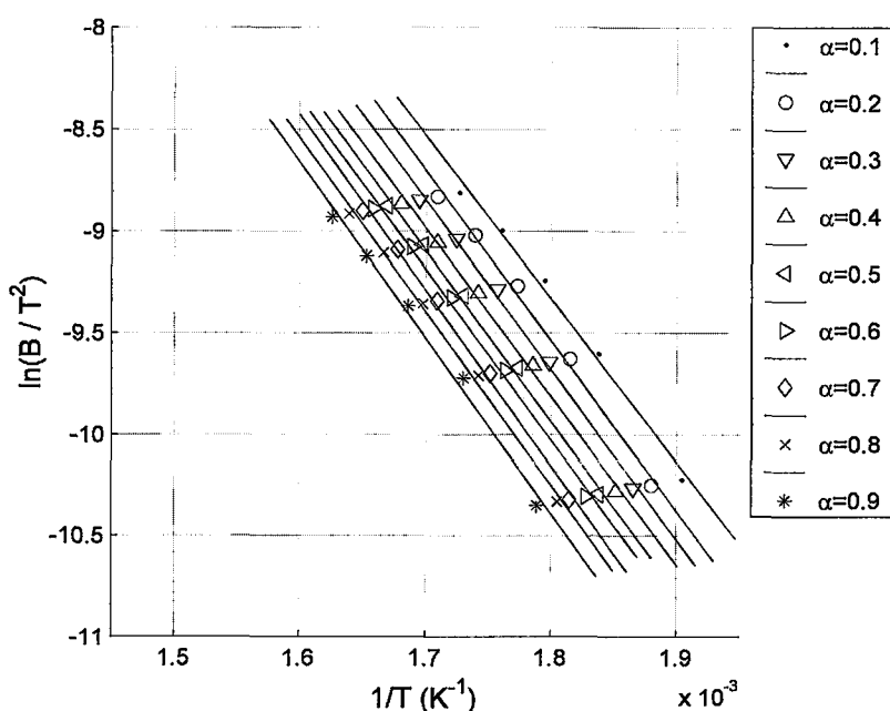
Figure 4.23: Reich plots of 4-armed OH-PL at varied fractions of degradation, \alpha = 0.9 to 0.1
