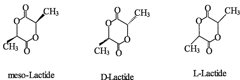
Figure 1.2: Structure of D-, L- and meso-lactide.
