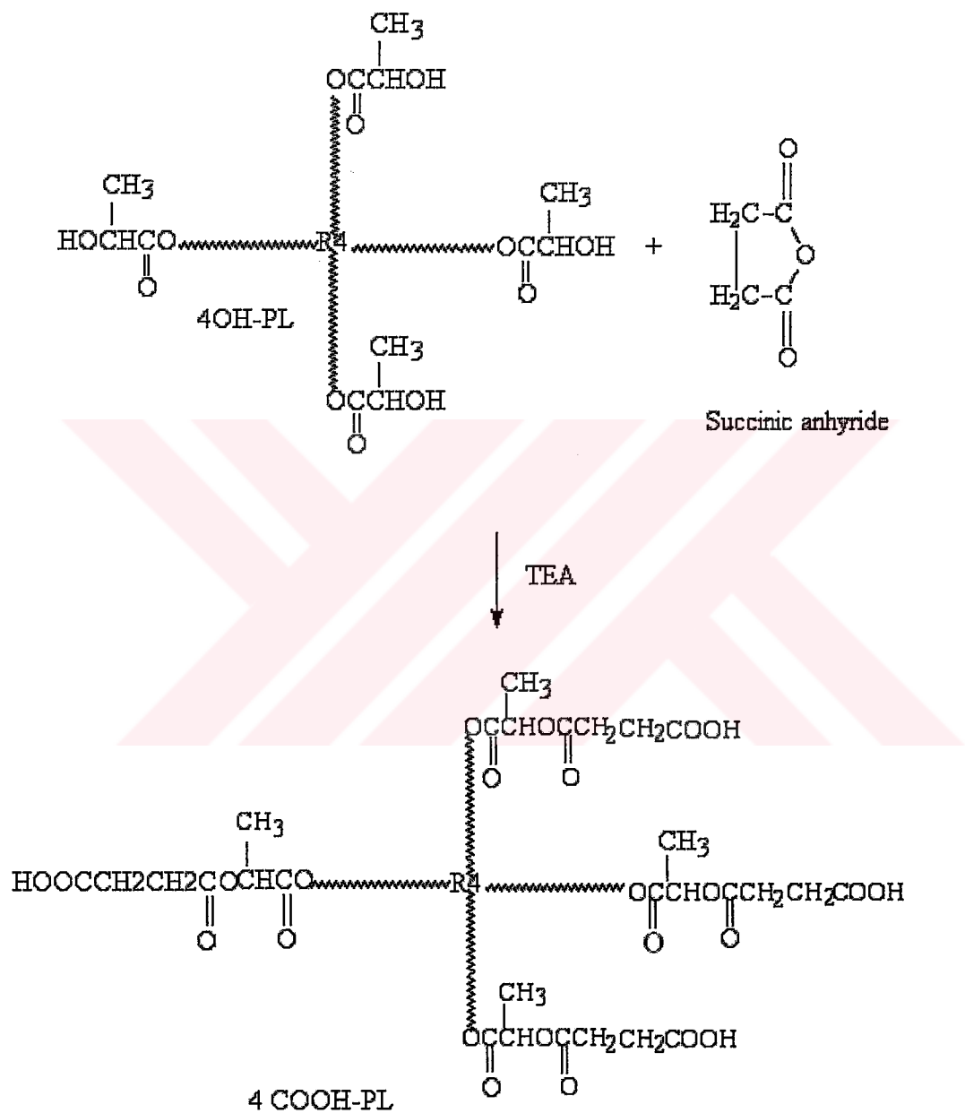
Figure 4.2: Acid modification reaction of 4-armed OH-PL to 4-armed COOH-PL.
