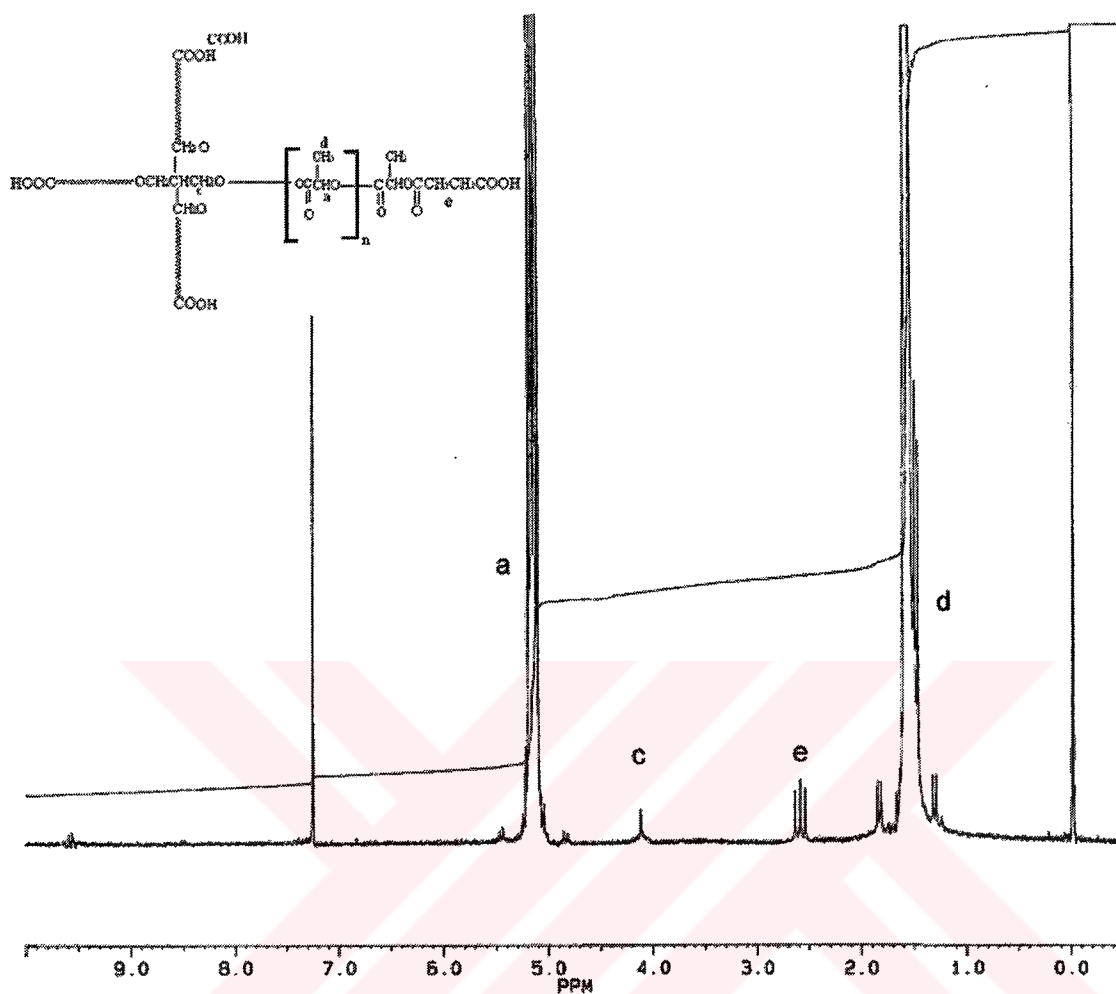
Figure 4.10: ^1\text{H} -NMR Spectrum of 4-armed COOH-PL.
