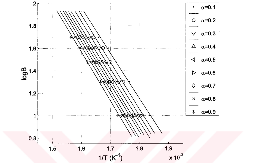
Figure 4.16: Ozawa plots of 1-armed OH-PL at varied fractions of degradation, \alpha = 0.9 to 0.1
