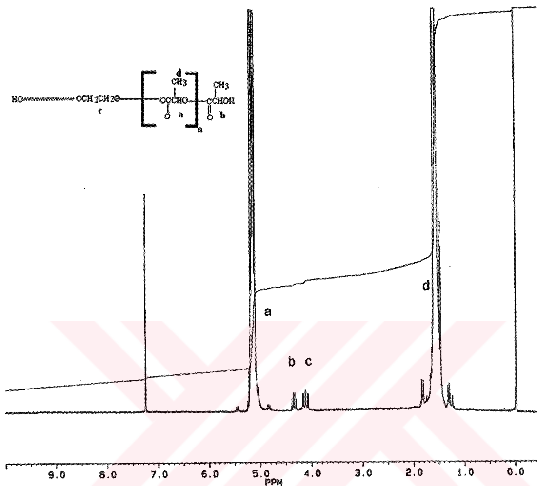
Figure 4.4: ^1\text{H} -NMR Spectrum of 2-armed OH-PL.
