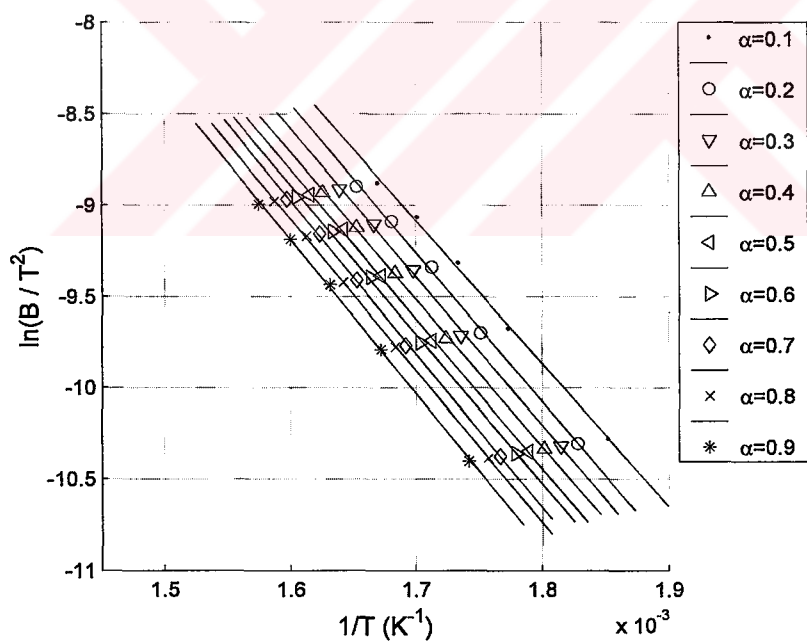
Figure 4.37: Reich plots of 4-armed COOH-PL at varied fractions of degradation, \alpha = 0.9 to 0.1
