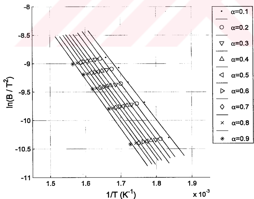
Figure 4.20: Reich plots of 1-armed OH-PL at varied fractions of degradation, \alpha = 0.9 to 0.1
