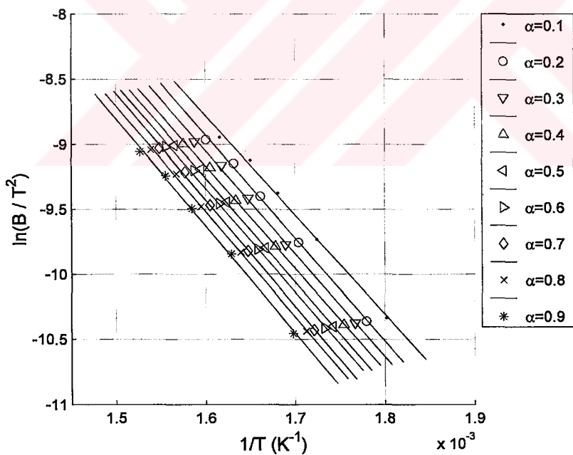
Figure 4.35: Reich plots of 2-armed COOH-PL at varied fractions of degradation, \alpha = 0.9 to 0.1
