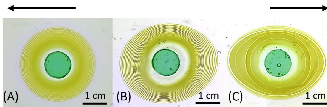
Figure 39. Comparison of different stress-release cycle with different time intervals after 6 hours while stretched. A) at constant stress, B) with 3 hour interval, C) with 2 hour interval. Arrows show the direction of applied mechanical stress. Elongation percentages were 40% for all of them.
