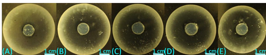
Figure 17. Change of precipitation patterns due to change of acrylamide concentration at constant inner electrolyte (magnesium ion) concentration 0.07 M and at constant outer electrolyte (hydroxide ion) concentration 2 M and at acrylamide concentrations: (A) = 5.49 % , (B) = 6.77 % , (C) = 8.01 % , (D) = 9.23 % , (E) = 10.41 %; alginate = 1.04%; BIS = 0.01 %; TEMED = 0.1 %; KPS = 0.25 %; (T= 21 °C).
