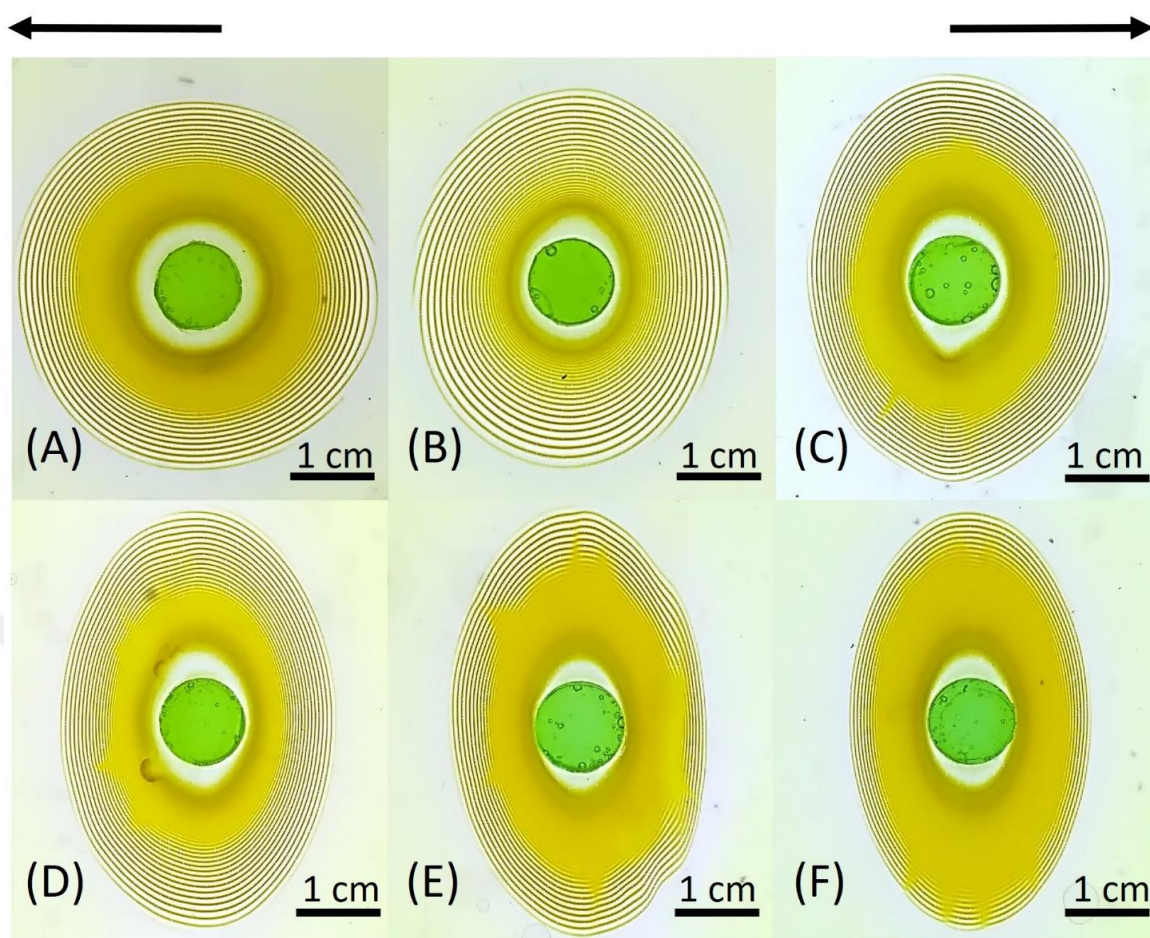
Figure 30. Liesegang patterns immediately after release of mechanical stress. A) 0 % percentage elongation, B) 10 % percentage elongation, C) 20 % percentage elongation, D) 30 % percentage elongation, E) 40 % percentage elongation, F) 50 % percentage elongation. Arrows show the direction of applied mechanical stress. Concentrations of components are as follows: inner electrolyte (chromate ion) = 0.01 M, outer electrolyte (copper (II) ion) = 1 M, acrylamide = 13.5 w%, BIS = 0.056 w%, KPS = 0.187 w%, TEMED = 0.0001 w%. T= 20 °C.
