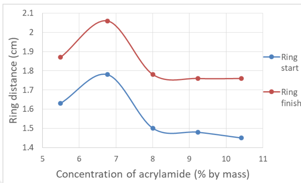
Figure 18. Calculated precipitation pattern distances as a function of acrylamide concentration.
