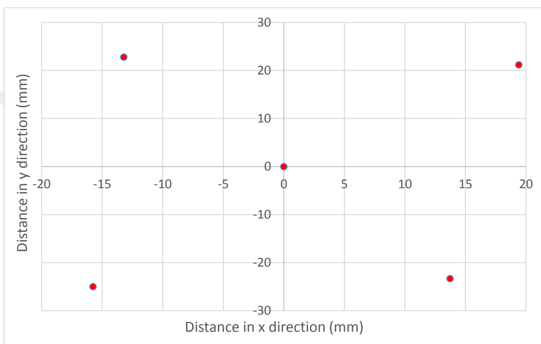
Figure 36. Setup for determining local elastic deformation by placing stamps to different positions. A) Pattern formation after 24 hours of applying stress, and B) immediate release of mechanical stress C) Positions of the stamps in the Cartesian coordinate while it is released from the stress (dots show the centers of the stamps and the origin is the stamp in the center. X direction is direction of applied stress and y direction is the perpendicular direction). Arrows show the direction of applied mechanical stress. Numbers shown on the stamps gives aspect ratios. Concentrations of components as follows: inner electrolyte (chromate ion) = 0.01 M, outer electrolyte (copper (II) ion) = 1 M, acrylamide = 13.5 w%, BIS = 0.056 w%, KPS = 0.187 w%, TEMED = 0.0001 w%. T = 20 °C.
