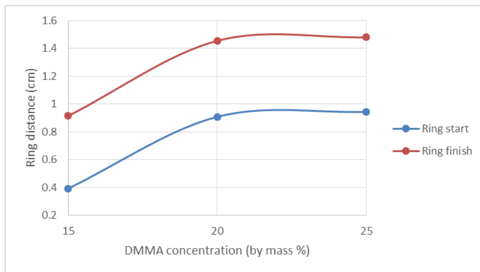
Figure 22. Calculated precipitation pattern distances as a function of DMMA concentration.
