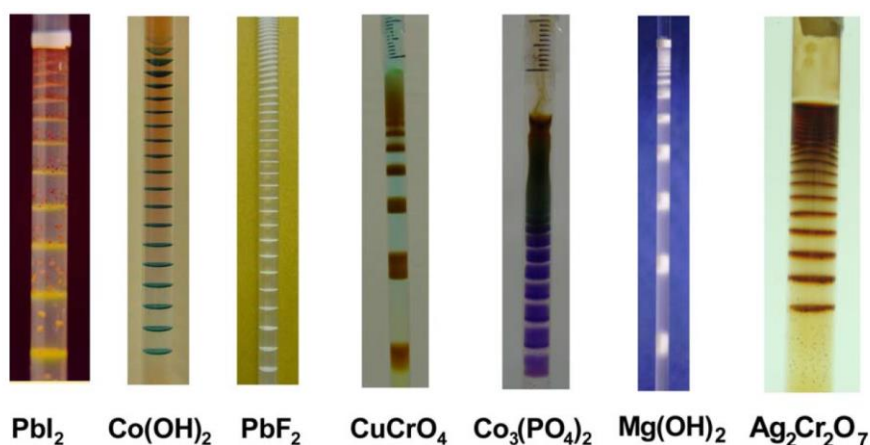
Figure 1. Liesegang band patterns in gels, for a number of sparingly soluble salts [1]
