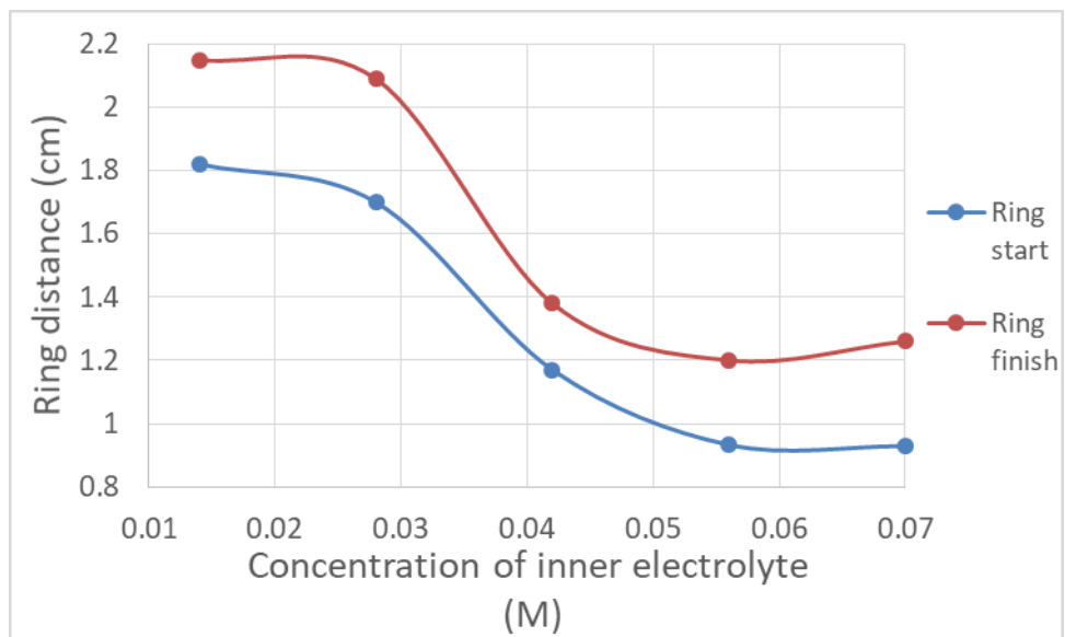
Figure 14. Calculated precipitation pattern distances as a function of inner electrolyte concentration.
