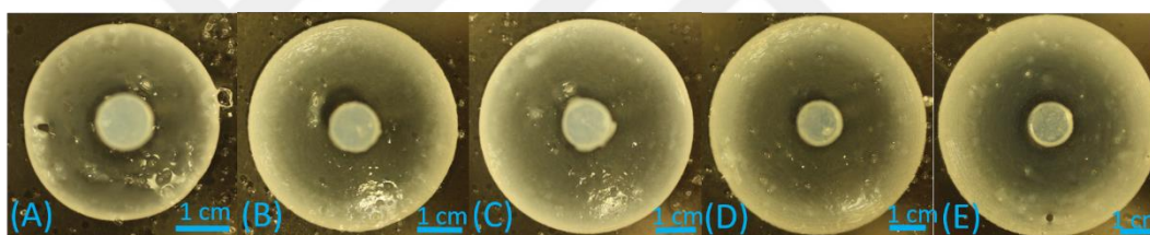
Figure 15. Change of precipitation patterns due to change of outer electrolyte concentration at constant inner electrolyte (magnesium ion) concentration 0.07 M and at outer electrolyte (hydroxide ion) concentrations : (A) = 2 M, (B) = 3 M, (C) = 4 M, (D) = 5 M, (E) = 6 M; acrylamide = 12.22 %; alginate = 1.53 %; BIS = 0.01 %; TEMED = 0.085 %; KPS = 0.25 %; (T= 20 °C).
