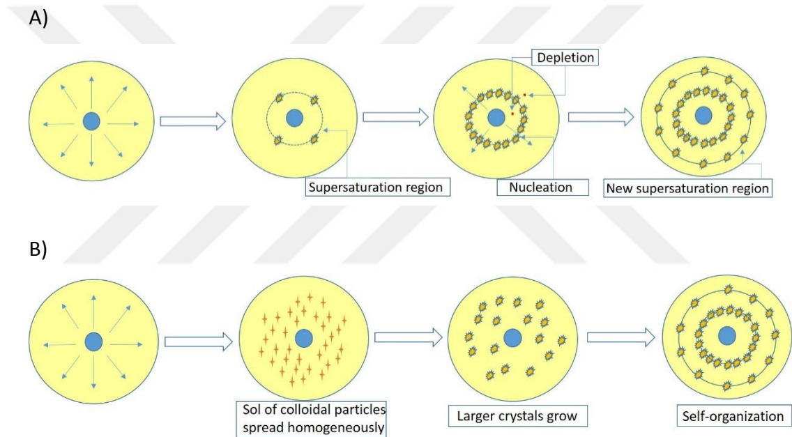
Figure 3. Theoretical models of LP formation. A) The “prenucleation” model, B) The “postnucleation” model
