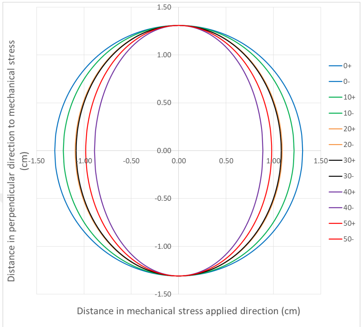
Figure 26. Precipitation patterns shapes at different percent elongations. The distances in the direction perpendicular to the applied stress is normalized to the same value to display the deviations from perfect circle (unstretched).
