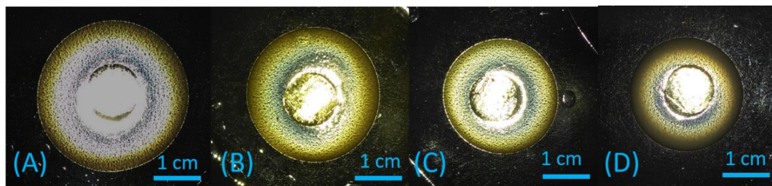
Figure 23. Precipitation patterns in DMMA gels at inner concentration (magnesium ion concentration) of: (A) 0.146 M, (B) 0.171 M, (C) 0.195 M, and (D) 0.220 M. Outer electrolyte concentration (hydroxide ion) is 3 M. Concentration of gel is 20 % by mass of DMAA. Concentrations of KPS is 0.85 % by mass and TEMED is 0.0001 % by mass. (T= 21 °C).
