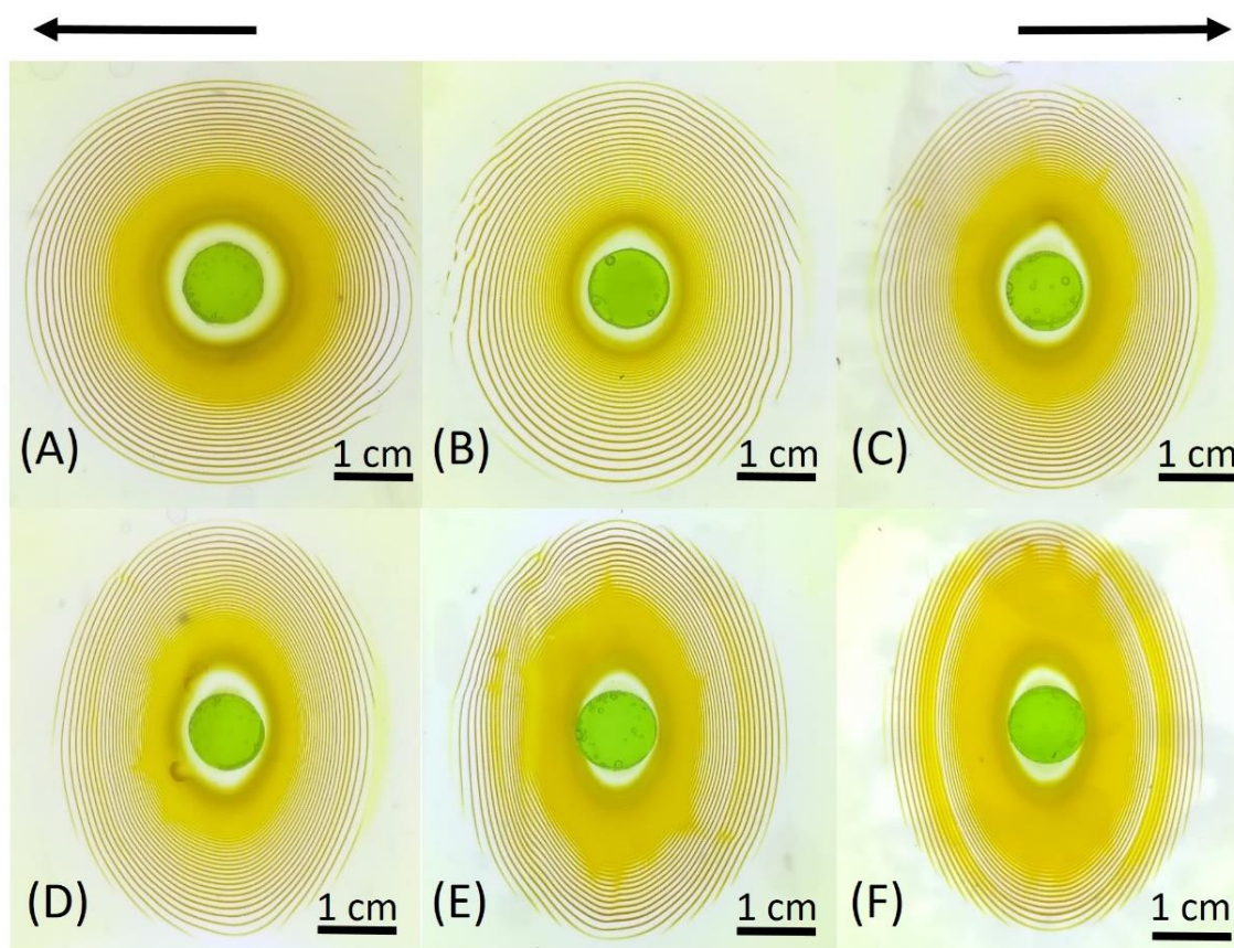
Figure 33. Patterns formed 18 hours (42 hours from the beginning) after release of the stress (Post rings). A) 0 % percentage elongation, B) 10 % percentage elongation, C) 20 % percentage elongation, D) 30 % percentage elongation, E) 40 % percentage elongation, F) 50 % percentage elongation. Arrows show the direction of applied mechanical stress. Concentrations of the components are as follows: inner electrolyte (chromate ion) = 0.01 M, outer electrolyte (copper (II) ion) = 1 M, acrylamide = 13.5 w%, BIS = 0.056 w%, KPS = 0.187 w%, TEMED = 0.0001 w%. T= 20 °C.
