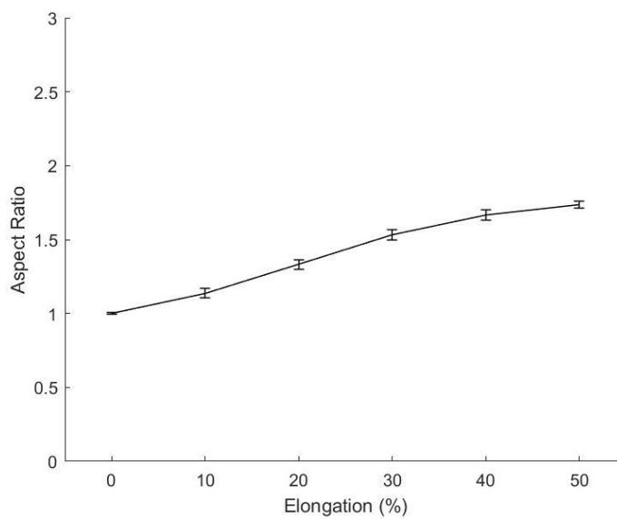
Figure 32. Aspect ratios of patterns obtained immediately after release. Data can be fit to equation y = 0.0145x + 1.0649 , with R^2 value of 0.995.
