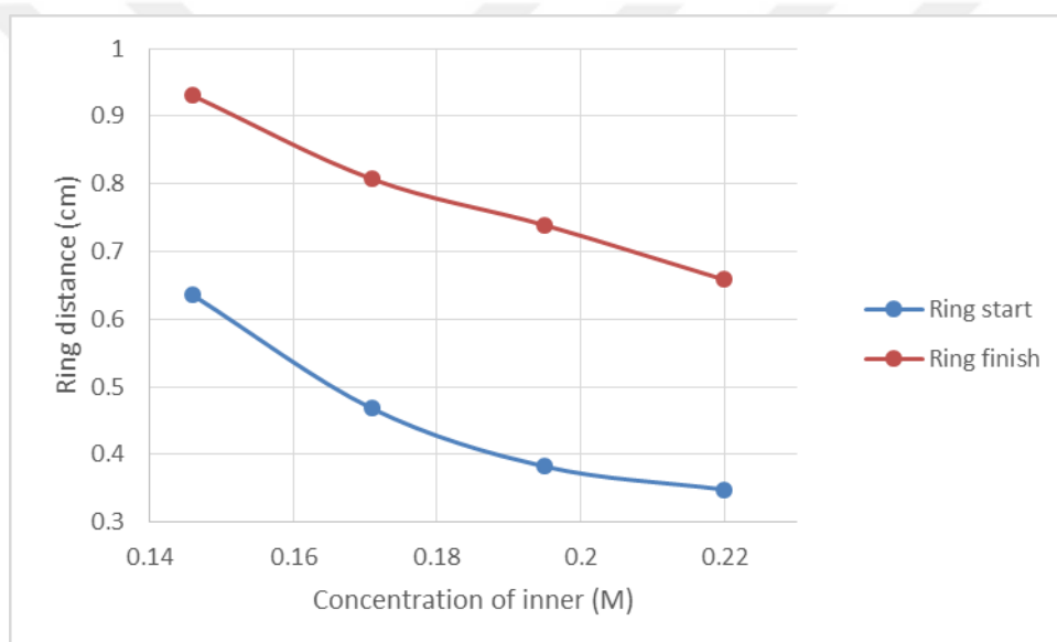
Figure 24. Calculated precipitation pattern distances as a function of inner electrolyte concentration.
