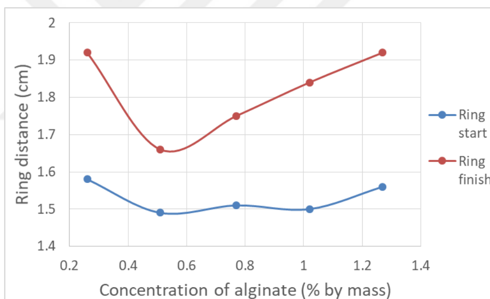
Figure 20. Calculated precipitation pattern distances as a function of alginate concentration.
