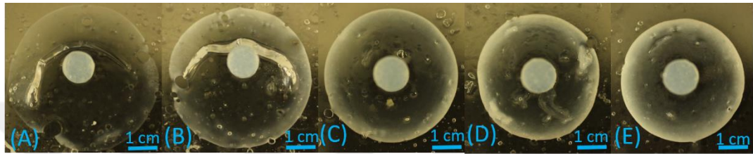
Figure 13. Change of precipitation patterns due to change of inner electrolyte concentration at constant outer electrolyte (hydroxide ion) concentration 1 M and at inner electrolyte (magnesium ion) concentrations : (A) = 0.014 M, (B) = 0.028 M, (C) = 0.042 M, (D) = 0.056 M, (E) = 0.070 M; acrylamide = 12.22 %; alginate = 1.53 %; BIS = 0.01 %; TEMED = 0.085 %; KPS = 0.25 %; (T= 20 °C).
