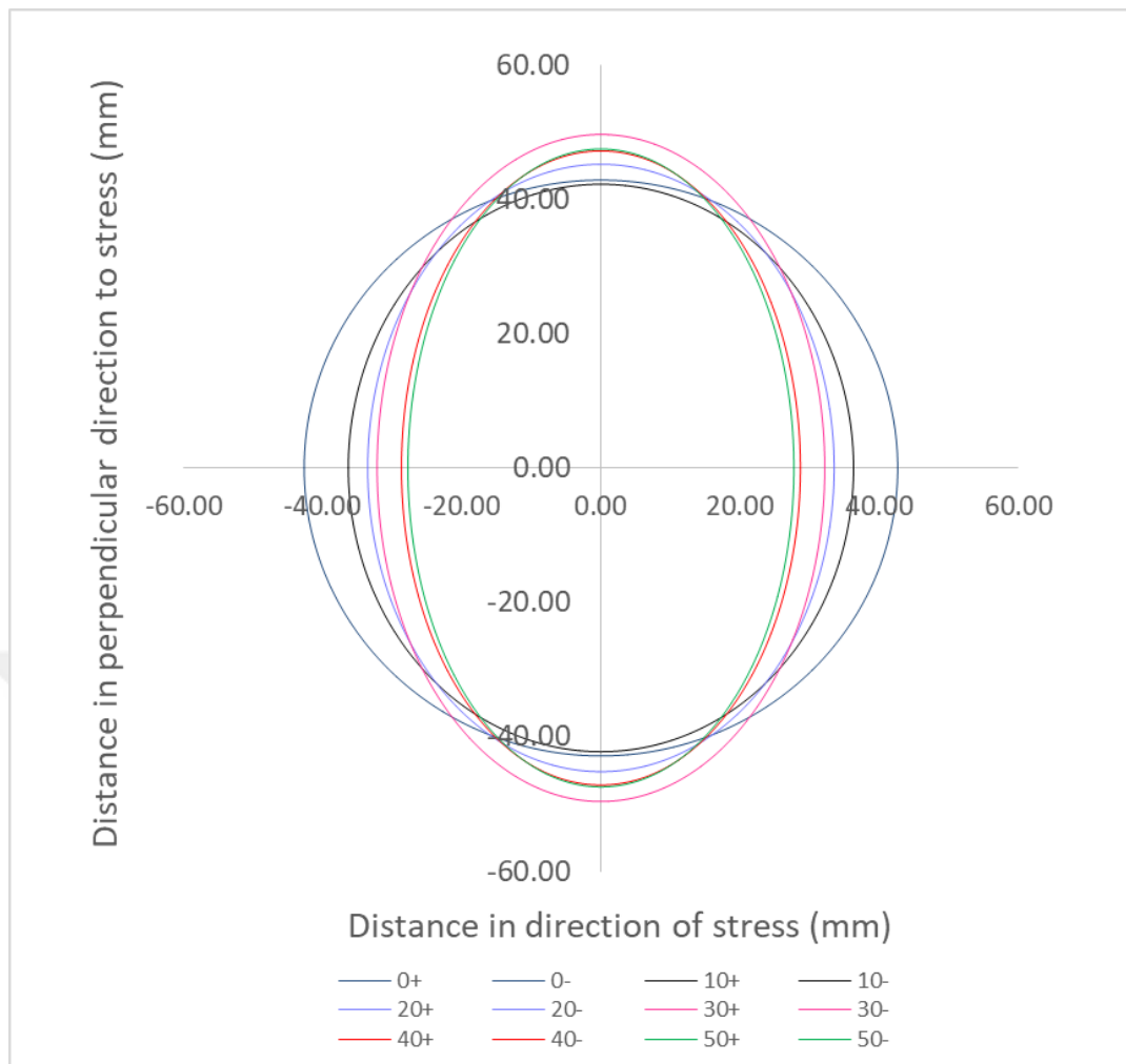
Figure 31. Cartesian coordinate of patterns immediately after release of stress.
