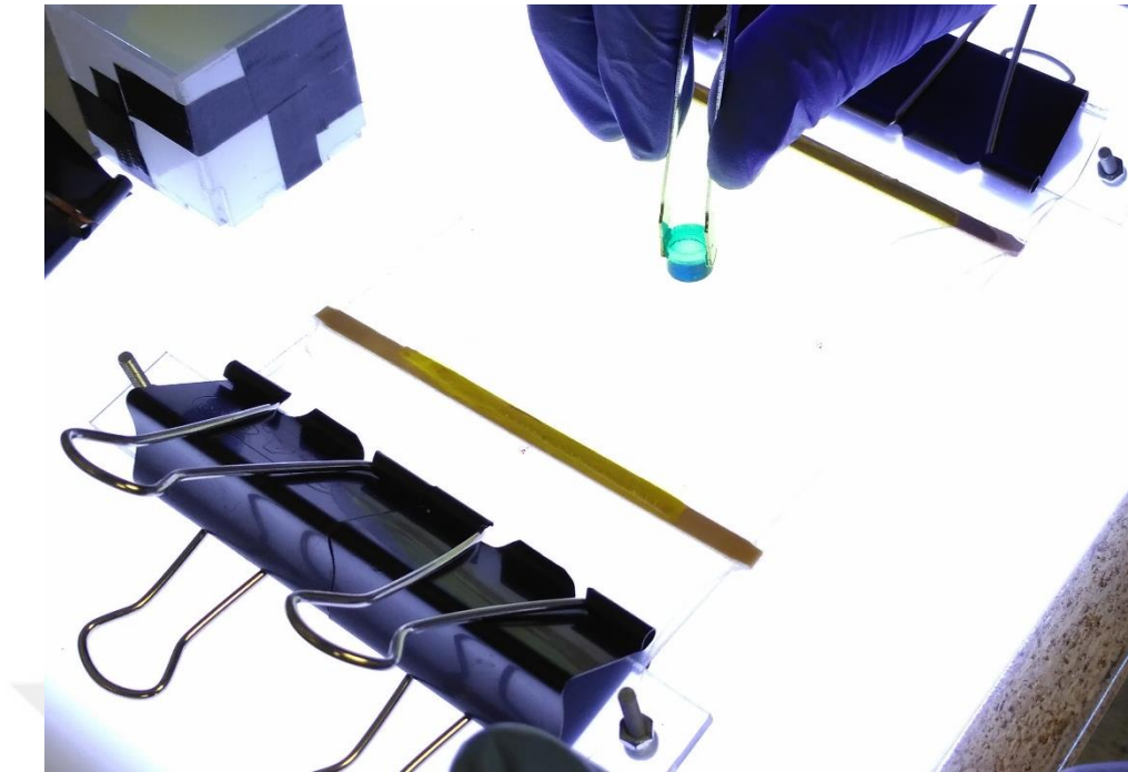
Figure 11. Placing of stamps with outer electrolyte into the center of the polyacrylamide gel.
