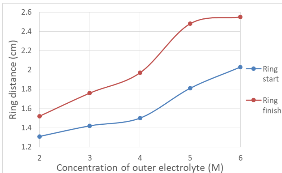
Figure 16. Calculated precipitation pattern distances as a function of outer electrolyte concentration.
