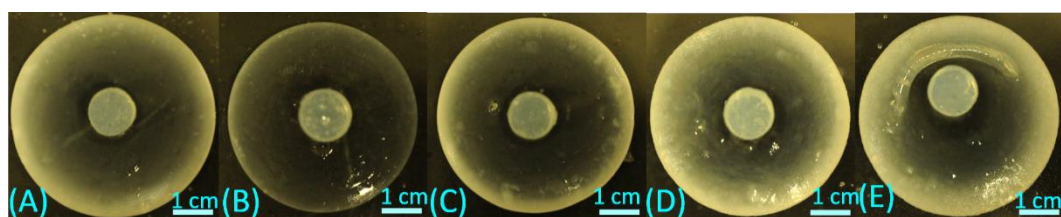
Figure 19. Change of precipitation patterns due to change of alginate concentrations at constant inner electrolyte (magnesium ion) concentration 0.07 M and at constant outer electrolyte (hydroxide ion) concentration 2 M and at alginate concentrations: (A) = 0.26 %, (B) = 0.51 %, (C) = 0.77 %, (D) = 1.02 %, (E) = 1.27 %; acrylamide = 12.25 %; BIS = 0.01 %; TEMED = 0.1 %; KPS = 0.25 %; (T= 20 °C).
