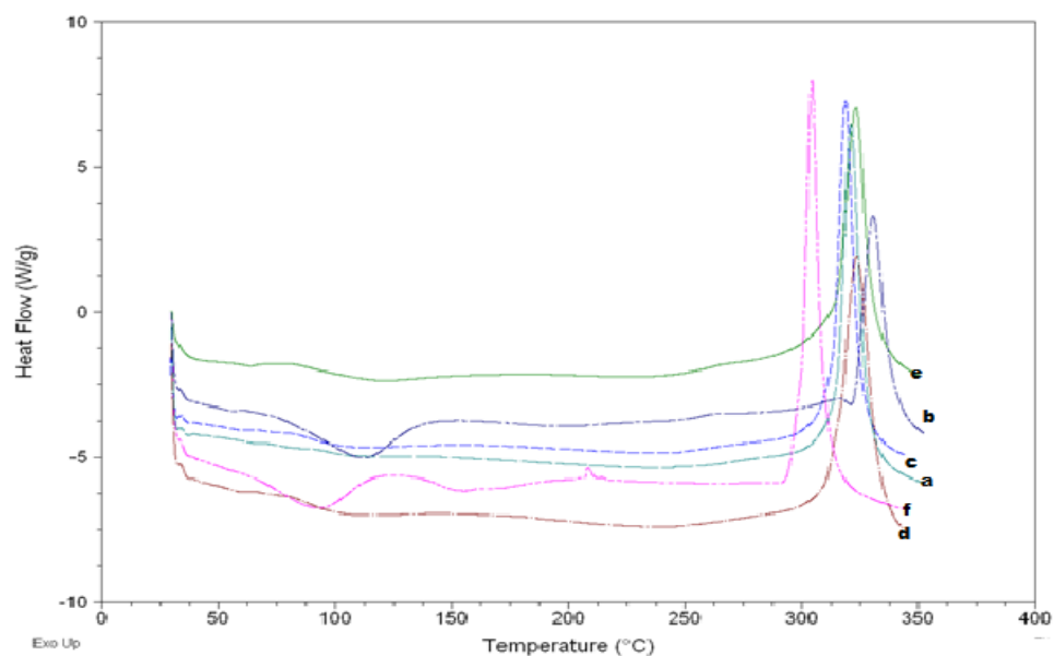
Figure 3.17 : DSC curves of electrospun nanofibers a-PAN/DMSO nanofiber, b)PAN/PANI(%3)/DMSO nanofiber, c-(%1) CNT-NH 2 /PAN/ DMSO nanofiber, d- (%3) CNT-NH 2 /PAN/ DMSO nanofiber, e- (%1) CNT-NH 2 /PAN/PANI/DMSO nanofiber, f-(%3) CNT-NH 2 /PAN/PANI/DMSO nanofiber.
