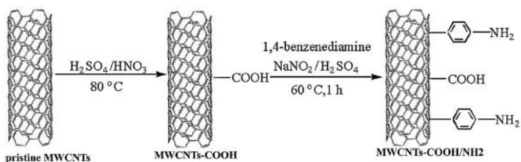
Figure 2.3 : Functionalization of CNTs with carboxyl or amine groups.
