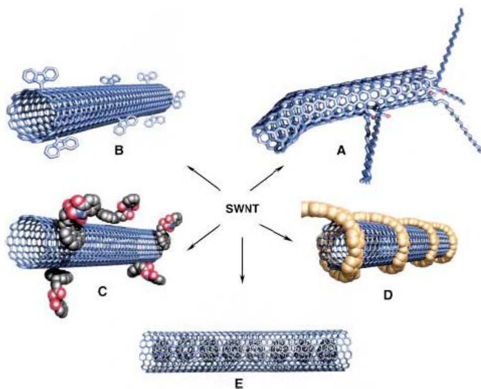
Figure 2.4 : Functionalization possibilities a) defect group functionalization b) covalent sidewall functionalization c) non-covalent exohedral functionalization with surfactants d) non-covalent exohedral functionalization with polymers e) endohedral functionalization [22].
