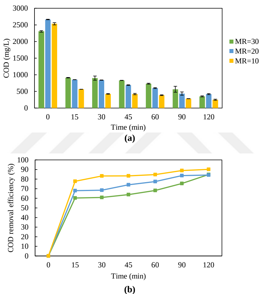
Figure 4.1. Change in COD of WAS during Fenton Oxidation (a); COD removal efficiency in time (b)
