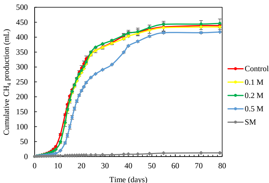
Figure 4.10. Average cumulative \text{CH}_4 production results for preliminary BMP test
