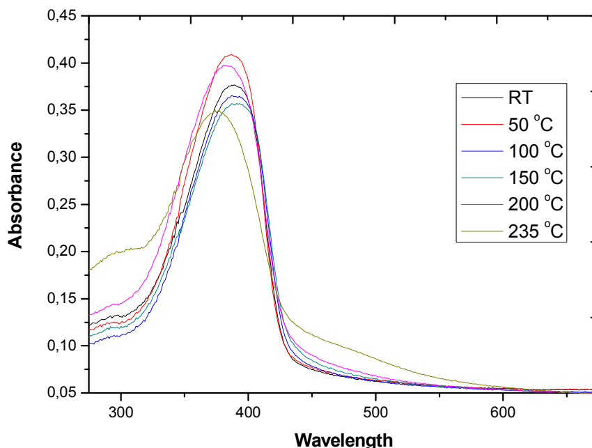
Fig. 2.47- In-situ UV-VIS measurement of P2 under heat exposure
