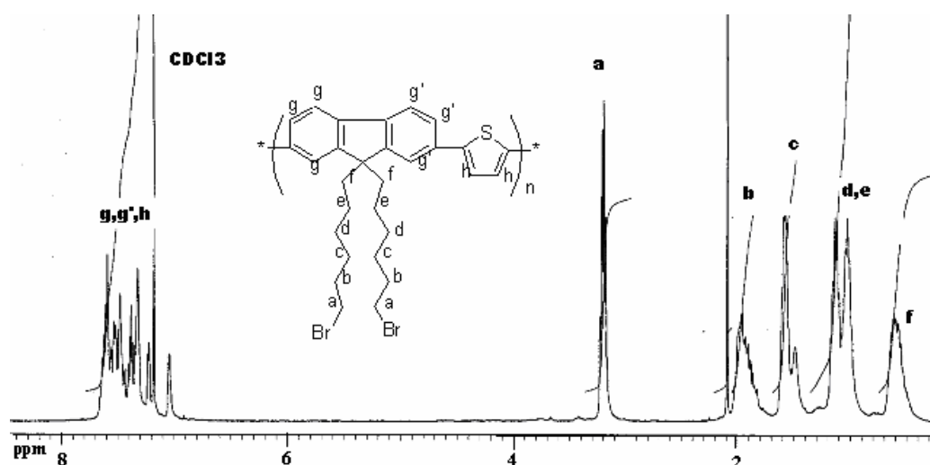
Fig. 2.32- ^1\text{H} -NMR spectrum of P5 (400 MHz, \text{CDCl}_3 , 25 °C)
