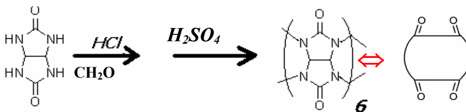
Figure 1.16- Synthesis of cucurbit[6]uril
