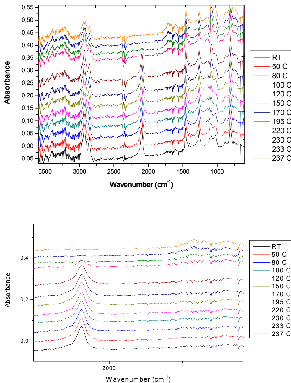
Fig. 2.45- (a) In-situ FT-IR measurement of P2 under heat exposure, (b) Inset between 2300 \text{cm}^{-1} and 1500 \text{cm}^{-1}
