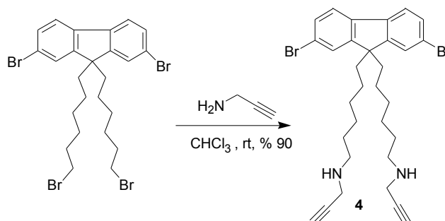
Scheme 2.17- The Synthesis of 4
