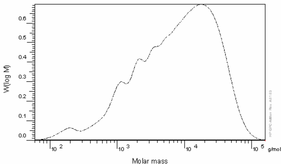
Fig. 2.29- GPC analysis of P4 (Polystyrene as standard)
