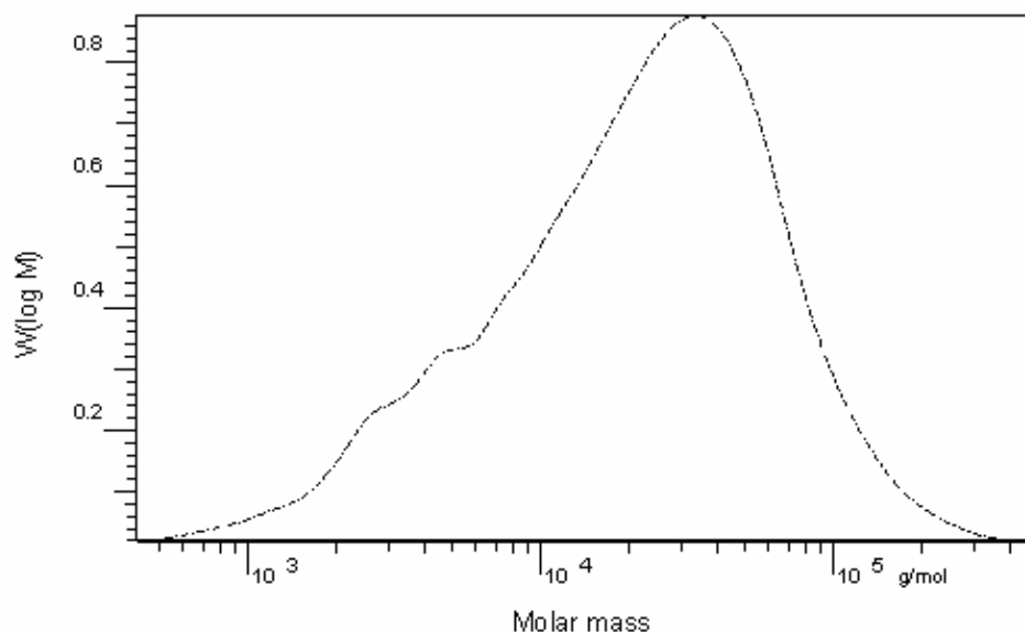
Fig. 2.14- GPC analysis of P1 (Polystyrene as standard)
