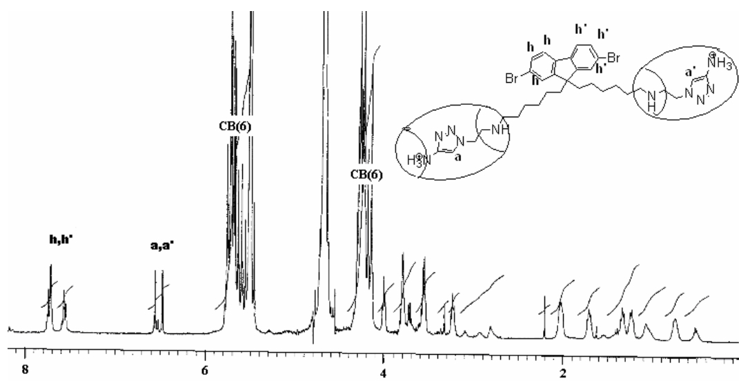
Fig. 2.40- ^1\text{H} -NMR spectrum of Rotaxane. (400 MHz, \text{D}_2\text{O} , 25 °C)
