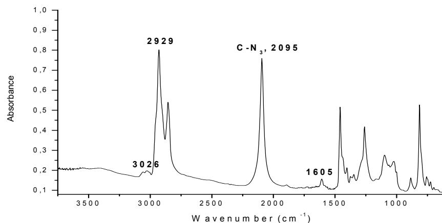
Fig. 2.18- FT-IR spectrum of P2
