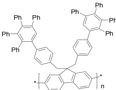
Fig. 1.14- Polyfluorene with Mullen type dendrons 31
