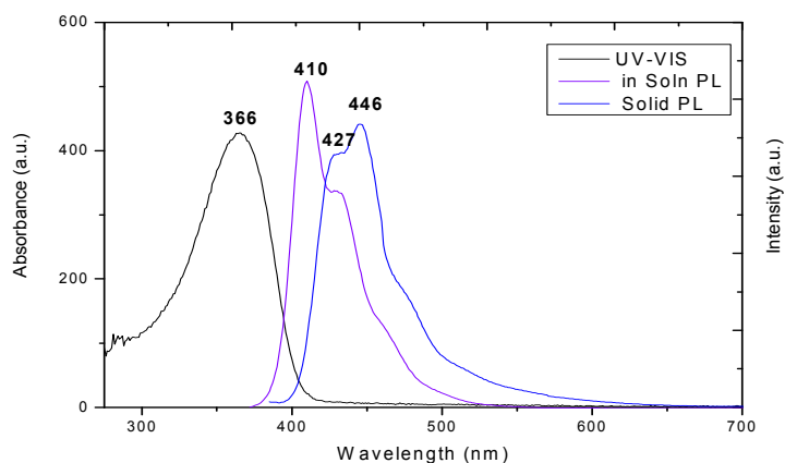
Fig. 2.28- UV-VIS and PL emission spectra of P4 in CHCl 3
