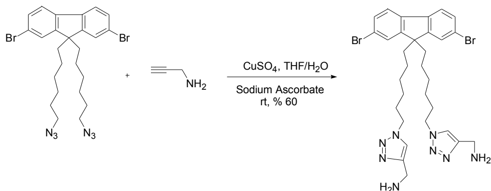
Scheme 2.16- Click chemistry reaction between 3 and propargylamine
