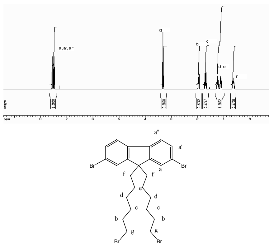
Fig. 2.1- 1 H-NMR Spectrum of 1 (400 MHz, CDCl 3 , 25 °C)
