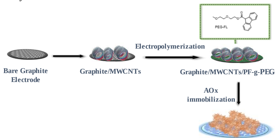
Figure 2.3. Representation of MWCNTs/ PF-g- PEG/AOx biosensor
