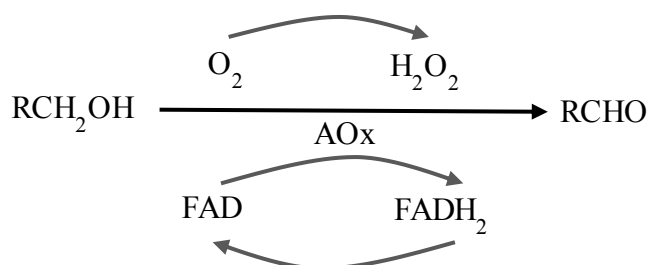
Figure 1.8. Representation of the reaction mechanism of alcohol oxidase
