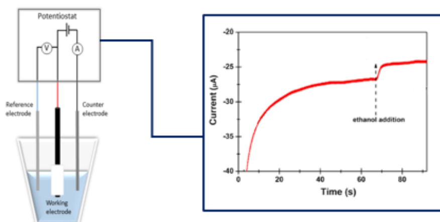
Figure 2.4. Representation of amperometric measurement
