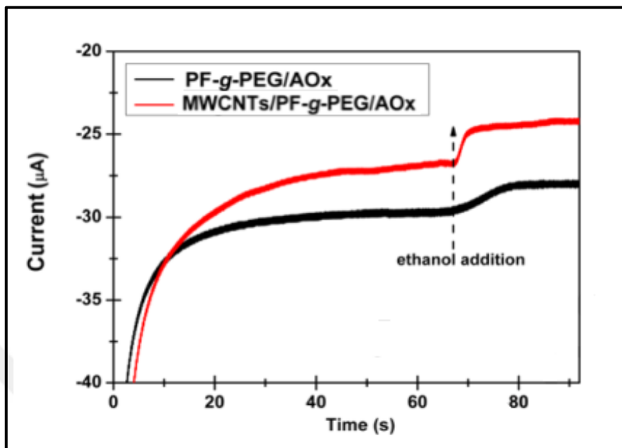
Figure 2.8. Comparison of the amperometric responses of the alcohol sensors for 4.25 mM ethanol
