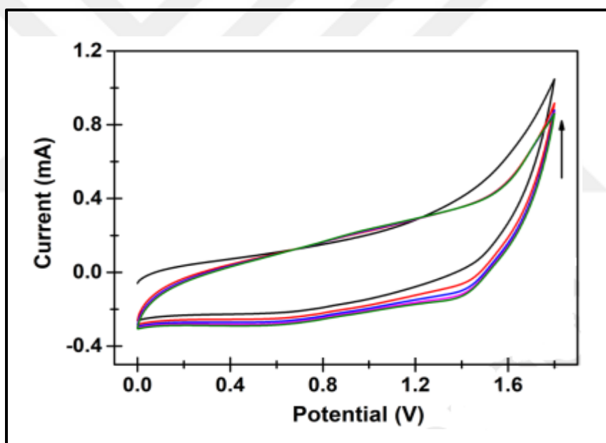
Figure 2.2. Cyclic voltammogram of PEG-FL on graphite electrode (up to 5 cycles)
