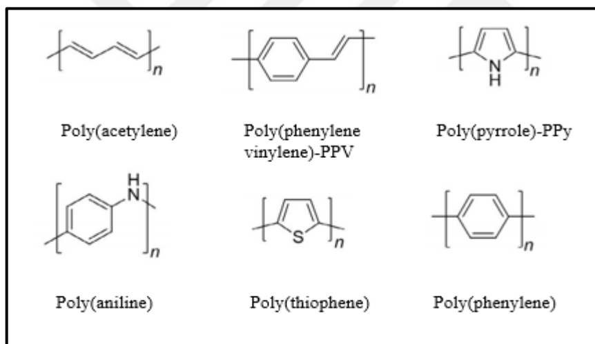
Figure 1.9. Some common conjugated polymers
